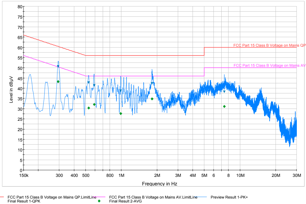
Plot 6-64. Line Conducted Plot with 802.11b (N)
