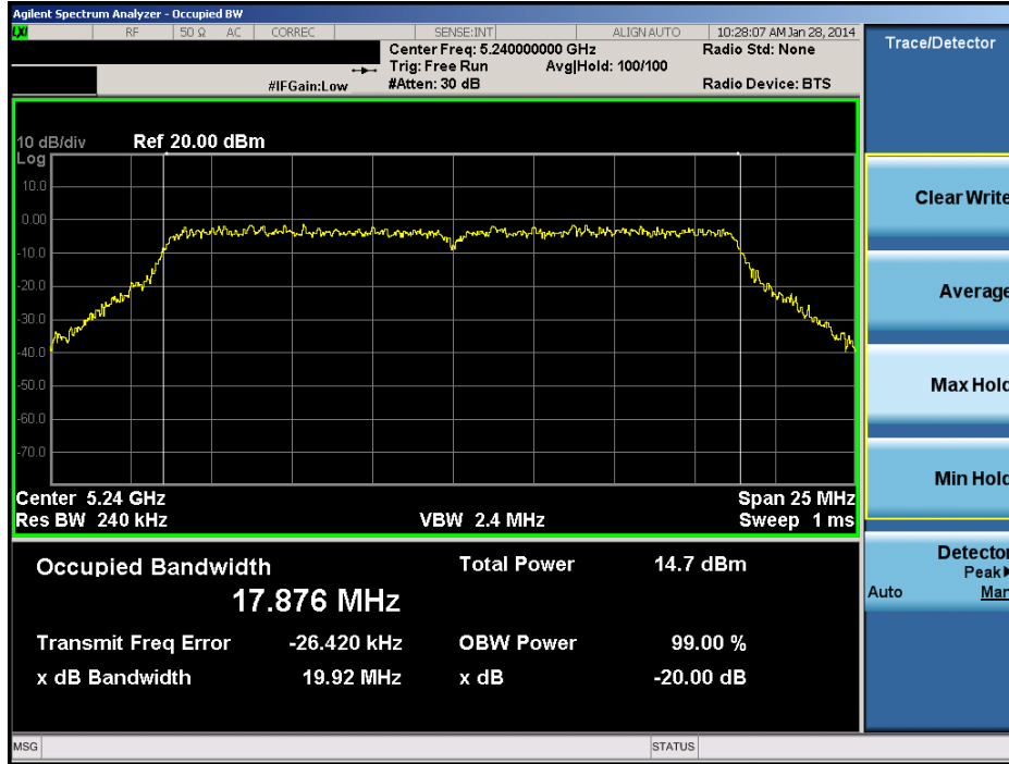
Plot 6-27. 20dB Bandwidth Plot (20MHz 802.11n (UNII Band 1) – Ch. 48)
