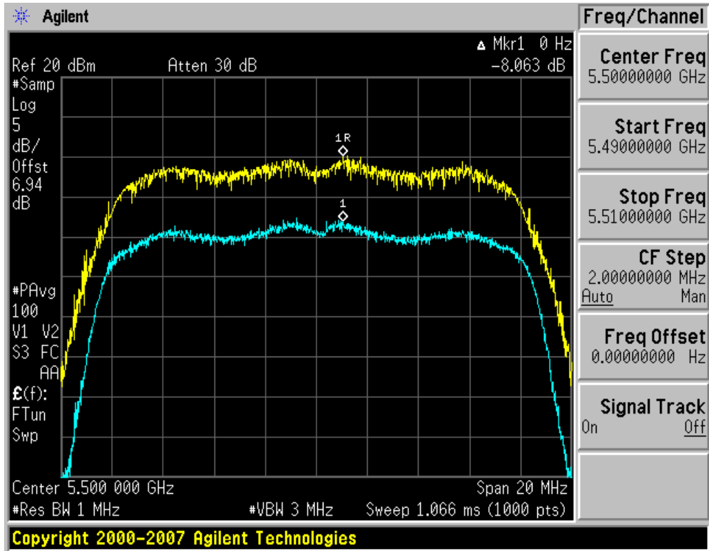
Plot 6-49. Peak Excursion Ratio Plot (802.11a (UNII Band 3) – Ch. 100)
