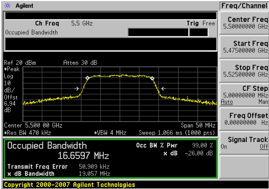
Plot 6-13. 26dB Bandwidth Plot (802.11a (UNII Band 3) – Ch. 100)
