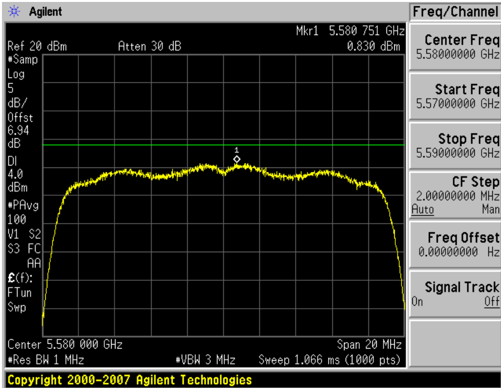
Plot 6-35. Peak Power Spectral Density Plot (802.11n (UNII Band 3) – Ch. 116)
