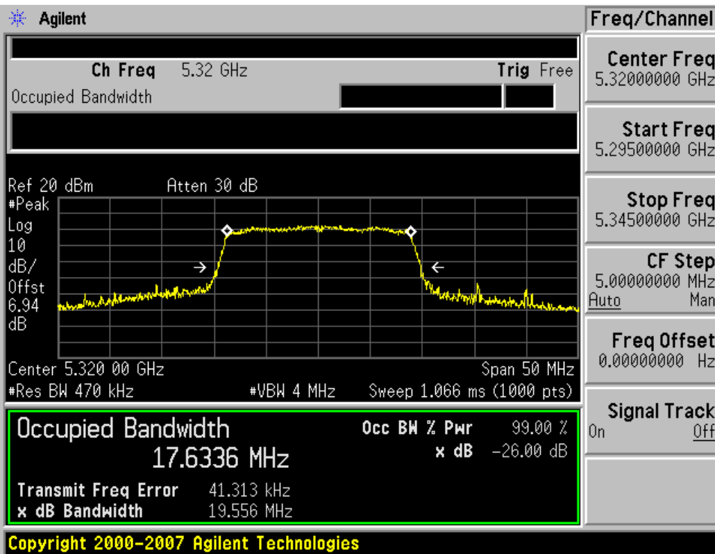
Plot 6-12. 26dB Bandwidth Plot (802.11n (UNII Band 2) – Ch. 64)
