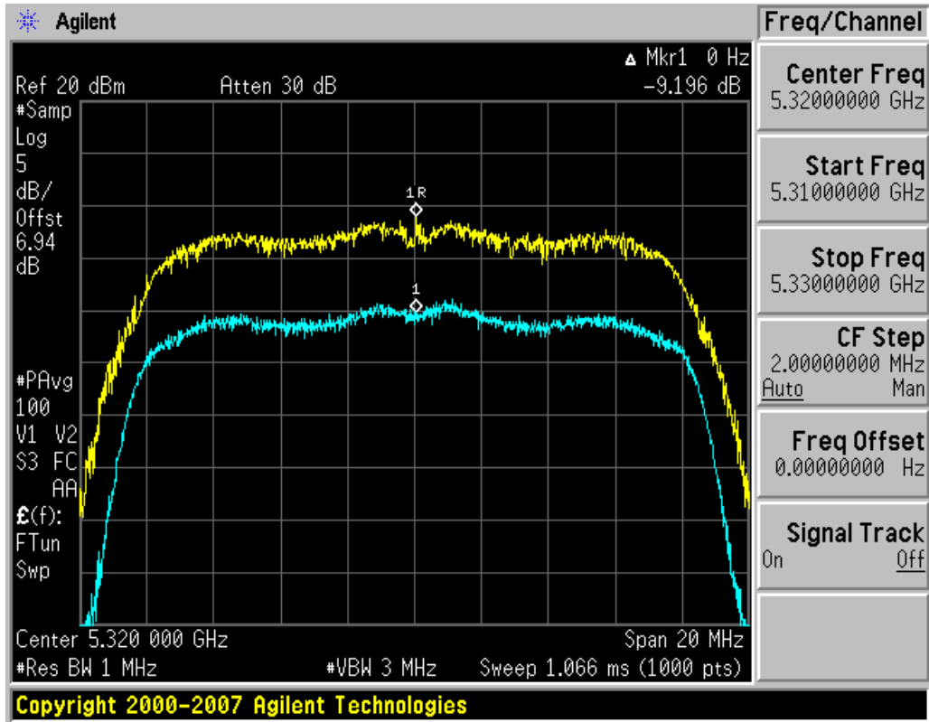
Plot 6-45. Peak Excursion Ratio Plot (802.11a (UNII Band 2) – Ch. 64)
