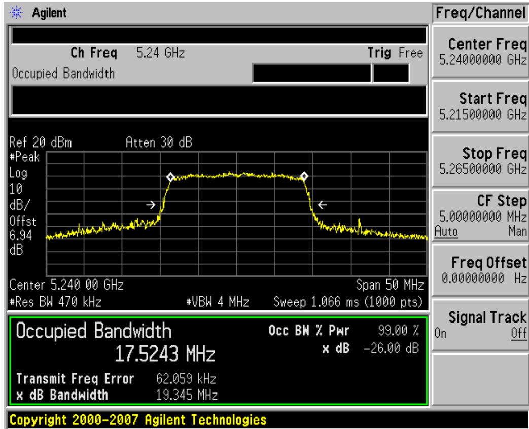
Plot 6-6. 26dB Bandwidth Plot (802.11n (UNII Band 1) – Ch. 48)
