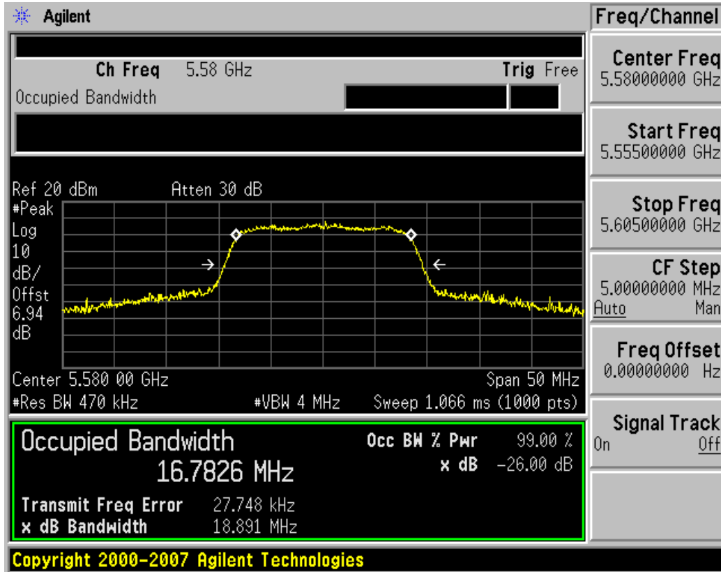
Plot 6-14. 26dB Bandwidth Plot (802.11a (UNII Band 3) – Ch. 116)
