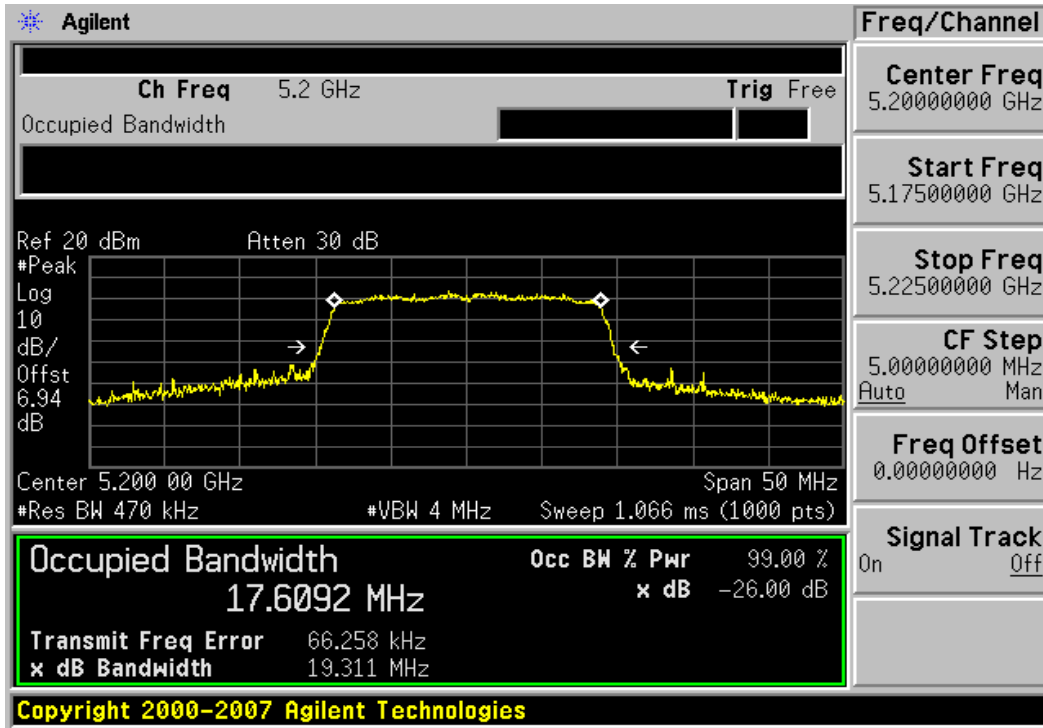
Plot 6-5. 26dB Bandwidth Plot (802.11n (UNII Band 1) – Ch. 40)
