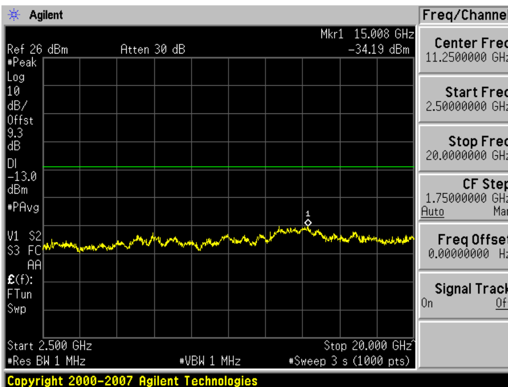
Plot 7-6. Conducted Spurious Plot (AWS WCDMA Mode – Ch. 1412)
