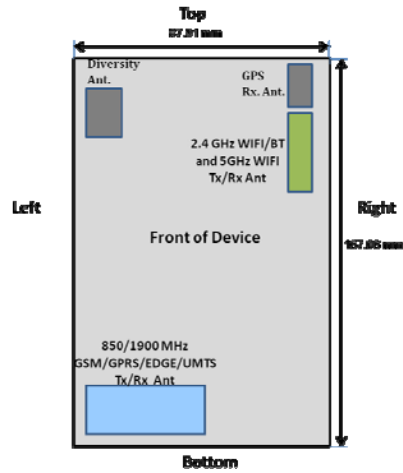
Figure 1-1 DUT Antenna Locations
