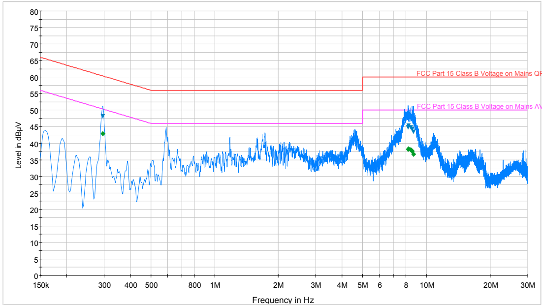
Plot 6-20. Line Conducted Plot with Bluetooth LE (N)
