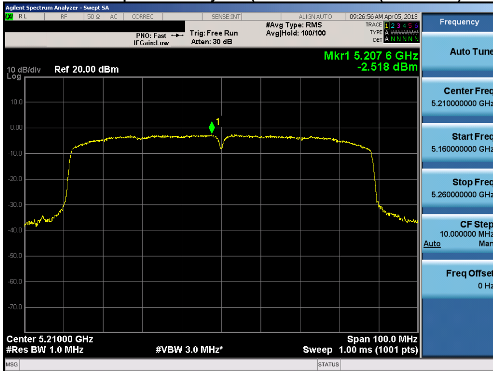
Plot 6-58. Peak Power Spectral Density Plot (80MHz BW 802.11ac (UNII Band 1) – Ch. 42)
