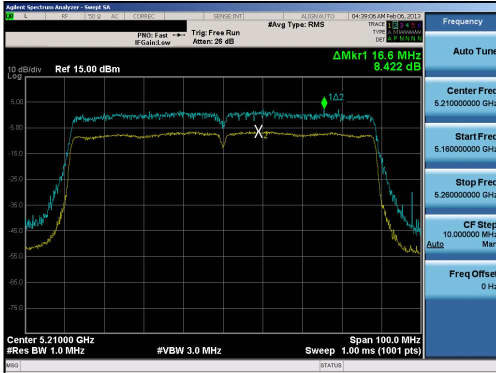
Plot 6-64. Peak Excursion Ratio Plot (80MHz BW 802.11n)
