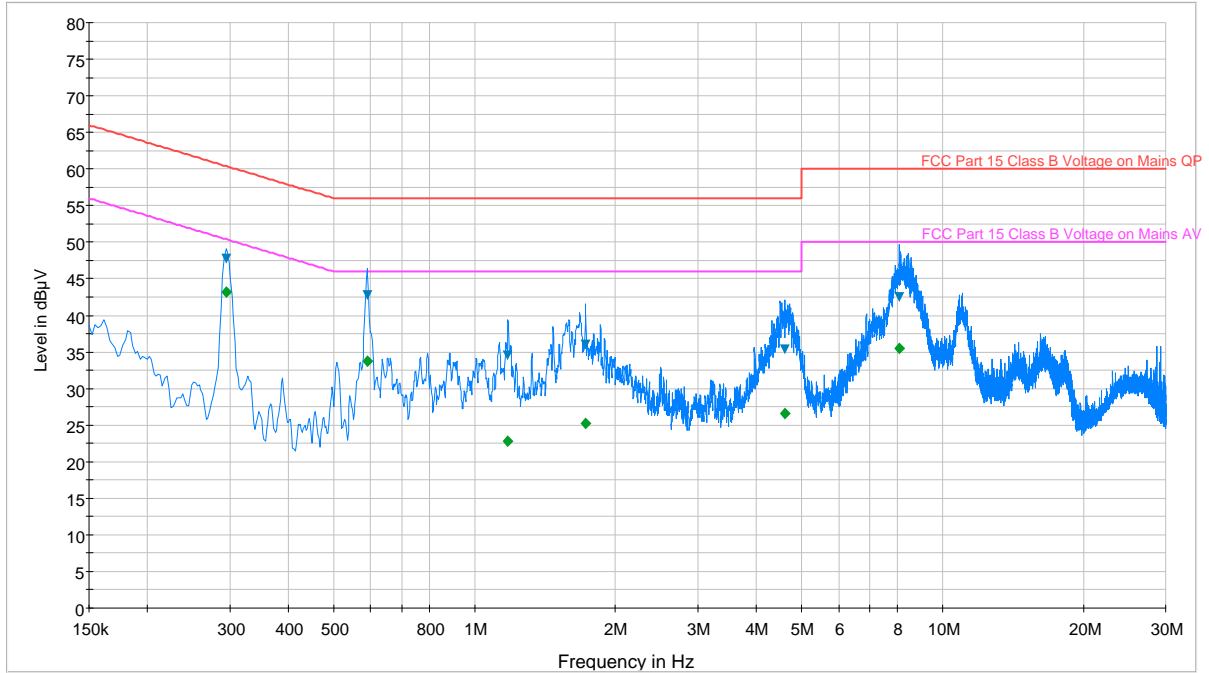
Plot 6-85. Line Conducted Plot with 802.11a UNII Band 1 (L1)
