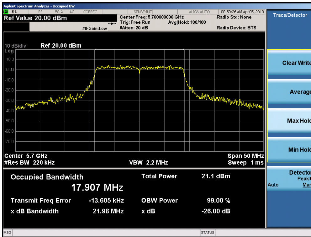
Plot 6-22. 26dB Bandwidth Plot (20MHz BW 802.11n (UNII Band 3) – Ch. 140)
