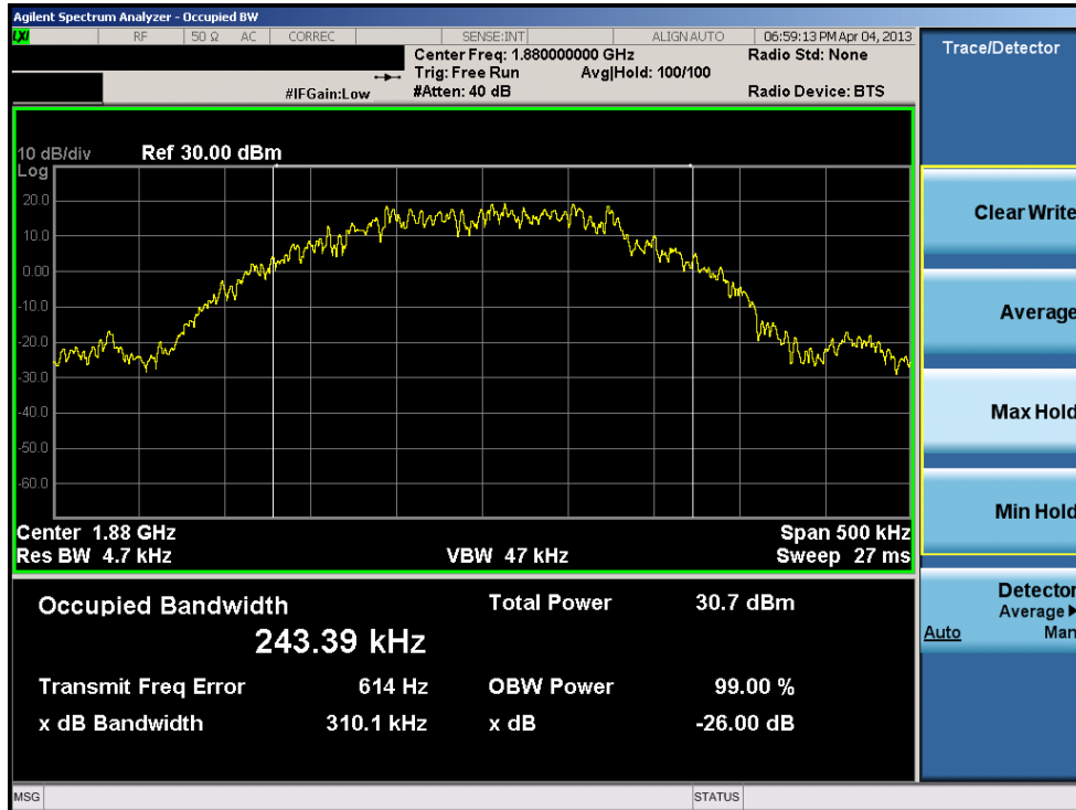
Plot 7-24. Occupied Bandwidth Plot (EDGE1900 Mode – Ch. 661)
