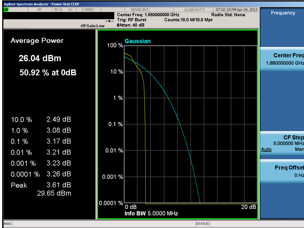
Plot 7-25. Peak-Average Ratio Plot (EDGE1900 Mode – Ch. 661)
