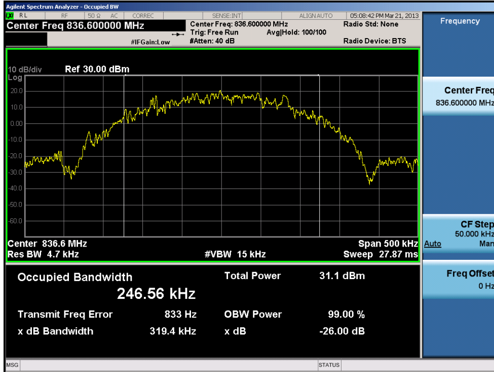
Plot 7-13. Occupied Bandwidth Plot (EDGE850 Mode – Ch. 190)
