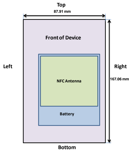
Figure 1-2 NFC Antenna Locations
