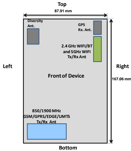
Figure 1-1 DUT Antenna Locations
