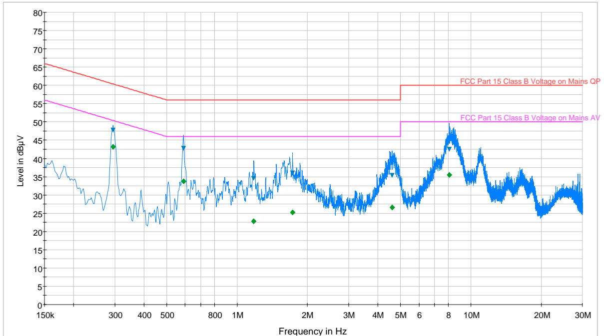
Plot 6-81. Line Conducted Plot with 802.11a UNII Band 1 (L1)
