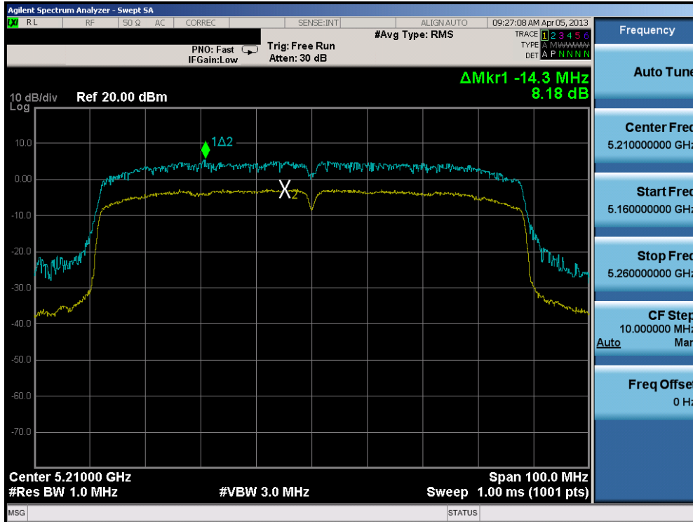
Plot 6-60. Peak Excursion Ratio Plot (80MHz BW 802.11n)
