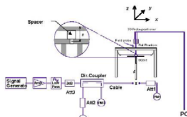
Figure 9-1 System Verification Setup Diagram
