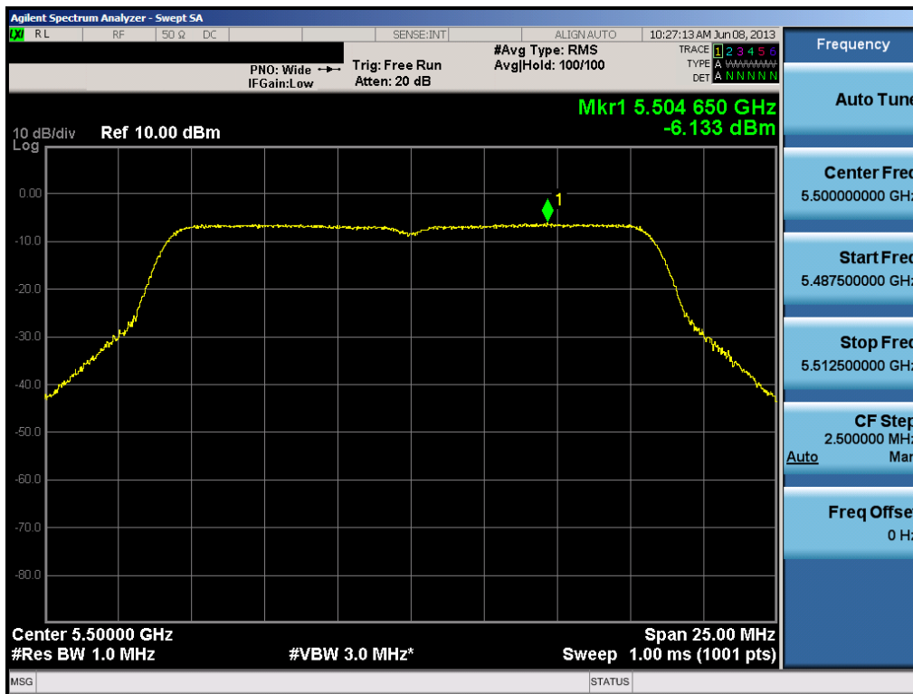
Plot 6-43. Peak Power Spectral Density Plot (802.11a (UNII Band 3) – Ch. 100)
