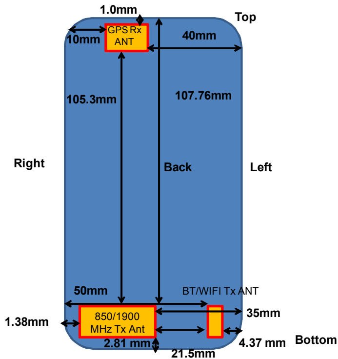
Figure 13-1 Identification of Sides for SAR Testing
