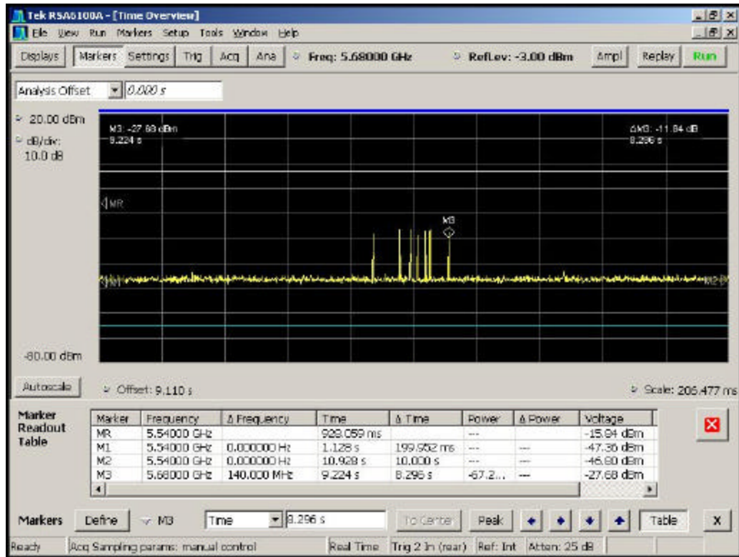
Figure 6-10. Pulse Grouping 5
