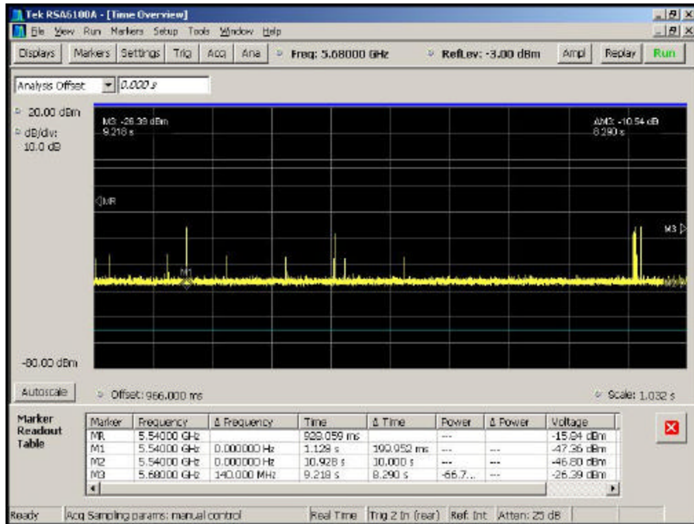
Figure 6-6. Pulse Grouping 1
