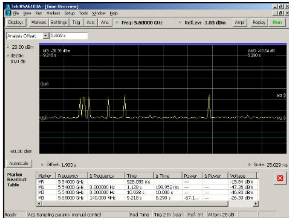
Figure 6-7. Pulse Grouping 2
