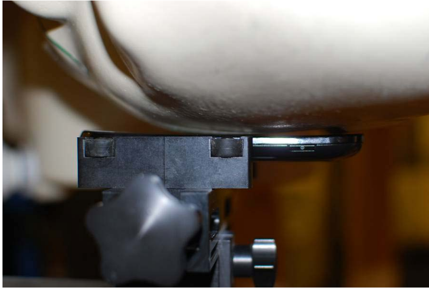
Figure 21-3 SAR Test Setup Photo – Left Touch
