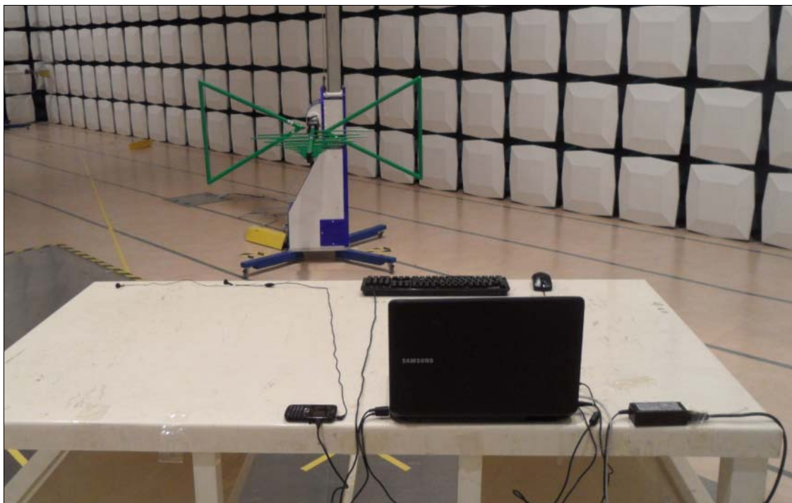
[ Radiated Disturbance for Below 1 GHz – Rear ]
