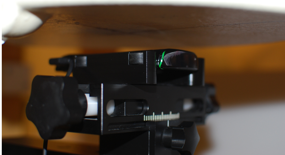
Figure 19-5 SAR Test Setup Photo 5
