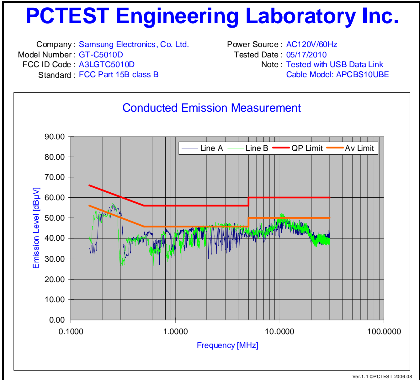
Plot 7-1. Line-Conducted Test Plot
