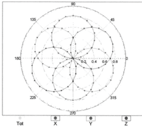
f=600 MHz,TEM
