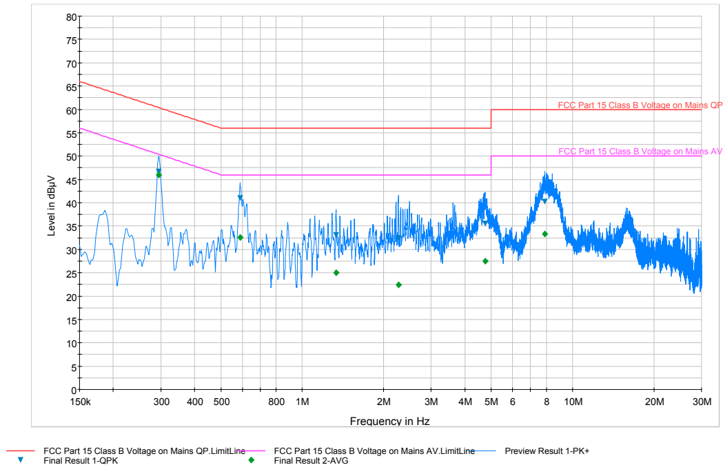
Plot 6-63. Line Conducted Plot with 802.11b (L1)
