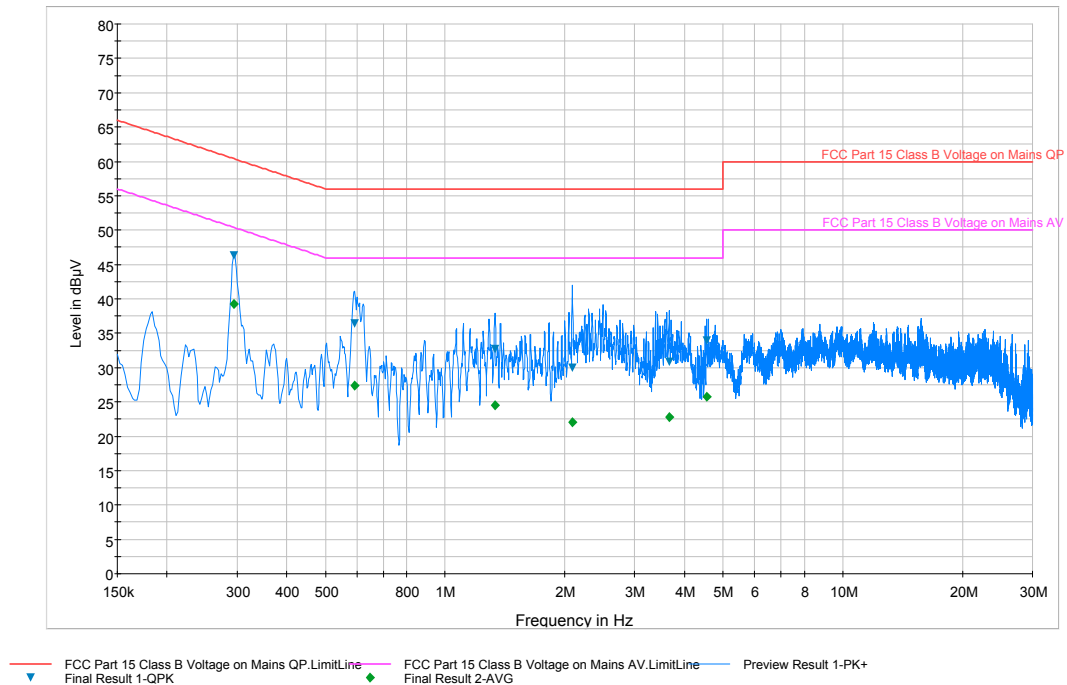
Plot 6-65. Line Conducted Plot with 802.11a (L1)
