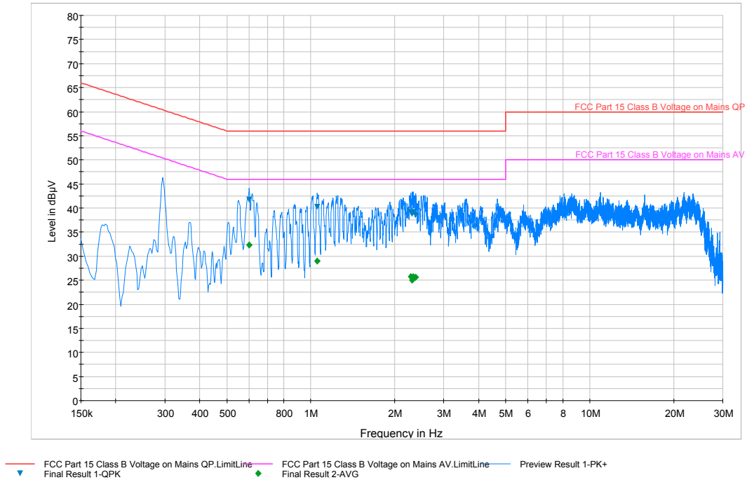
Plot 6-66. Line Conducted Plot with 802.11a (N)
