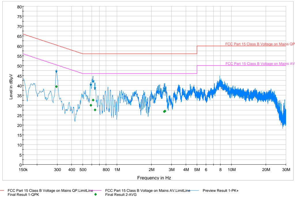
Plot 6-71. Line Conducted Plot with 802.11a UNII Band 2 (N)
