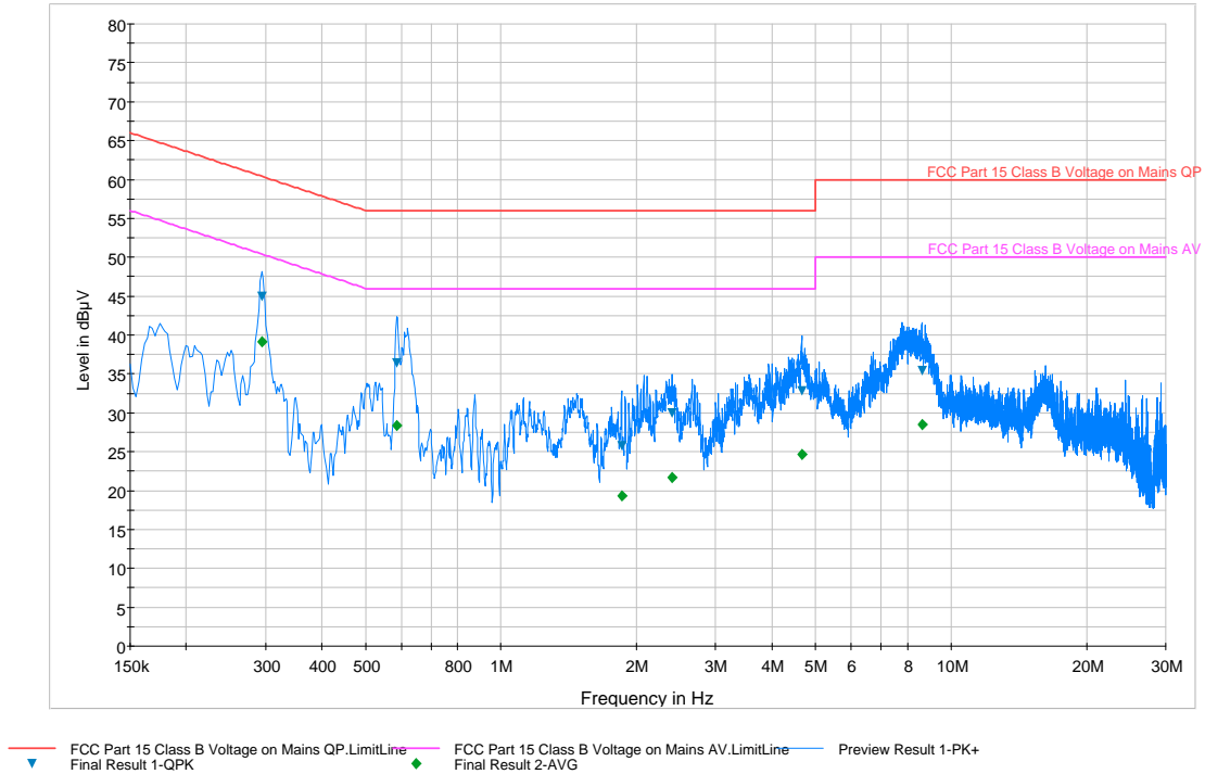
Plot 6-68. Line Conducted Plot with 802.11a UNII Band 1 (L1)
