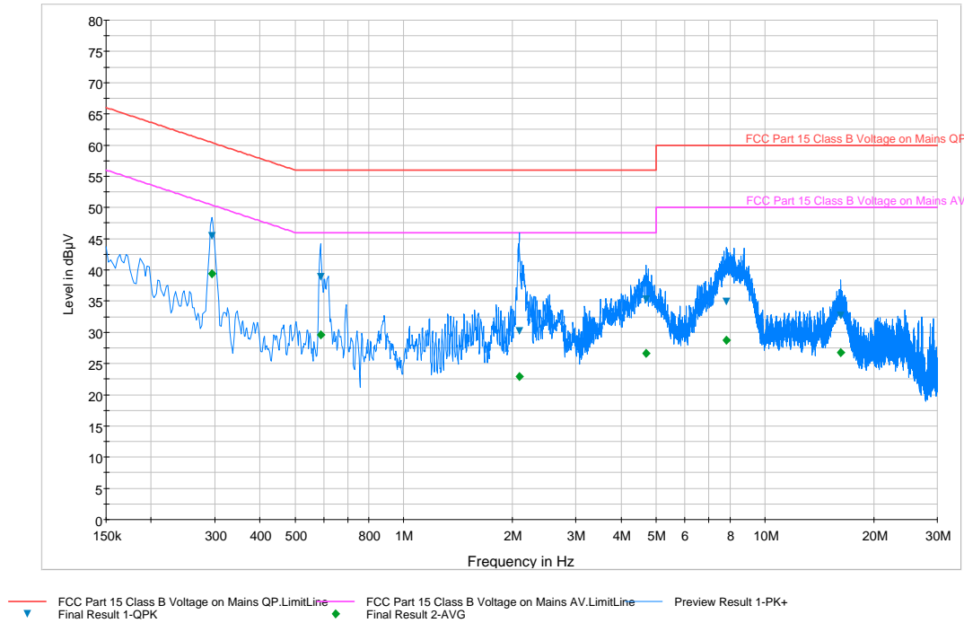
Plot 6-72. Line Conducted Plot with 802.11a UNII Band 3 (L1)
