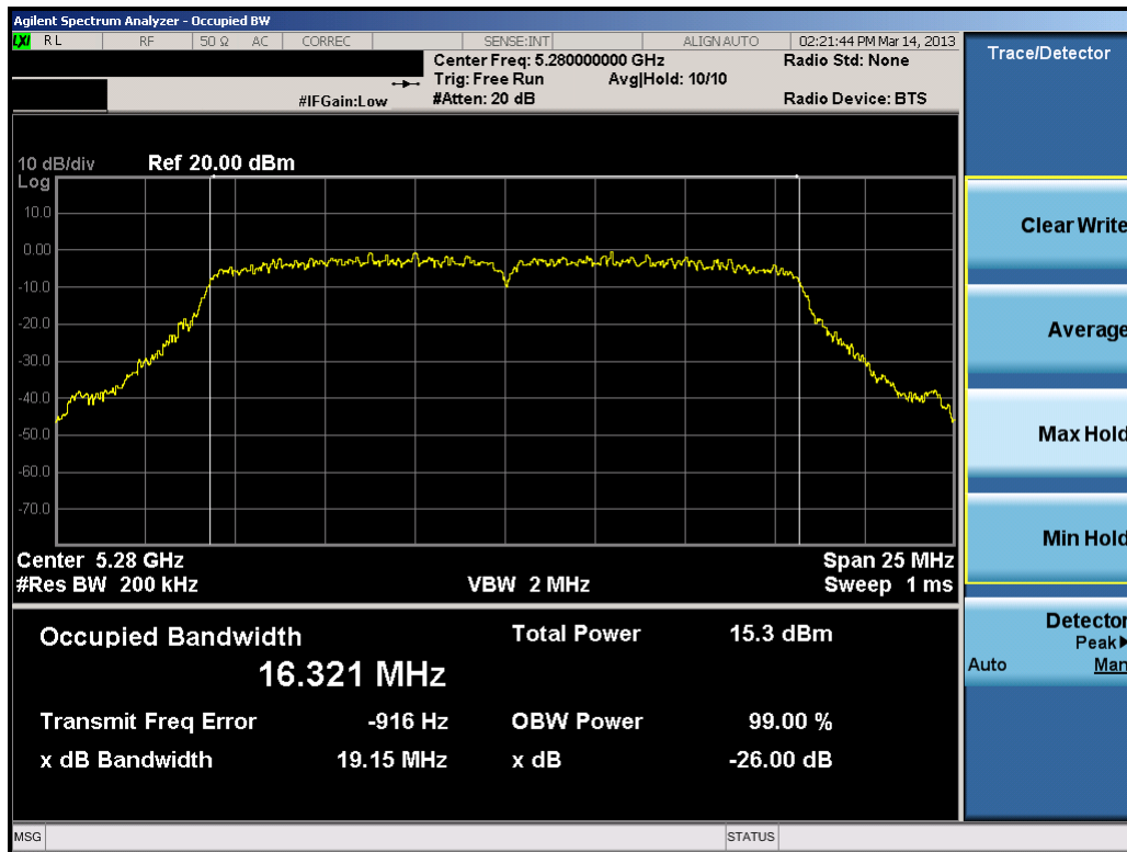
Plot 6-35. 26dB Bandwidth Plot (802.11a (UNII Band 2) – Ch. 56)
