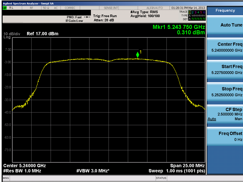
Plot 6-53. Peak Power Spectral Density Plot (802.11a (UNII Band 1) – Ch. 48)
