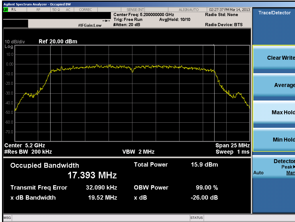
Plot 6-30. 26dB Bandwidth Plot (20MHz BW 802.11n (UNII Band 1) – Ch. 40)
