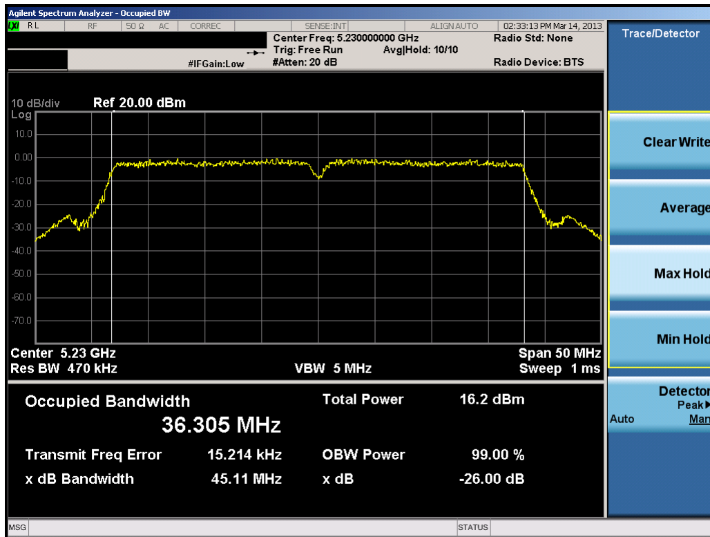
Plot 6-33. 26dB Bandwidth Plot (40MHz BW 802.11n (UNII Band 1) – Ch. 46)
