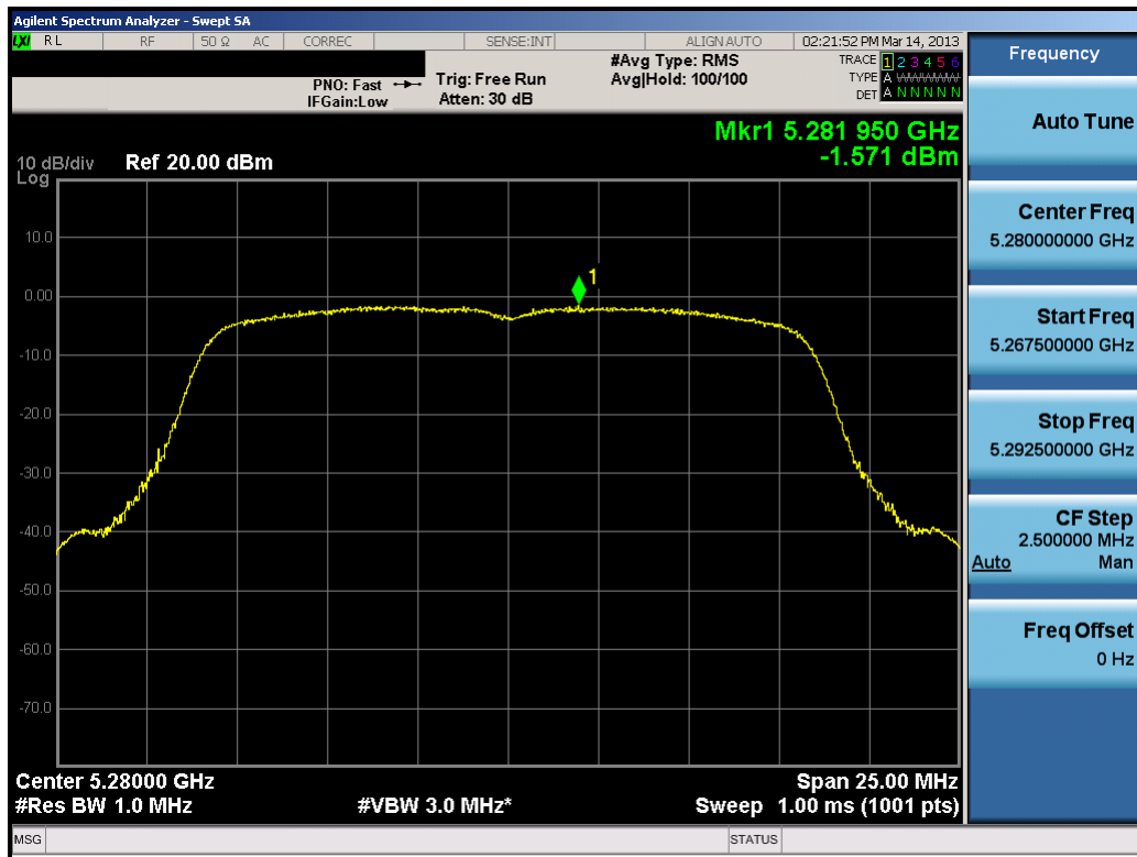
Plot 6-85. Peak Power Spectral Density Plot (802.11a (UNII Band 2) – Ch. 56)
