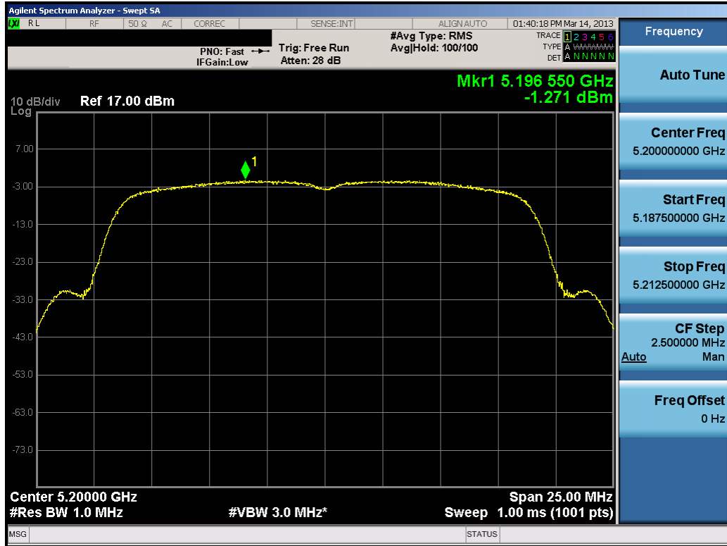
Plot 6-55. Peak Power Spectral Density Plot (20MHz BW 802.11n (UNII Band 1) – Ch. 40)
