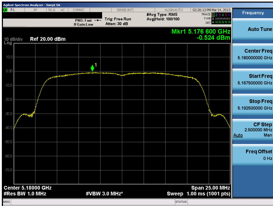
Plot 6-79. Peak Power Spectral Density Plot (20MHz BW 802.11n (UNII Band 1) – Ch. 36)
