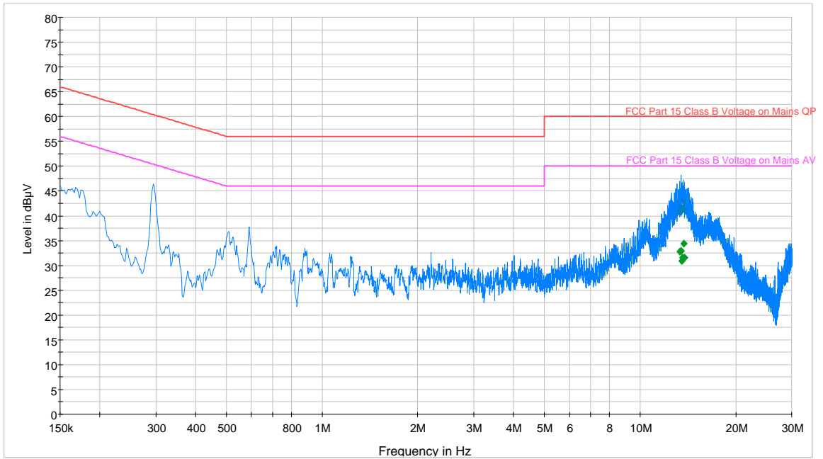
Plot 6-162. Line Conducted Plot with 802.11n UNII Band 1 (N)
