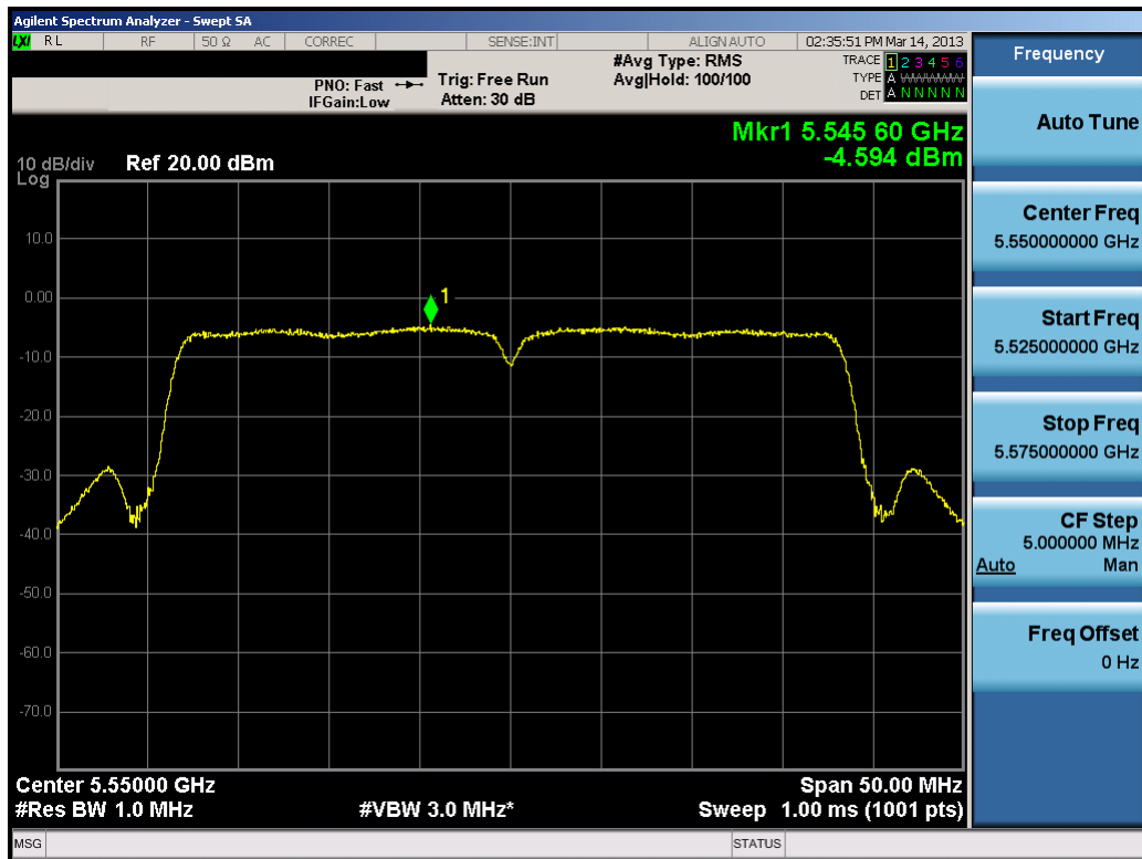
Plot 6-99. Peak Power Spectral Density Plot (40MHz BW 802.11n (UNII Band 3) – Ch. 110)
