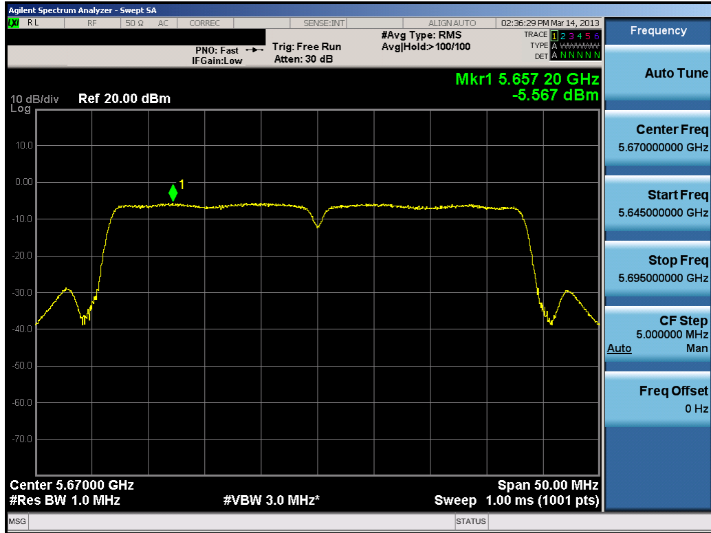
Plot 6-100. Peak Power Spectral Density Plot (40MHz BW 802.11n (UNII Band 3) – Ch. 134)
