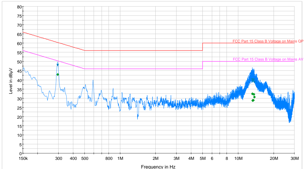
Plot 6-156. Line Conducted Plot with 802.11a UNII Band 1 (N)
