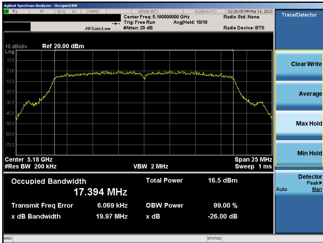
Plot 6-29. 26dB Bandwidth Plot (20MHz BW 802.11n (UNII Band 1) – Ch. 36)
