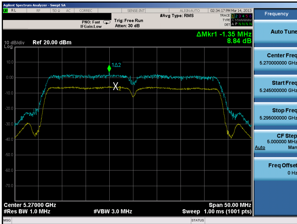
Plot 6-106. Peak Excursion Ratio Plot (40MHz BW 802.11n)
