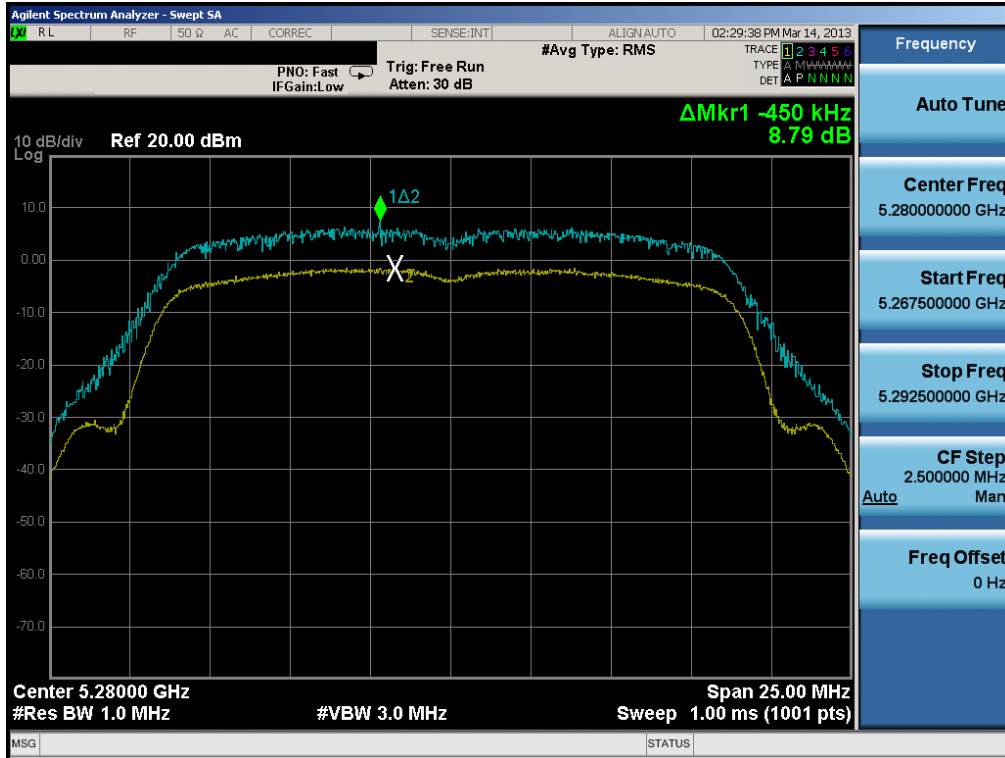
Plot 6-105. Peak Excursion Ratio Plot (20MHz BW 802.11n)
