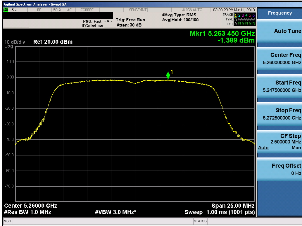
Plot 6-84. Peak Power Spectral Density Plot (802.11a (UNII Band 2) – Ch. 52)
