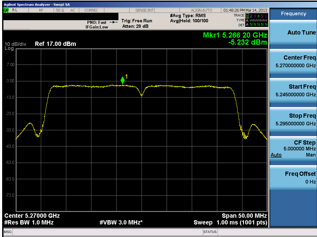
Plot 6-65. Peak Power Spectral Density Plot (40MHz BW 802.11n (UNII Band 2) – Ch. 54)
