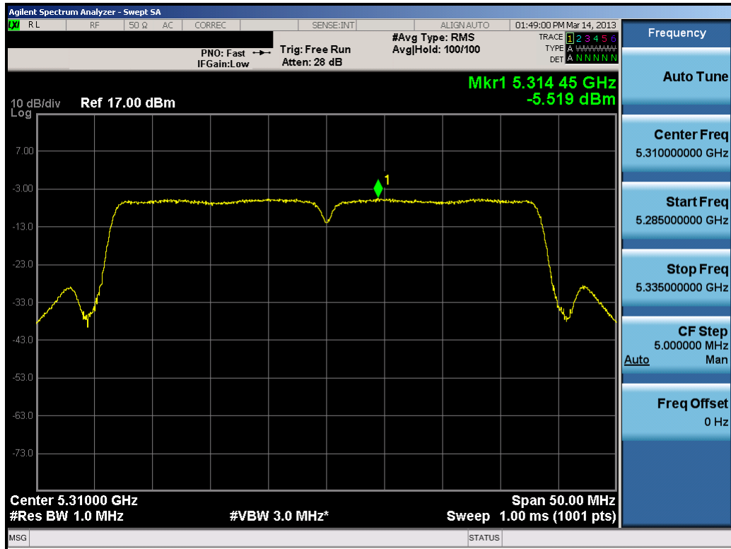
Plot 6-66. Peak Power Spectral Density Plot (40MHz BW 802.11n (UNII Band 2) – Ch. 62)
