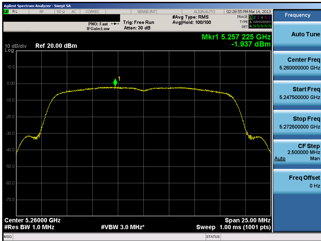
Plot 6-87. Peak Power Spectral Density Plot (20MHz BW 802.11n (UNII Band 2) – Ch. 52)
