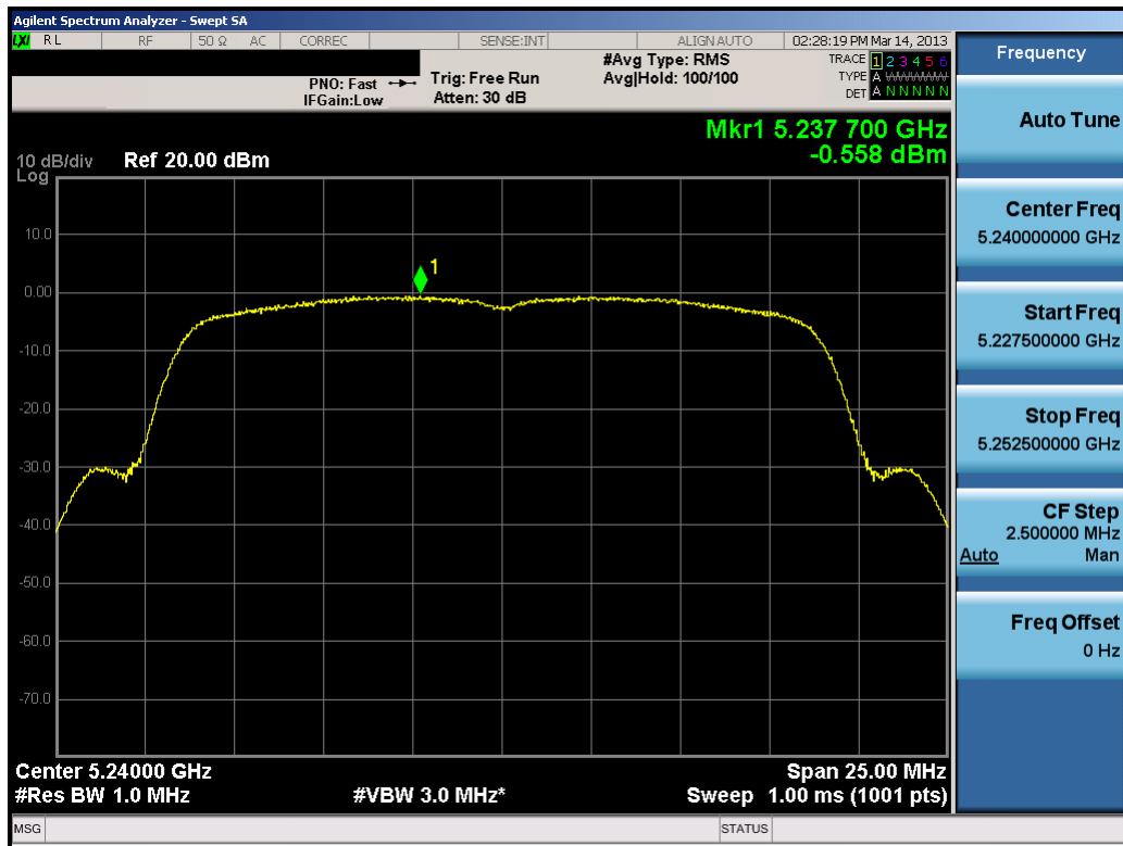
Plot 6-81. Peak Power Spectral Density Plot (20MHz BW 802.11n (UNII Band 1) – Ch. 48)
