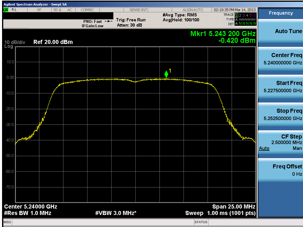
Plot 6-78. Peak Power Spectral Density Plot (802.11a (UNII Band 1) – Ch. 48)
