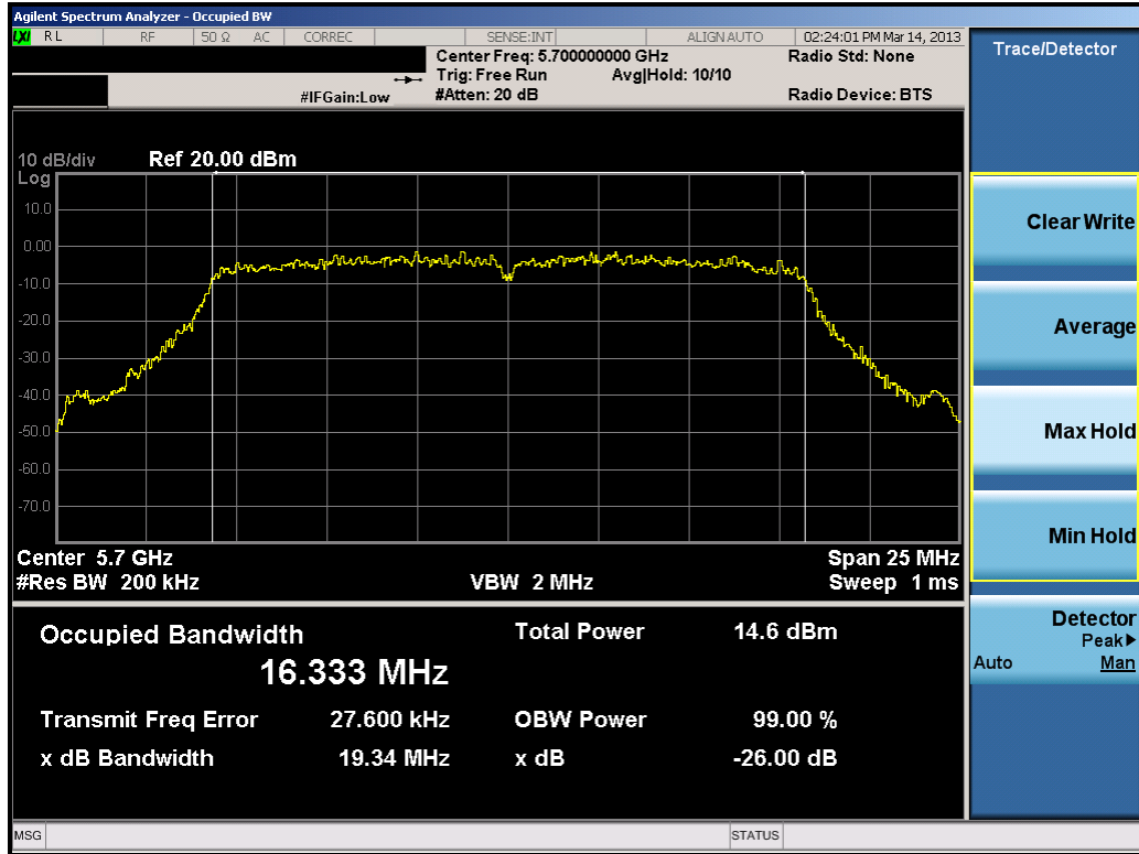
Plot 6-44. 26dB Bandwidth Plot (802.11a (UNII Band 3) – Ch. 140)
