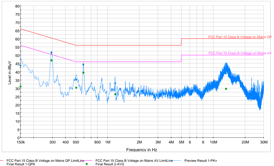
Plot 6-153. Line Conducted Plot with 802.11a UNII Band 3 (L1)
