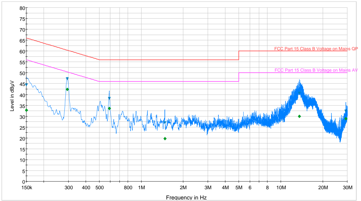
— FCC Part 15 Class B Voltage on Mains QP.LimitLine — FCC Part 15 Class B Voltage on Mains AV.LimitLine — Preview Result 1-PK+ ◆ Final Result 2-AVG ▼ Final Result 1-QPK
