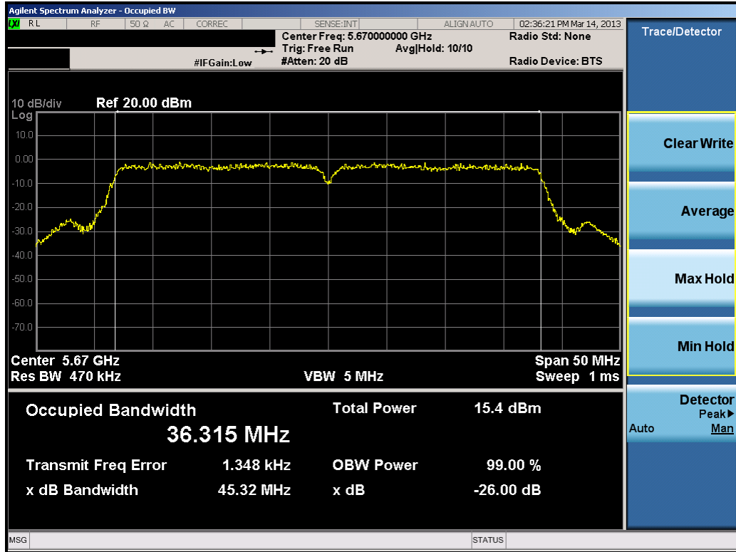
Plot 6-50. 26dB Bandwidth Plot (40MHz BW 802.11n (UNII Band 3) – Ch. 134)
