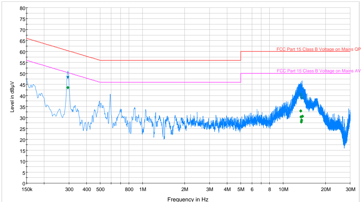
Plot 6-158. Line Conducted Plot with 802.11a UNII Band 2 (N)
