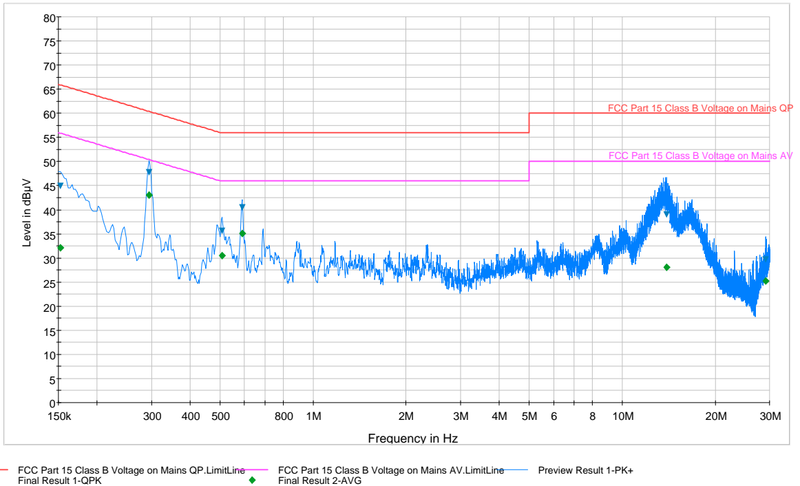
Plot 6-161. Line Conducted Plot with 802.11n UNII Band 1 (L1)
