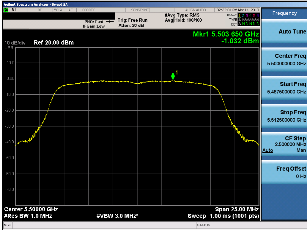
Plot 6-92. Peak Power Spectral Density Plot (802.11a (UNII Band 3) – Ch. 100)
