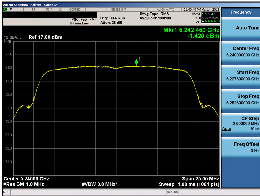
Plot 6-56. Peak Power Spectral Density Plot (20MHz BW 802.11n (UNII Band 1) – Ch. 48)
