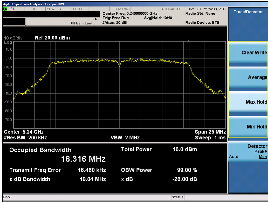
Plot 6-28. 26dB Bandwidth Plot (802.11a (UNII Band 1) – Ch. 48)
