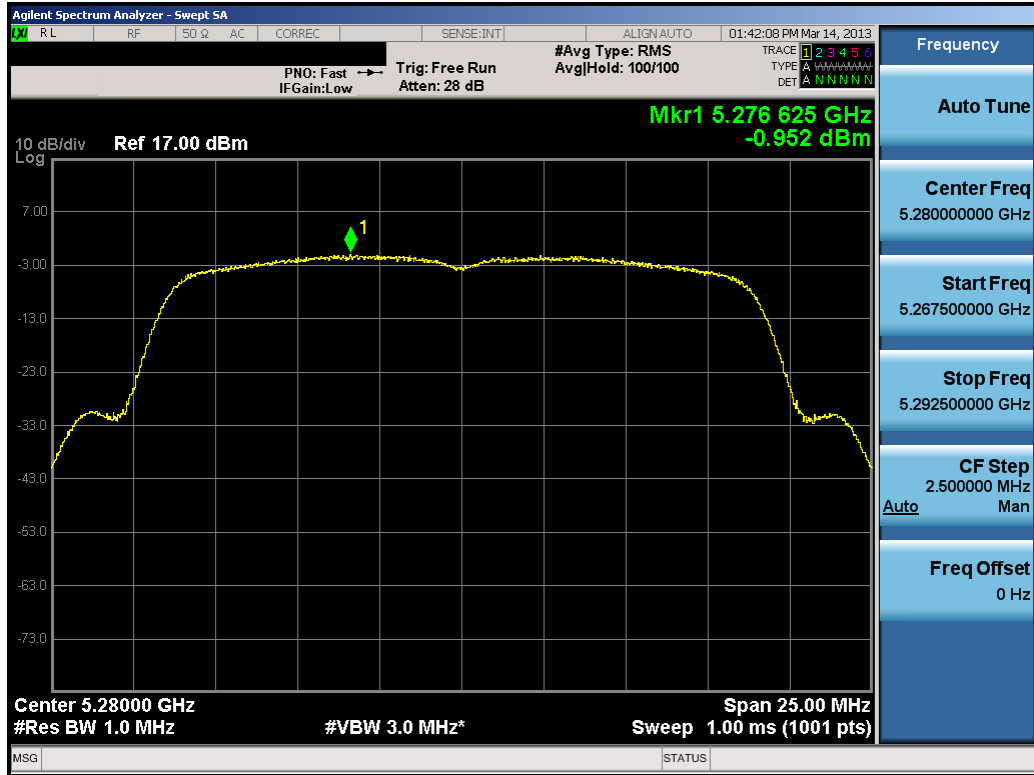
Plot 6-63. Peak Power Spectral Density Plot (20MHz BW 802.11n (UNII Band 2) – Ch. 56)
