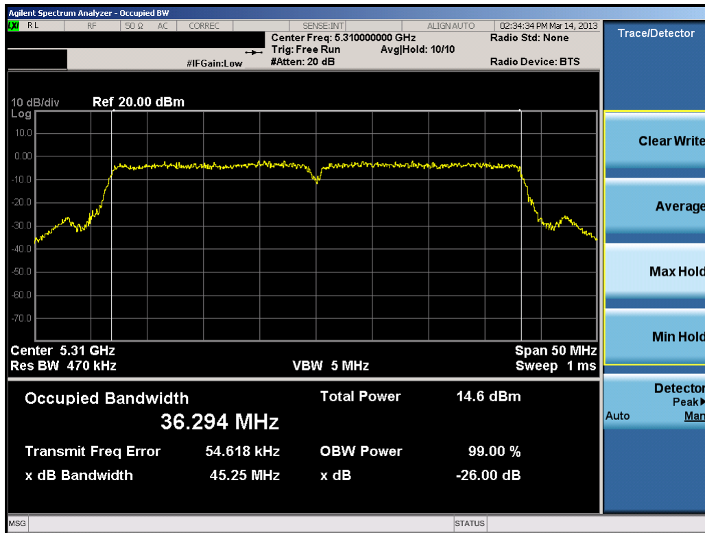
Plot 6-41. 26dB Bandwidth Plot (40MHz BW 802.11n (UNII Band 2) – Ch. 62)
