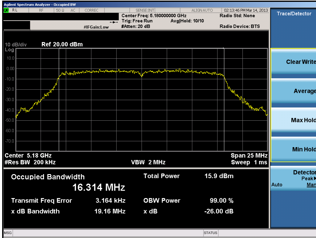
Plot 6-26. 26dB Bandwidth Plot (802.11a (UNII Band 1) – Ch. 36)
