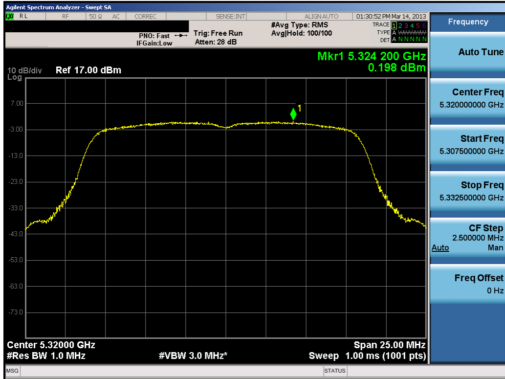
Plot 6-61. Peak Power Spectral Density Plot (802.11a (UNII Band 2) – Ch. 64)
