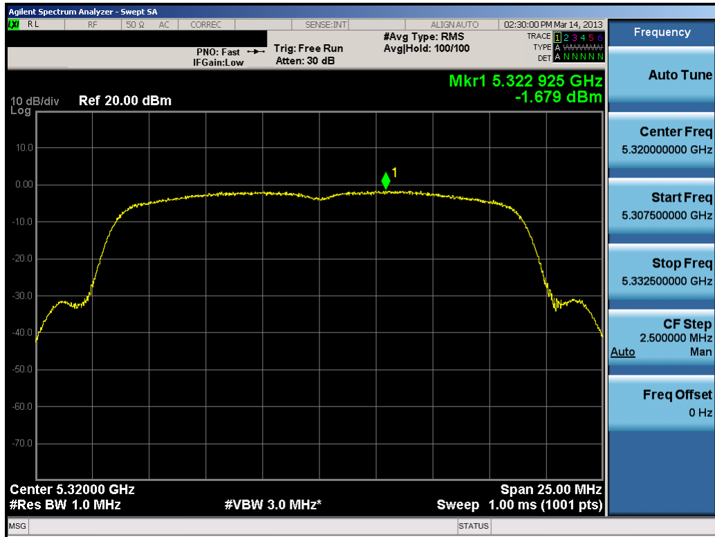
Plot 6-89. Peak Power Spectral Density Plot (20MHz BW 802.11n (UNII Band 2) – Ch. 64)
