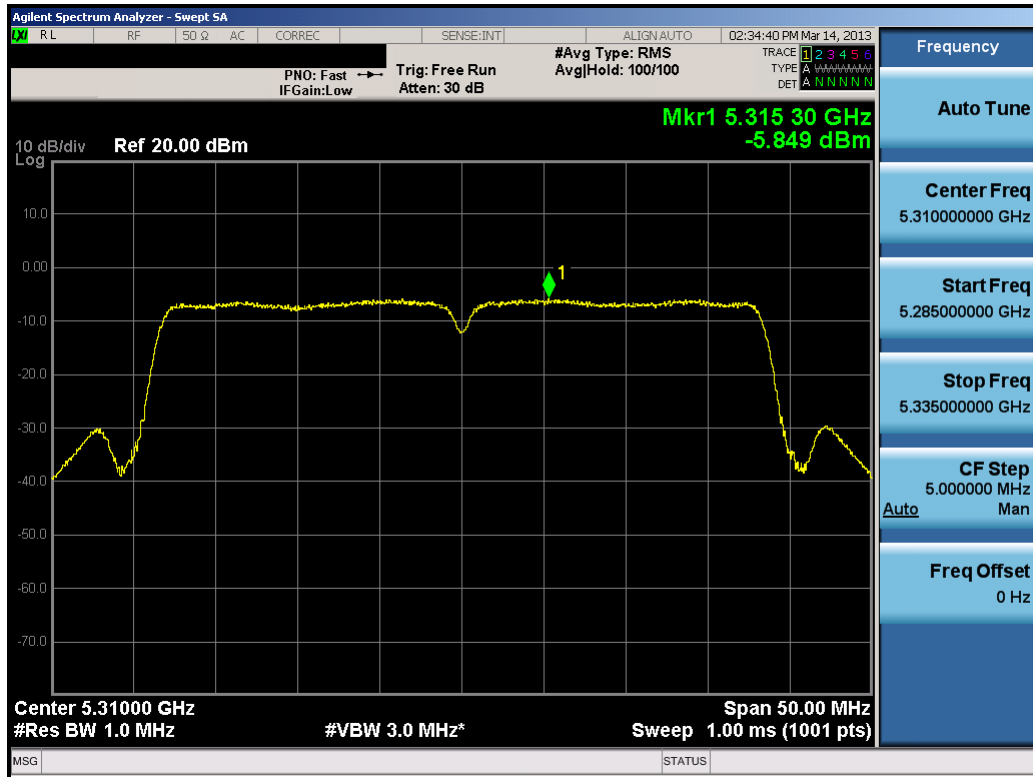
Plot 6-91. Peak Power Spectral Density Plot (40MHz BW 802.11n (UNII Band 2) – Ch. 62)
