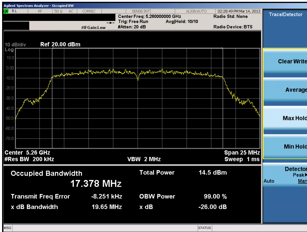
Plot 6-37. 26dB Bandwidth Plot (20MHz BW 802.11n (UNII Band 2) – Ch. 52)
