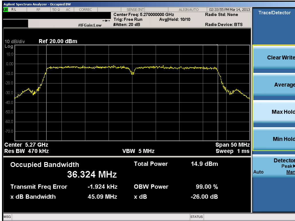
Plot 6-40. 26dB Bandwidth Plot (40MHz BW 802.11n (UNII Band 2) – Ch. 54)
