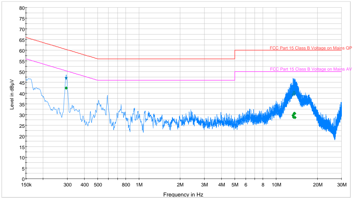
Plot 6-166. Line Conducted Plot with 802.11n UNII Band 3 (N)
