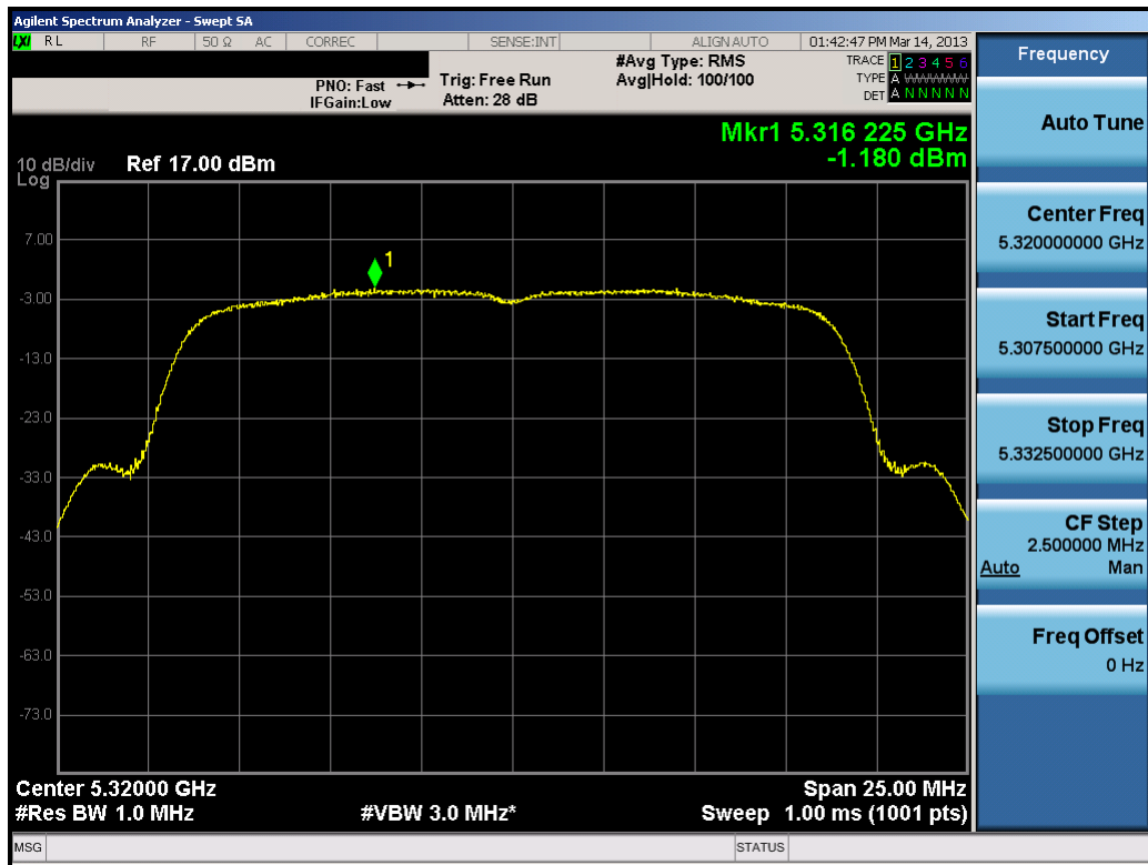
Plot 6-64. Peak Power Spectral Density Plot (20MHz BW 802.11n (UNII Band 2) – Ch. 64)
