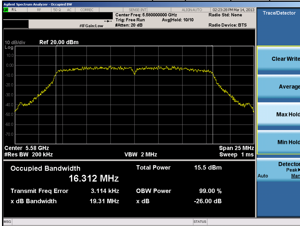
Plot 6-43. 26dB Bandwidth Plot (802.11a (UNII Band 3) – Ch. 116)
