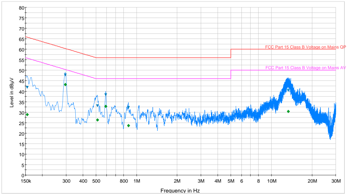
Plot 6-159. Line Conducted Plot with 802.11a UNII Band 3 (L1)
