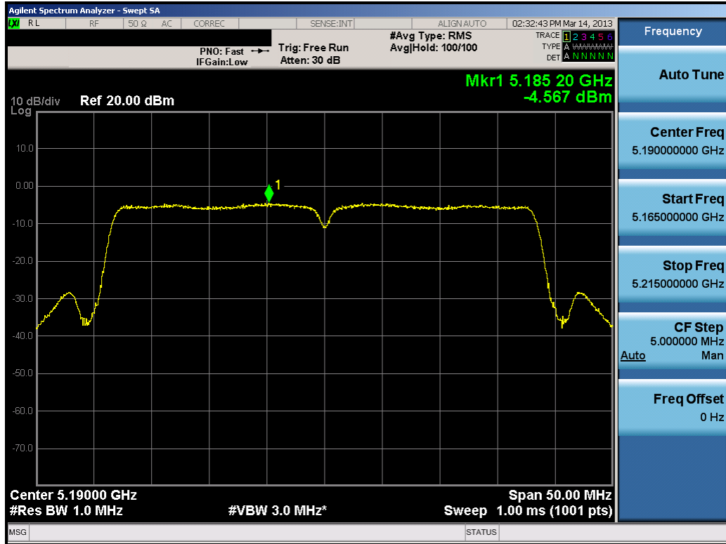
Plot 6-82. Peak Power Spectral Density Plot (40MHz BW 802.11n (UNII Band 1) – Ch. 38)
