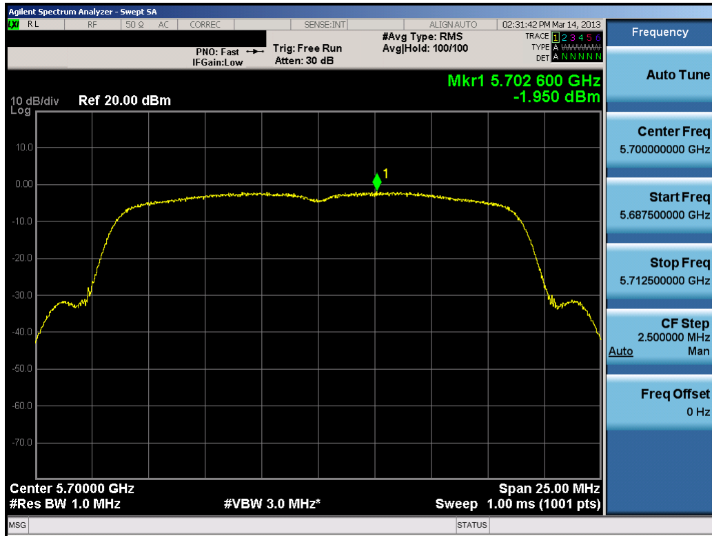
Plot 6-97. Peak Power Spectral Density Plot (20MHz BW 802.11n (UNII Band 3) – Ch. 140)
