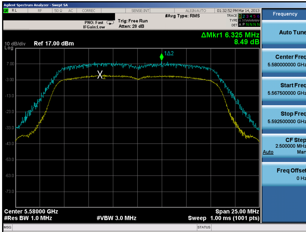
Plot 6-101. Peak Excursion Ratio Plot (802.11a)
