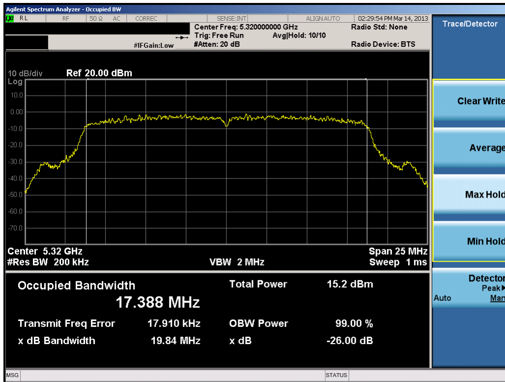
Plot 6-39. 26dB Bandwidth Plot (20MHz BW 802.11n (UNII Band 2) – Ch. 64)
