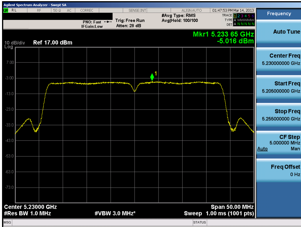
Plot 6-58. Peak Power Spectral Density Plot (40MHz BW 802.11n (UNII Band 1) – Ch. 46)
