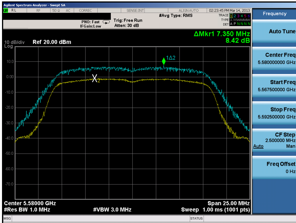
Plot 6-104. Peak Excursion Ratio Plot (802.11a)
