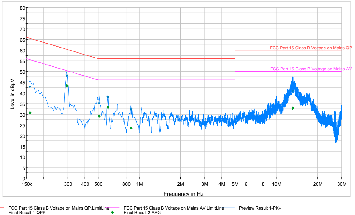
Plot 6-155. Line Conducted Plot with 802.11a UNII Band 1 (L1)
