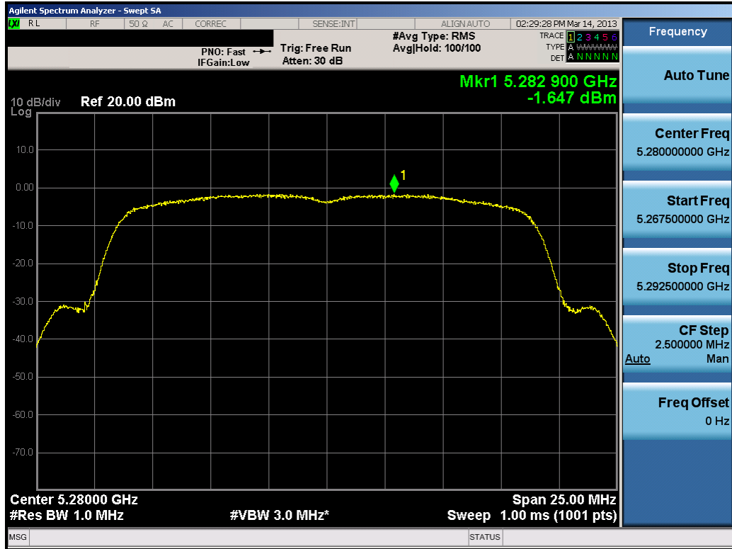
Plot 6-88. Peak Power Spectral Density Plot (20MHz BW 802.11n (UNII Band 2) – Ch. 56)
