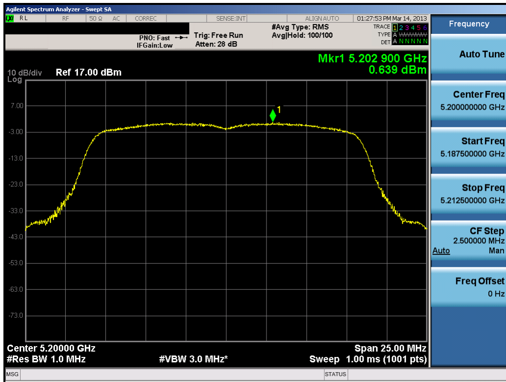
Plot 6-52. Peak Power Spectral Density Plot (802.11a (UNII Band 1) – Ch. 40)
