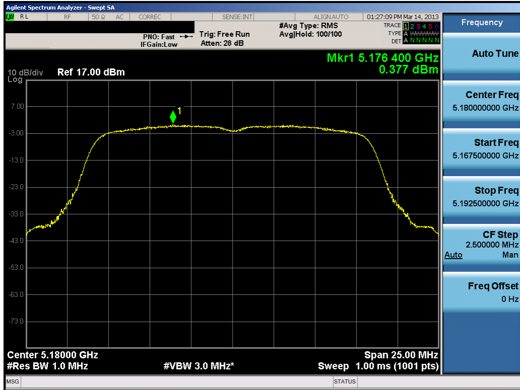
Plot 6-51. Peak Power Spectral Density Plot (802.11a (UNII Band 1) – Ch. 36)
