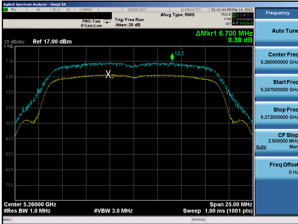
Plot 6-102. Peak Excursion Ratio Plot (20MHz BW 802.11n)
