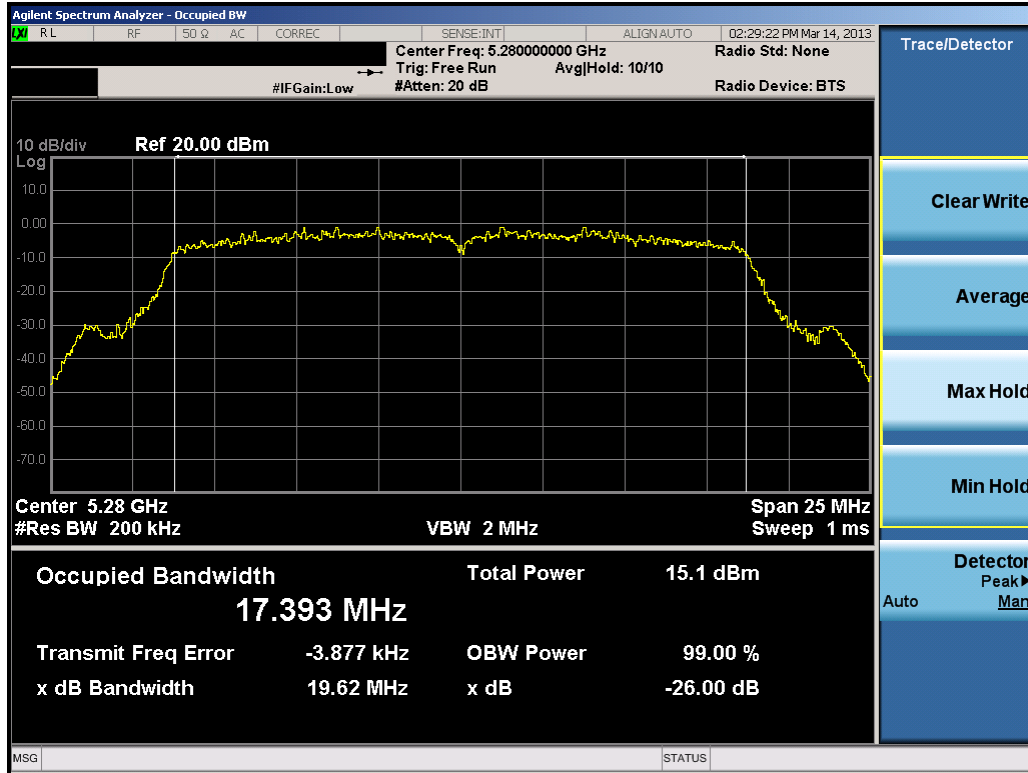
Plot 6-38. 26dB Bandwidth Plot (20MHz BW 802.11n (UNII Band 2) – Ch. 56)
