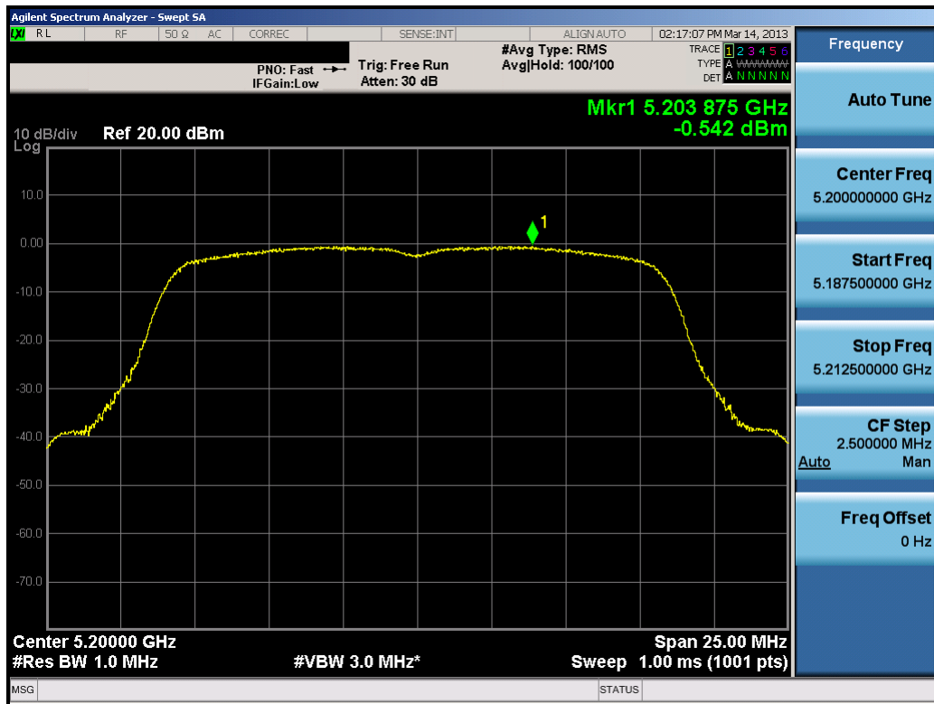
Plot 6-77. Peak Power Spectral Density Plot (802.11a (UNII Band 1) – Ch. 40)
