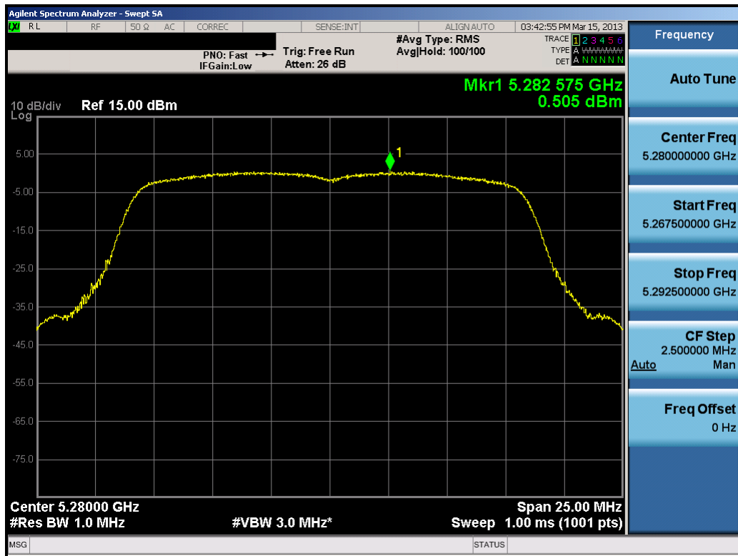
Plot 6-60. Peak Power Spectral Density Plot (802.11a (UNII Band 2) – Ch. 56)
