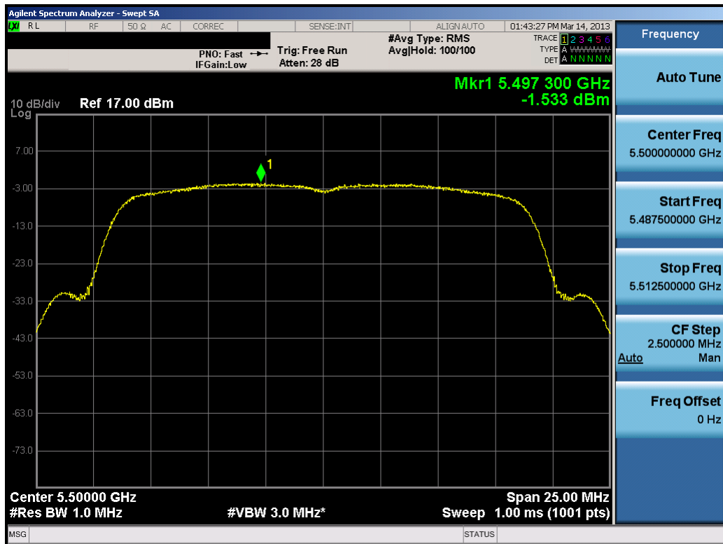
Plot 6-70. Peak Power Spectral Density Plot (20MHz BW 802.11n (UNII Band 3) – Ch. 100)
