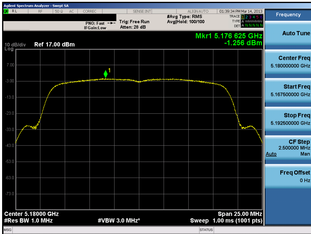
Plot 6-54. Peak Power Spectral Density Plot (20MHz BW 802.11n (UNII Band 1) – Ch. 36)
