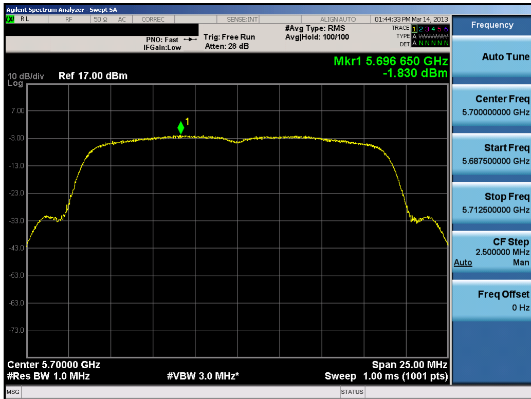
Plot 6-72. Peak Power Spectral Density Plot (20MHz BW 802.11n (UNII Band 3) – Ch. 140)
