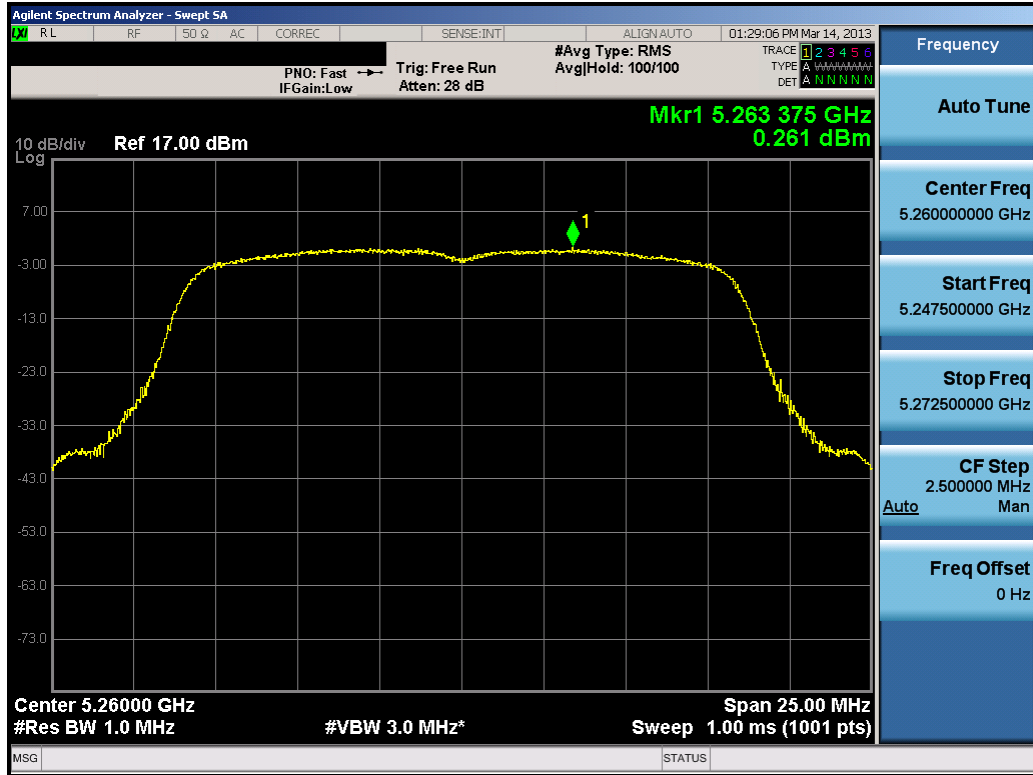
Plot 6-59. Peak Power Spectral Density Plot (802.11a (UNII Band 2) – Ch. 52)
