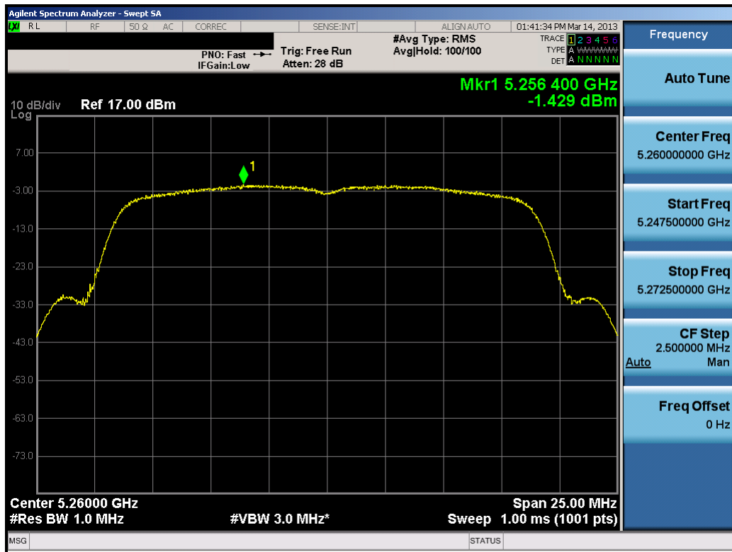
Plot 6-62. Peak Power Spectral Density Plot (20MHz BW 802.11n (UNII Band 2) – Ch. 52)
