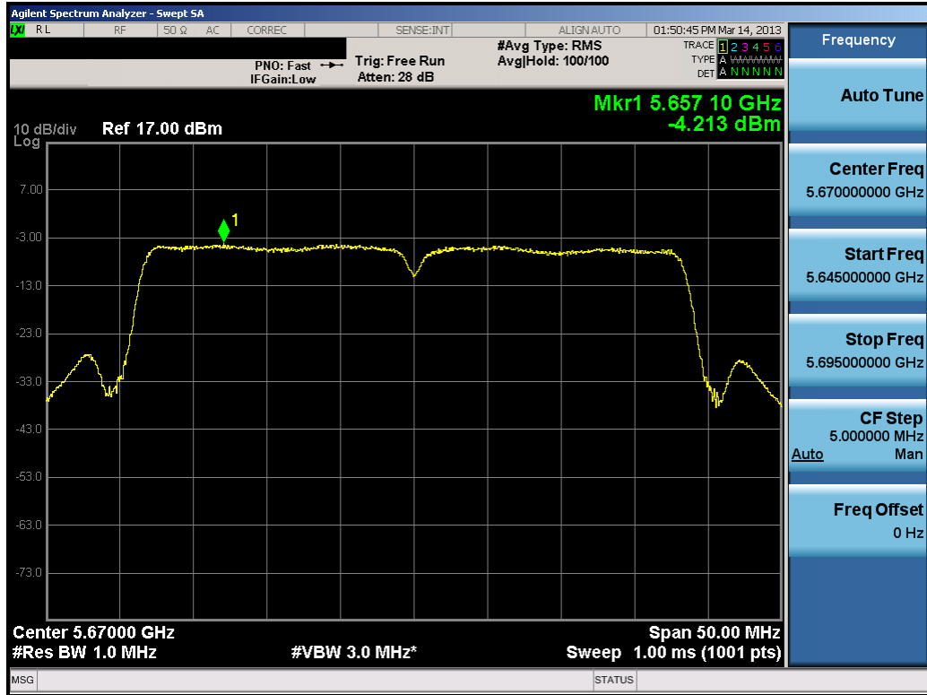
Plot 6-75. Peak Power Spectral Density Plot (40MHz BW 802.11n (UNII Band 3) – Ch. 134)
