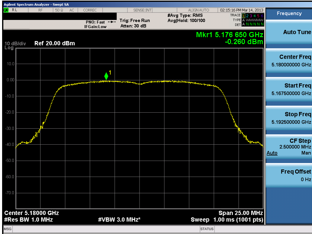
Plot 6-76. Peak Power Spectral Density Plot (802.11a (UNII Band 1) – Ch. 36)
