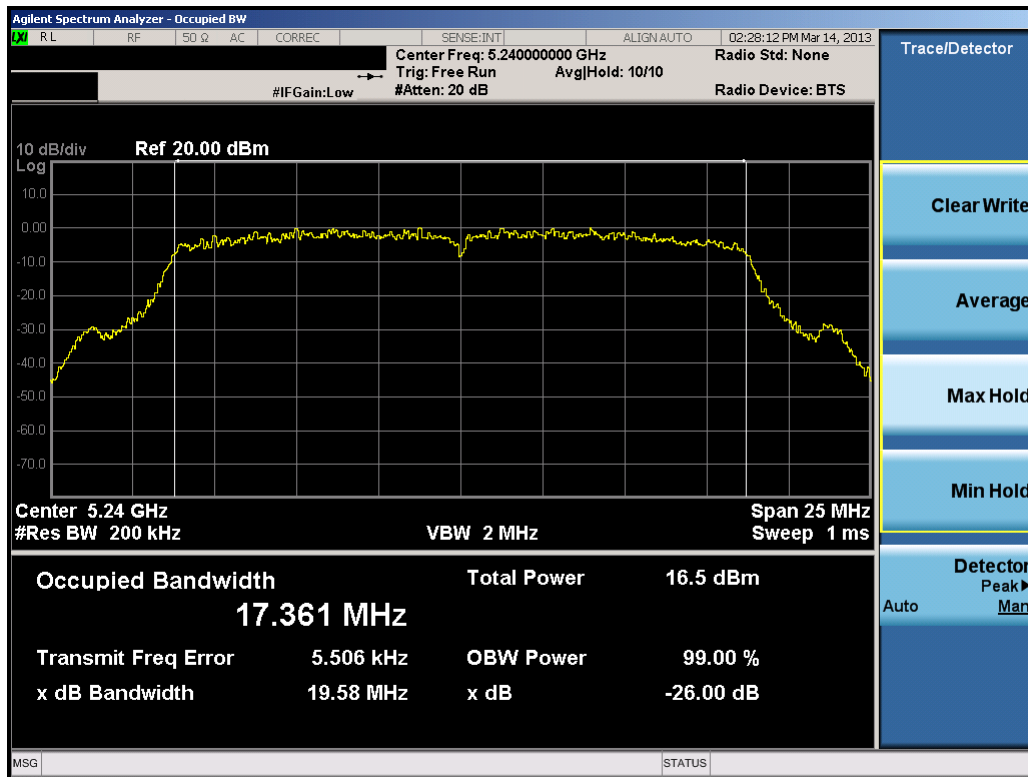
Plot 6-31. 26dB Bandwidth Plot (20MHz BW 802.11n (UNII Band 1) – Ch. 48)
