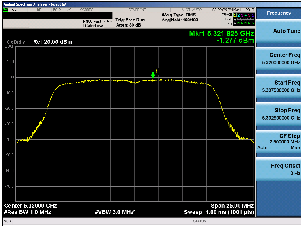
Plot 6-86. Peak Power Spectral Density Plot (802.11a (UNII Band 2) – Ch. 64)
