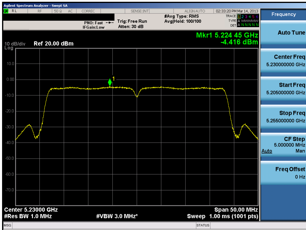
Plot 6-83. Peak Power Spectral Density Plot (40MHz BW 802.11n (UNII Band 1) – Ch. 46)
