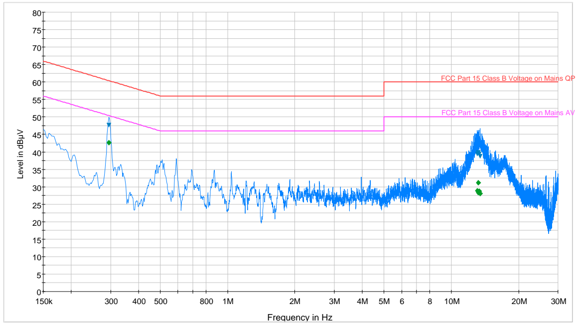
Plot 6-154. Line Conducted Plot with 802.11a UNII Band 3 (N)
