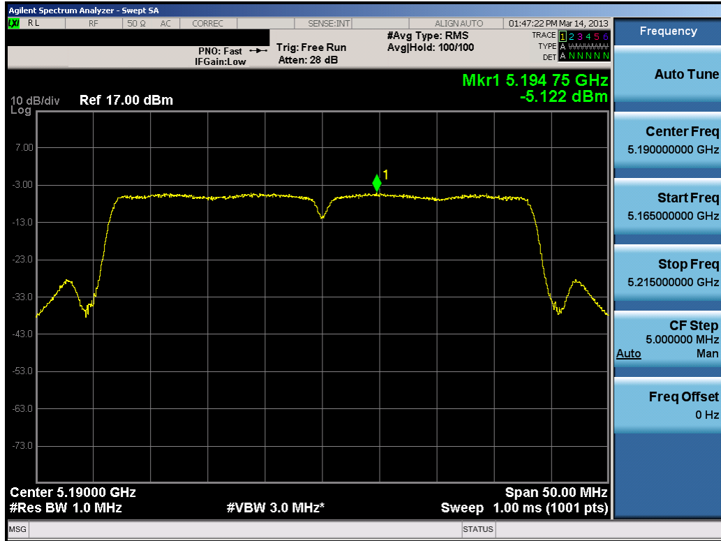
Plot 6-57. Peak Power Spectral Density Plot (40MHz BW 802.11n (UNII Band 1) – Ch. 38)
