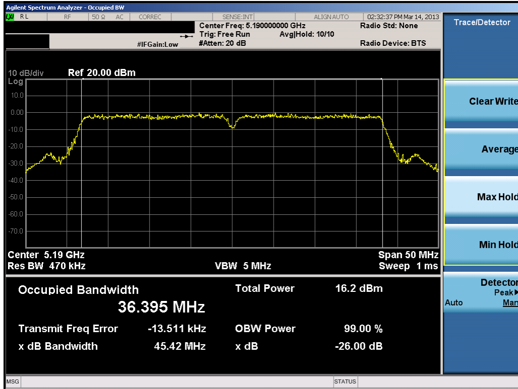
Plot 6-32. 26dB Bandwidth Plot (40MHz BW 802.11n (UNII Band 1) – Ch. 38)
