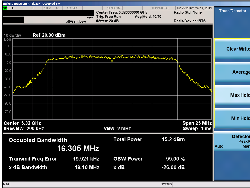
Plot 6-36. 26dB Bandwidth Plot (802.11a (UNII Band 2) – Ch. 64)
