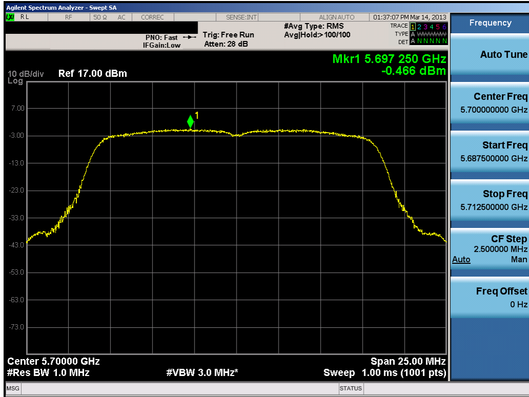
Plot 6-69. Peak Power Spectral Density Plot (802.11a (UNII Band 3) – Ch. 140)
