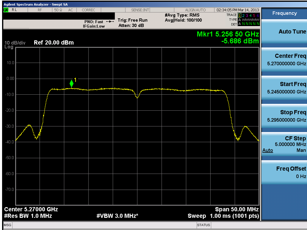
Plot 6-90. Peak Power Spectral Density Plot (40MHz BW 802.11n (UNII Band 2) – Ch. 54)
