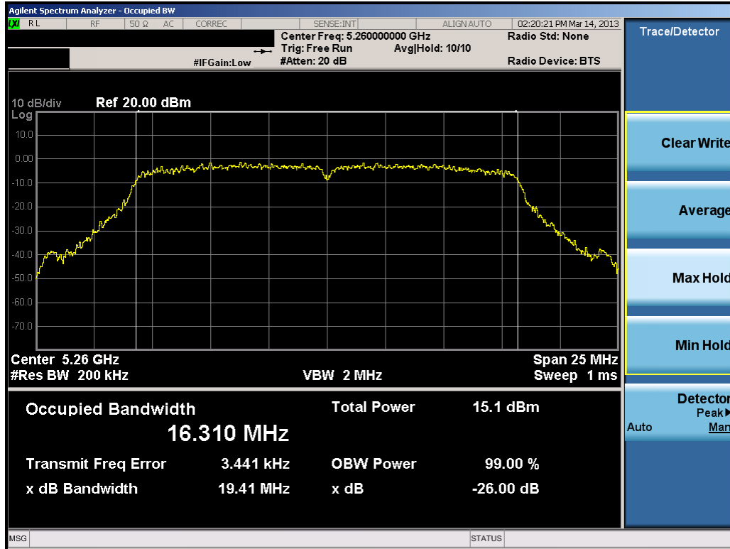
Plot 6-34. 26dB Bandwidth Plot (802.11a (UNII Band 2) – Ch. 52)
