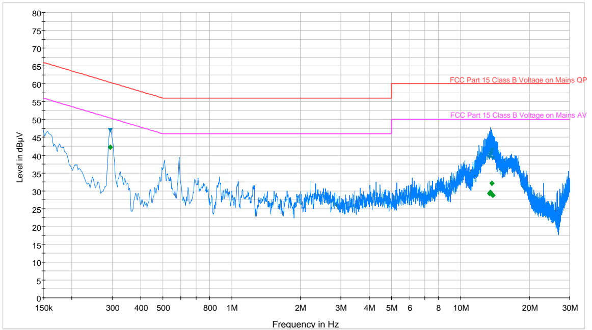
Plot 6-164. Line Conducted Plot with 802.11n UNII Band 2 (N)
