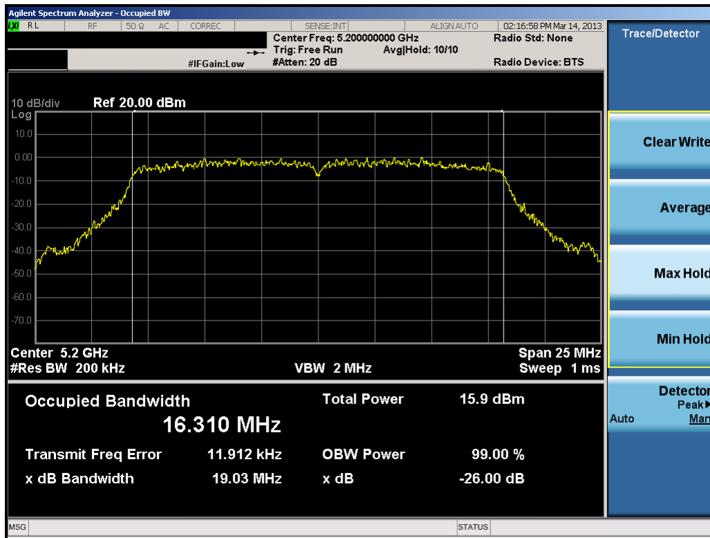
Plot 6-27. 26dB Bandwidth Plot (802.11a (UNII Band 1) – Ch. 40)
