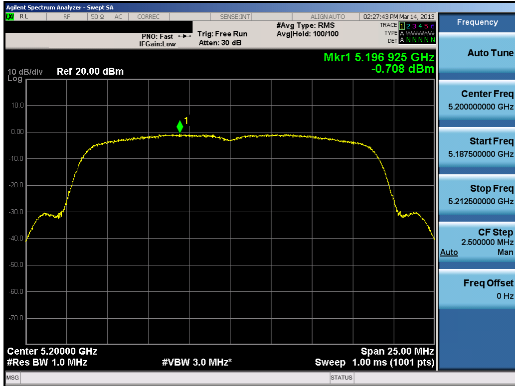
Plot 6-80. Peak Power Spectral Density Plot (20MHz BW 802.11n (UNII Band 1) – Ch. 40)
