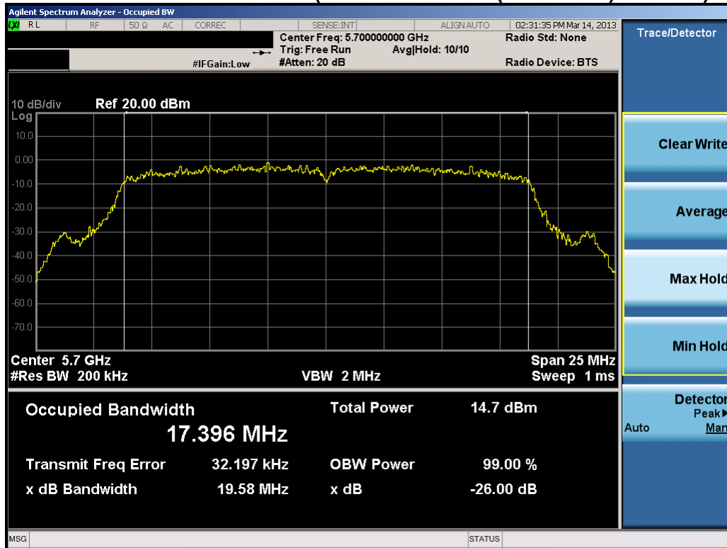
Plot 6-47. 26dB Bandwidth Plot (20MHz BW 802.11n (UNII Band 3) – Ch. 140)
