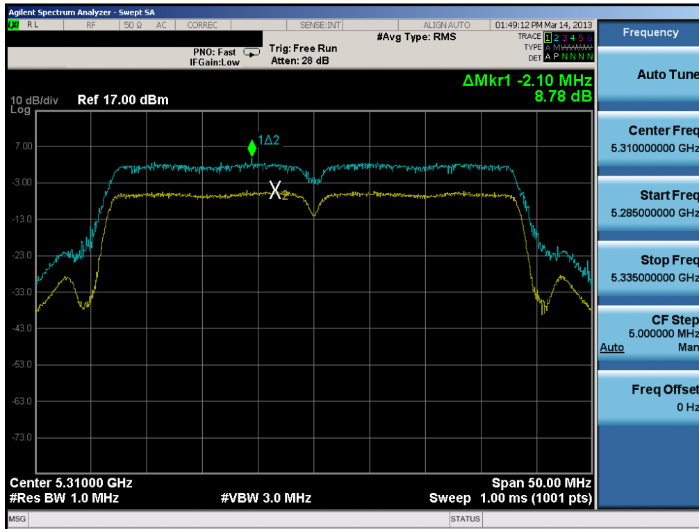
Plot 6-103. Peak Excursion Ratio Plot (40MHz BW 802.11n)
