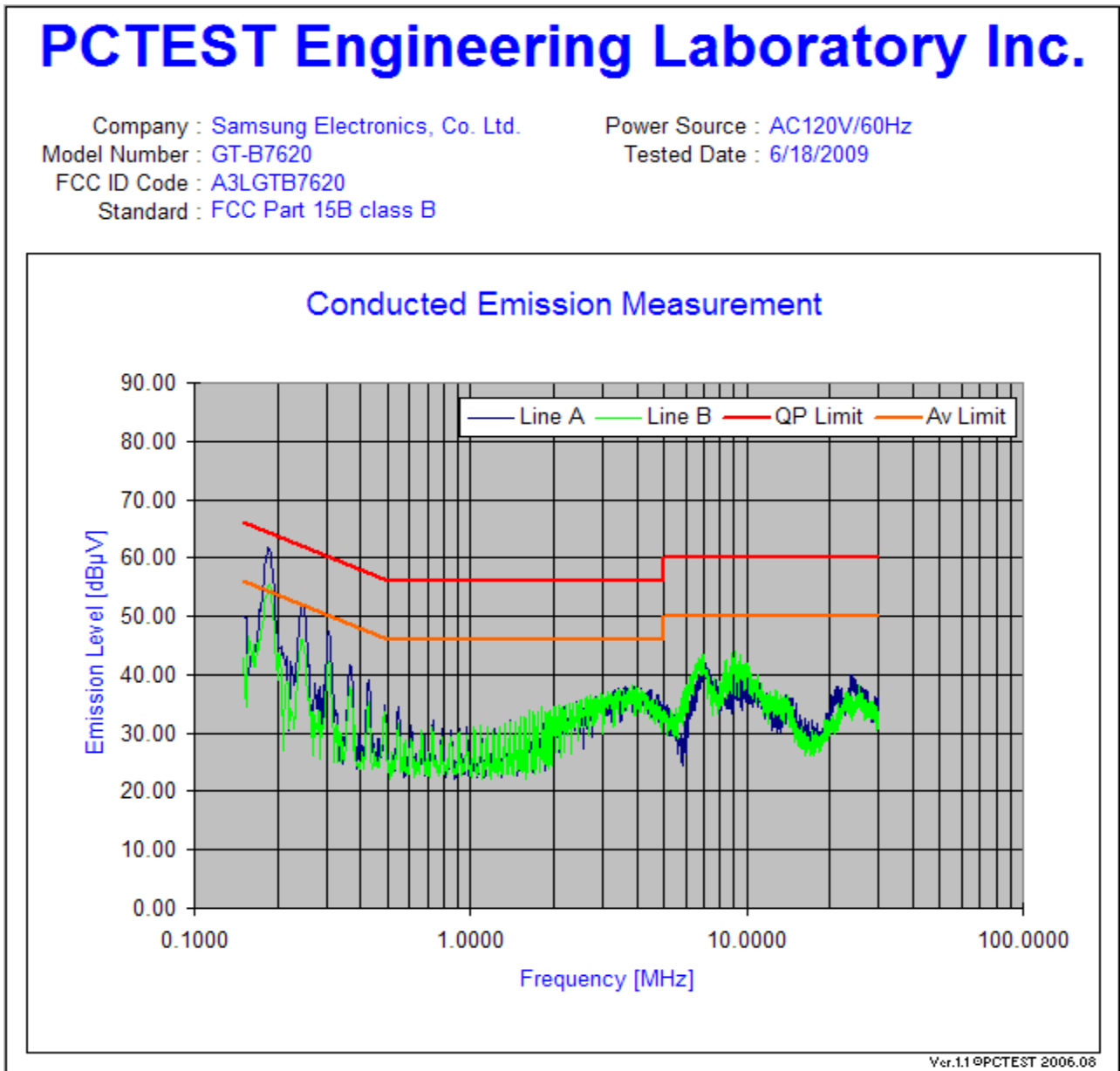
Plot 7-1. Line-Conducted Test Plot
