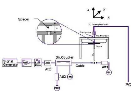
Figure 14-1 System Verification Setup Diagram
