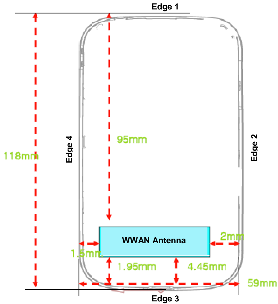
Front View of the DUT
