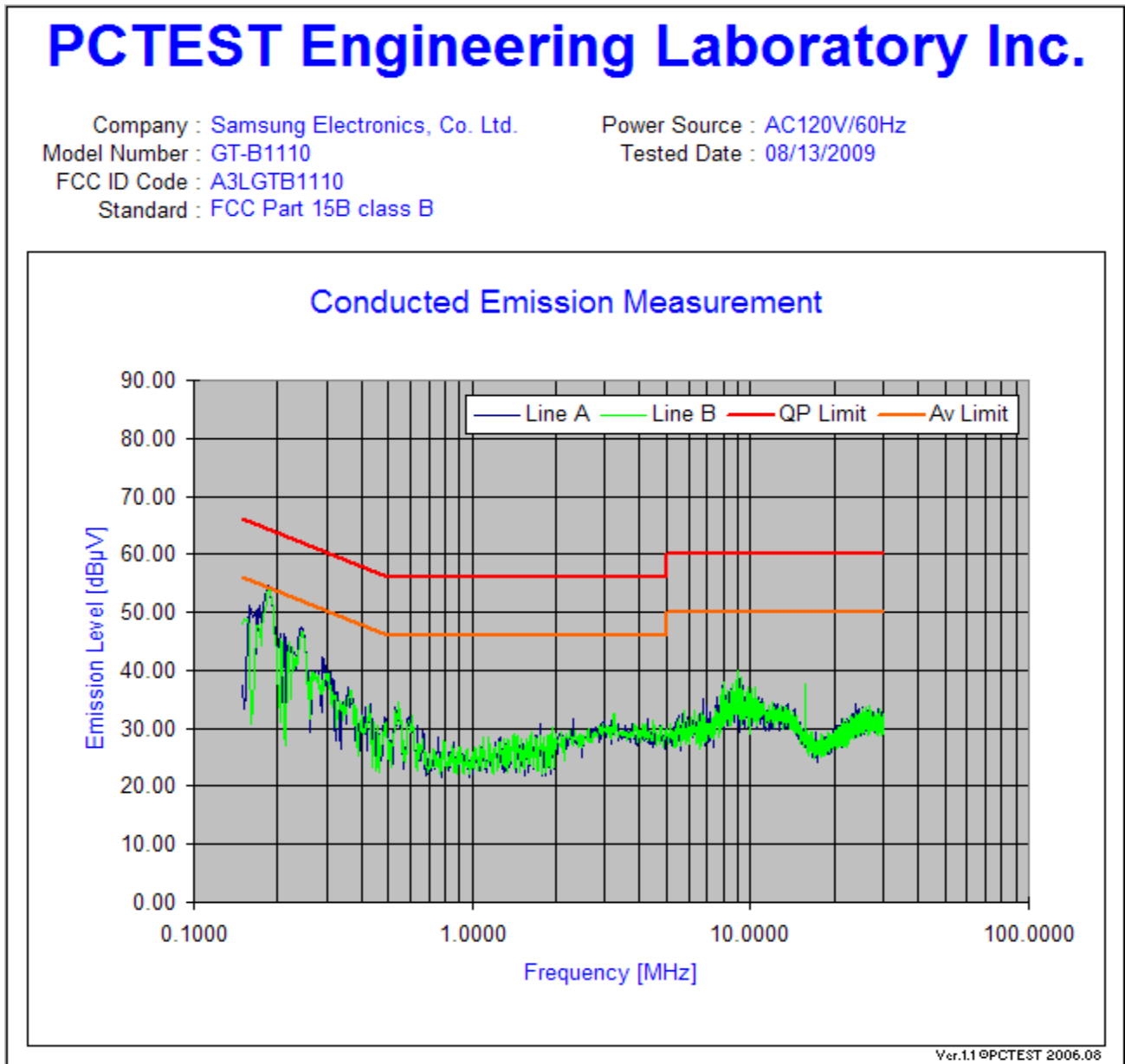
Plot 7-1. Line-Conducted Test Plot
