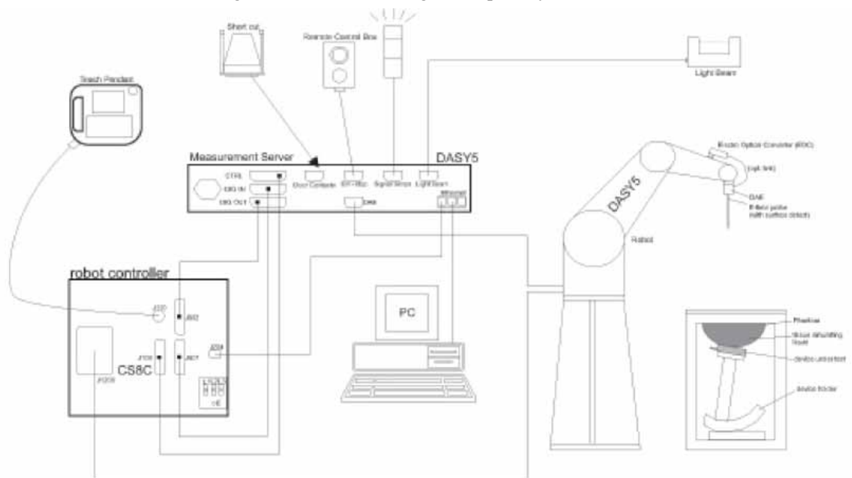
Fig a. The microwave circuit arrangement used for SAR system verification
