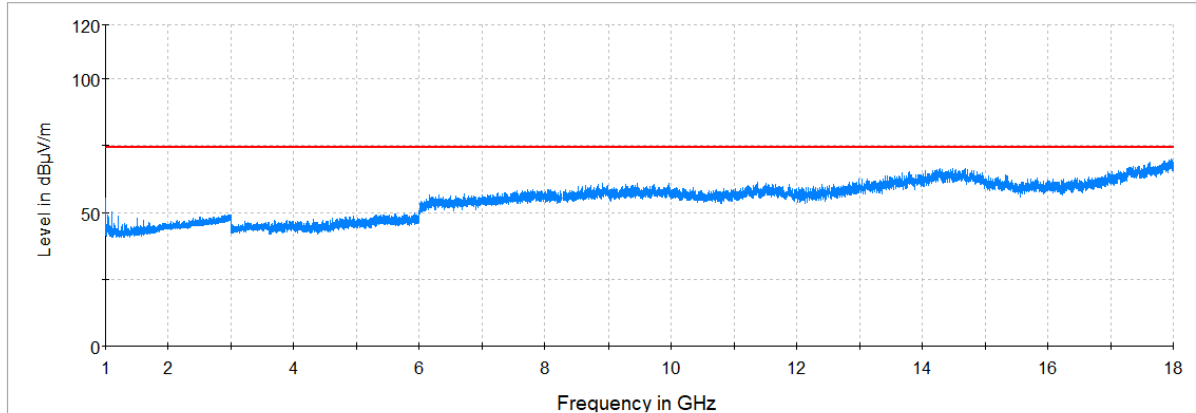
Plot 7-2. Radiated Spurious Plot above 1GHz (Zwave – 921.7MHz, Ant. Pol. H)
