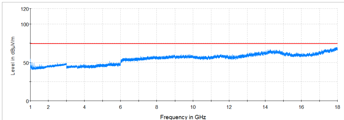
Plot 7-3. Radiated Spurious Plot above 1GHz (Zwave – 921.7MHz, Ant. Pol. V)
