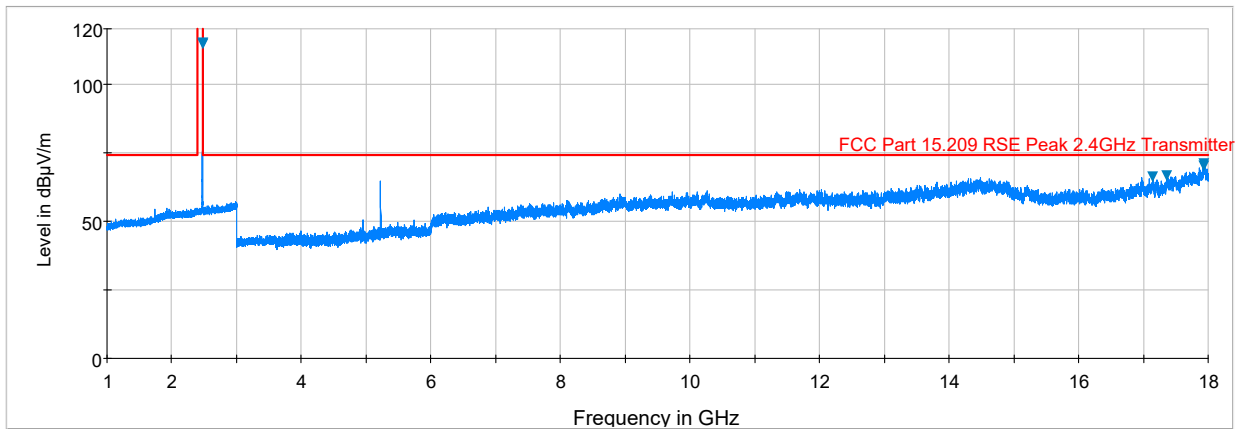
Plot 7-20. Radiated Spurious Plot above 1GHz (Zigbee – Ch. 25, Ant. Pol. V)
