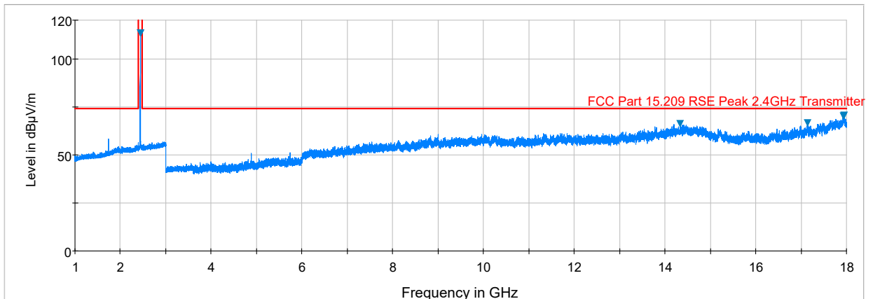
Plot 7-18. Radiated Spurious Plot above 1GHz (Zigbee– Ch. 18, Ant. Pol. V)
