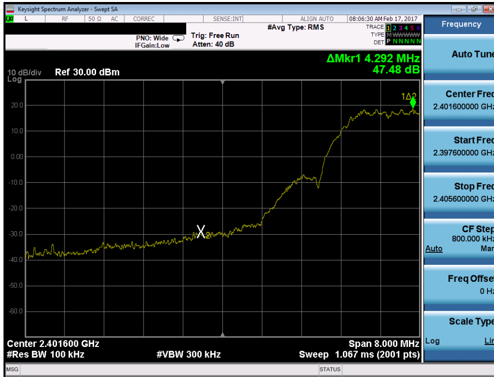
Plot 7-7. Band Edge Plot (ZigBee – Ch. 11)
