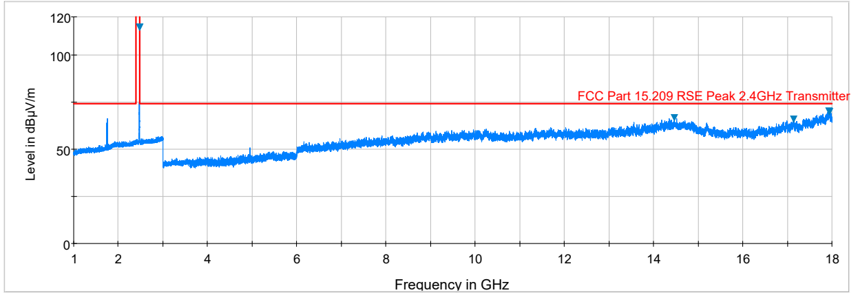
Plot 7-19. Radiated Spurious Plot above 1GHz (Zigbee – Ch. 25, Ant. Pol. H)
