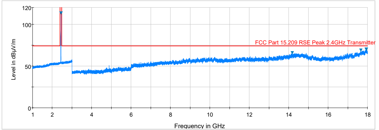
Plot 7-17. Radiated Spurious Plot above 1GHz (Zigbee – Ch. 18, Ant. Pol. H)
