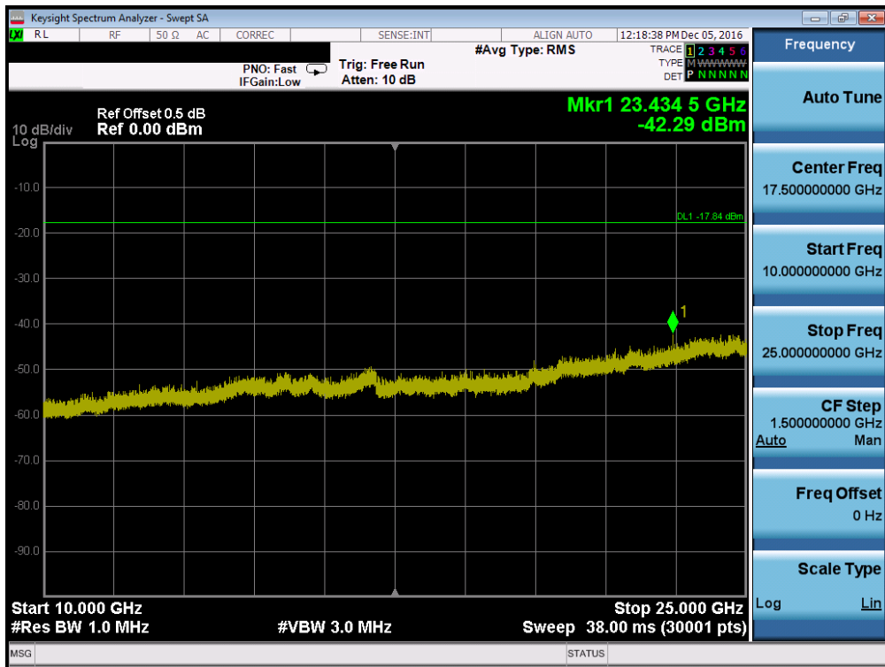
Plot 7-132. Conducted Spurious Plot (802.11b – Ch. 6)
