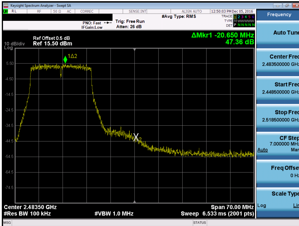
Plot 7-118. Band Edge Plot (802.11n (2.4GHz) – Ch. 11)
