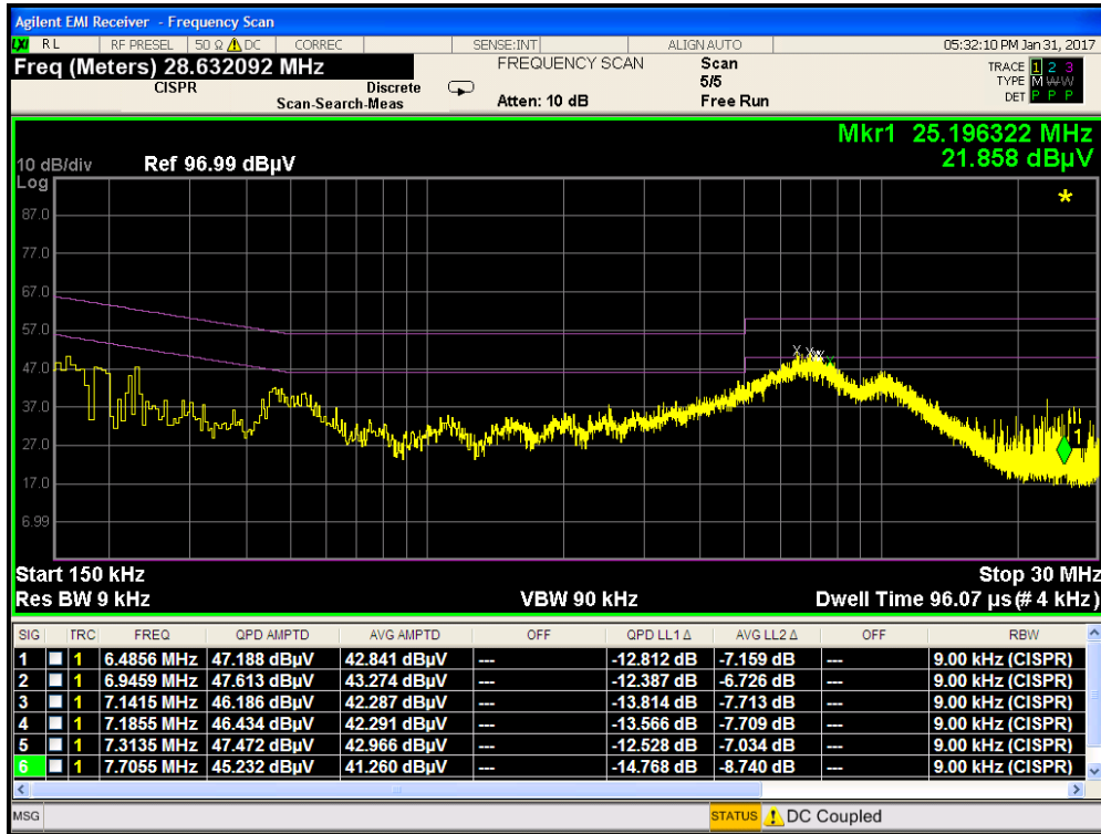
Plot 7-239. Line Conducted Plot with 802.11b (L1)
