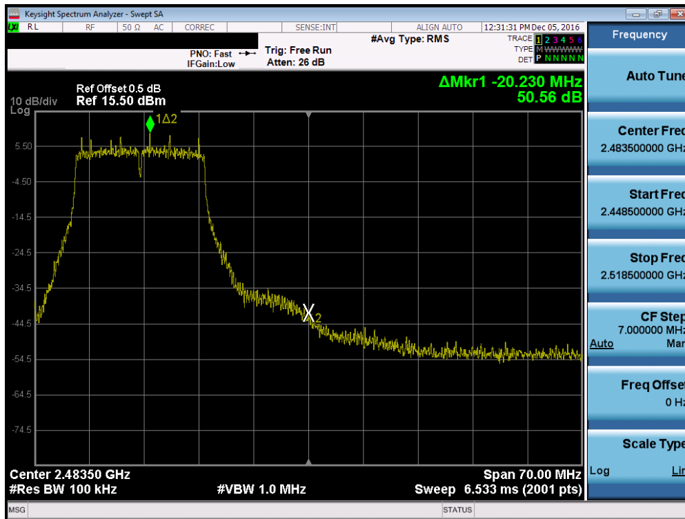
Plot 7-100. Band Edge Plot (802.11g - Ch. 11)
