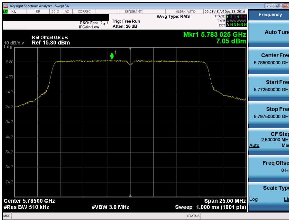
Plot 7-128. Power Spectral Density Plot (802.11a (UNII Band 3) – Ch. 157)
