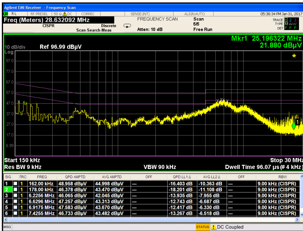
Plot 7-247. Line Conducted Plot with 802.11a UNII Band 1 (L1)
