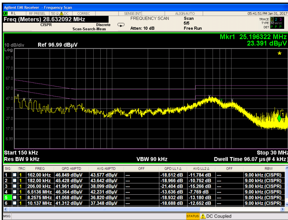
Plot 7-248. Line Conducted Plot with 802.11a UNII Band 1 (N)
