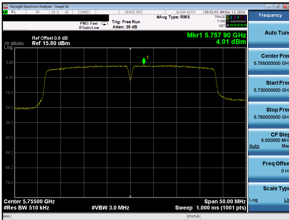
Plot 7-133. Power Spectral Density Plot (40MHz BW 802.11n (UNII Band 3) – Ch. 151)
