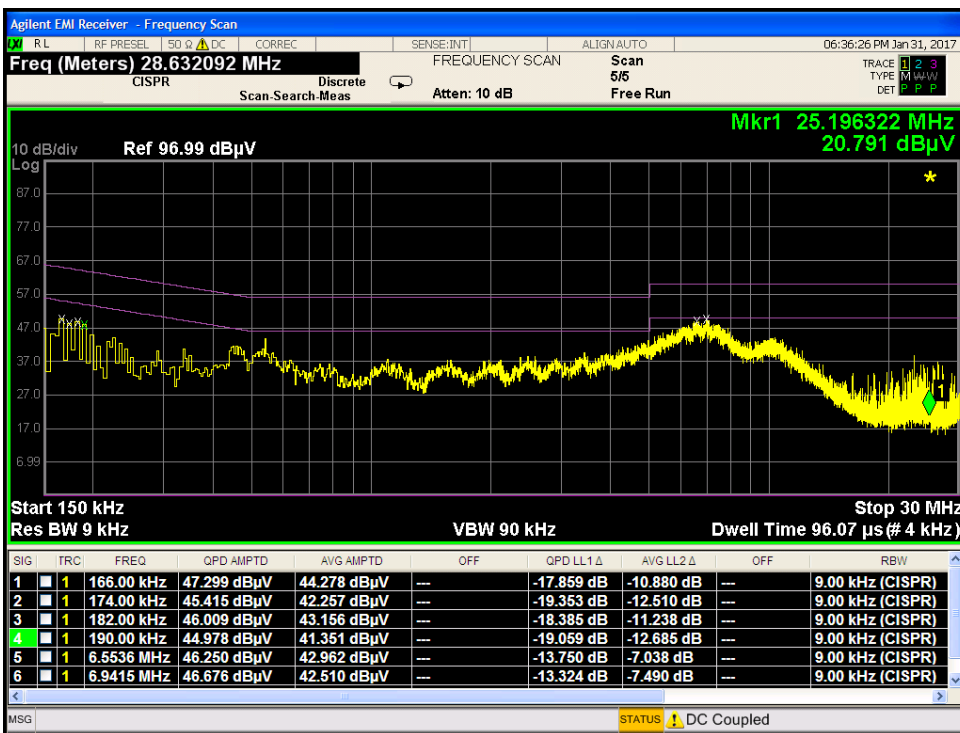
Plot 7-254. Line Conducted Plot with 802.11a UNII Band 3 (N)
