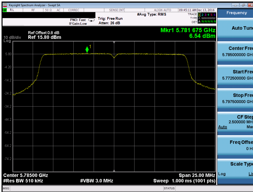
Plot 7-131. Power Spectral Density Plot (20MHz BW 802.11n (UNII Band 3) – Ch. 157)
