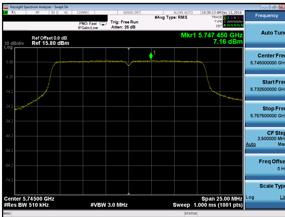
Plot 7-136. Power Spectral Density Plot (802.11a (UNII Band 3) – Ch. 149)
