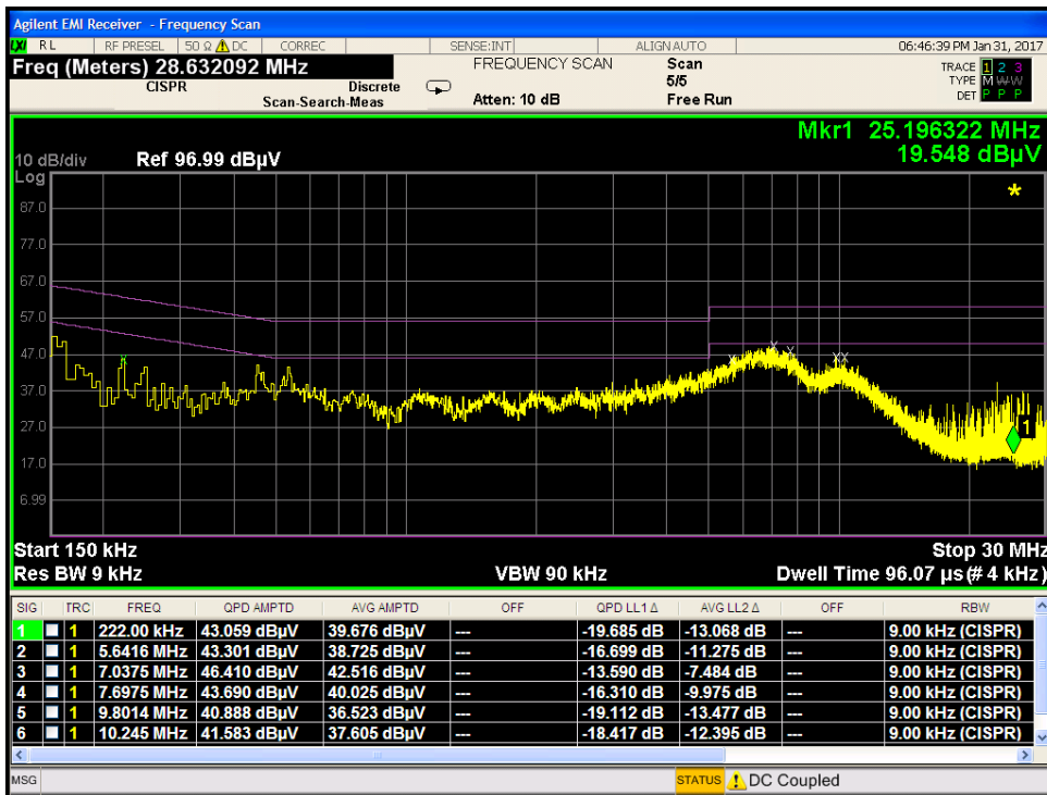
Plot 7-258. Line Conducted Plot with 802.11a UNII Band 3 (N)
