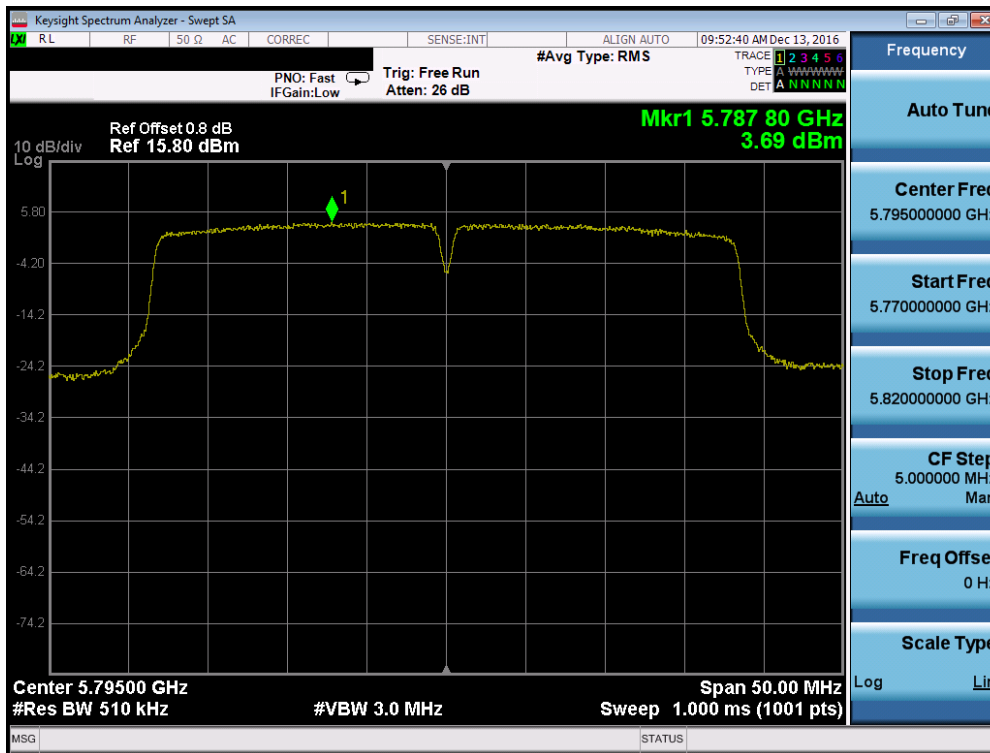
Plot 7-134. Power Spectral Density Plot (40MHz BW 802.11n (UNII Band 3) – Ch. 159)
