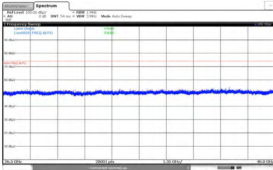
Plot 7-152. Radiated Spurious Plot above 26.5GHz - 40GHz (802.11a – Ant. Pol. V)
