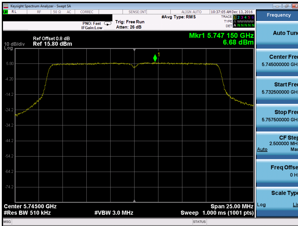
Plot 7-139. Power Spectral Density Plot (20MHz BW 802.11n (UNII Band 3) – Ch. 149)
