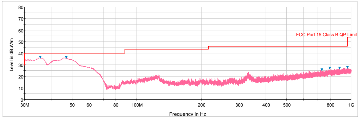
Plot 7-241. Radiated Spurious Plot below 1GHz (802.11a – U3 Ch. 157, Ant. Pol. H)
