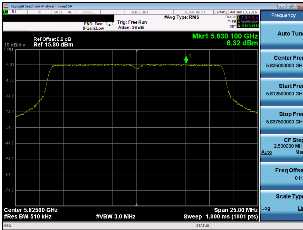
Plot 7-132. Power Spectral Density Plot (20MHz BW 802.11n (UNII Band 3) – Ch. 165)
