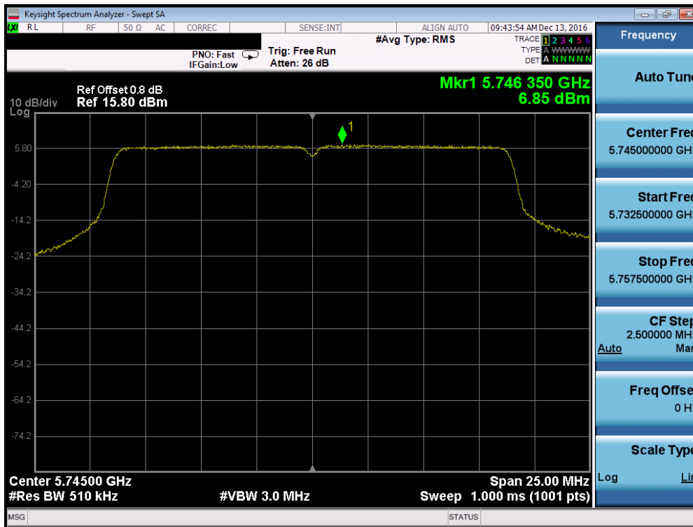
Plot 7-130. Power Spectral Density Plot (20MHz BW 802.11n (UNII Band 3) – Ch. 149)
