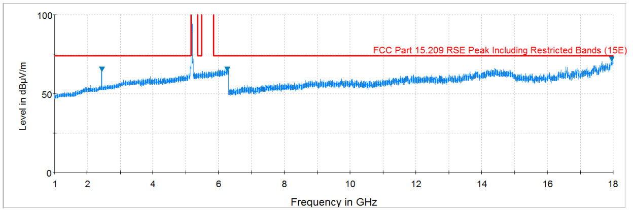
Plot 7-145. Radiated Spurious Plot above 1GHz (802.11a – U1 Ch. 40, Ant. Pol. H)
