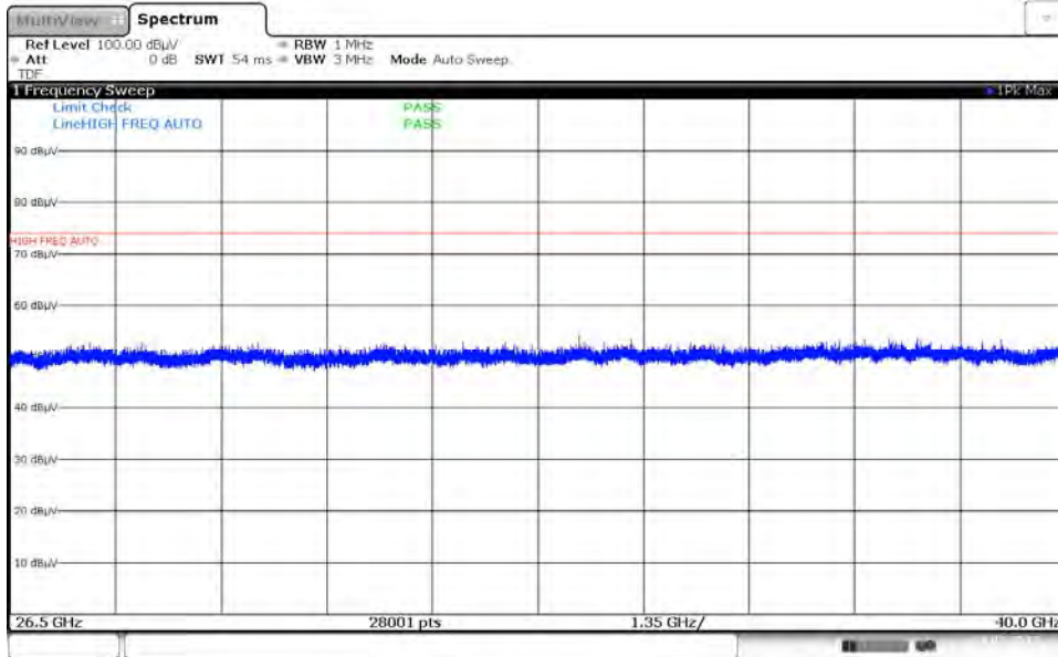
Plot 7-159. Radiated Spurious Plot 26.5GHz - 40GHz (802.11a – Ant. Pol. H)
