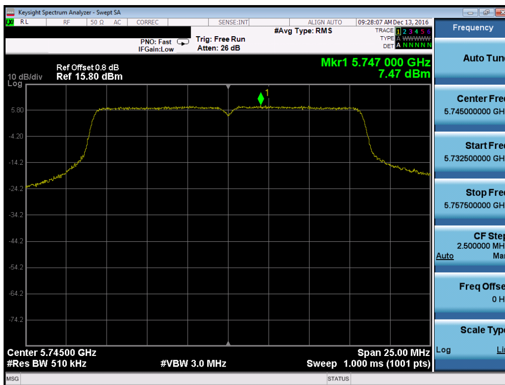
Plot 7-127. Power Spectral Density Plot (802.11a (UNII Band 3) – Ch. 149)
