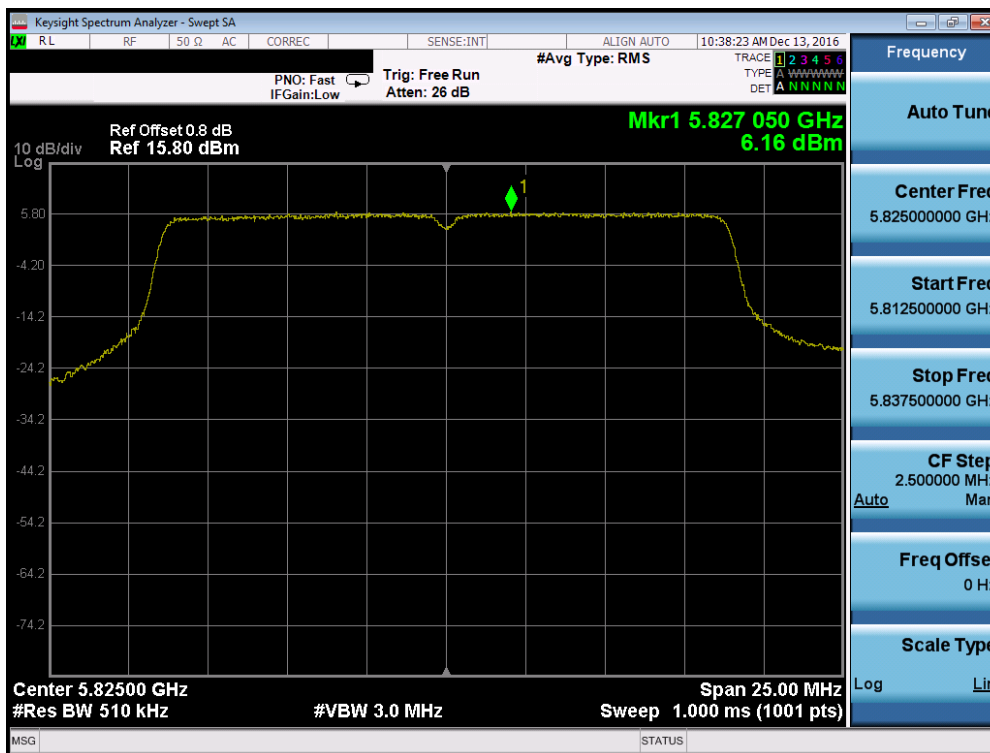
Plot 7-141. Power Spectral Density Plot (20MHz BW 802.11n (UNII Band 3) – Ch. 165)
