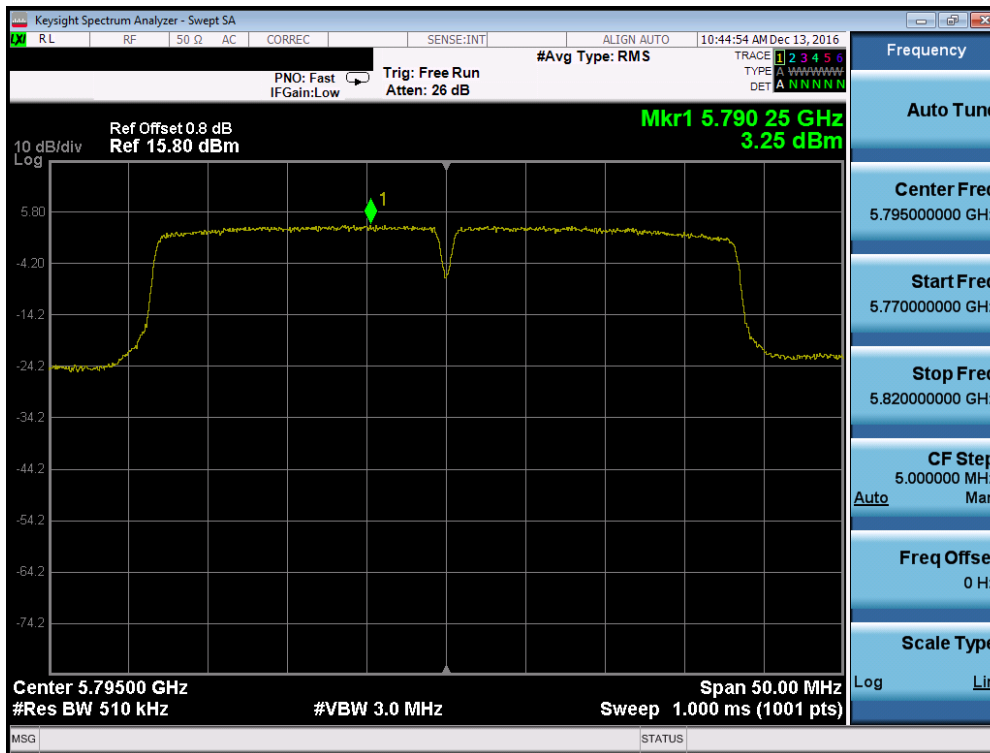
Plot 7-143. Power Spectral Density Plot (40MHz BW 802.11n (UNII Band 3) – Ch. 159)
