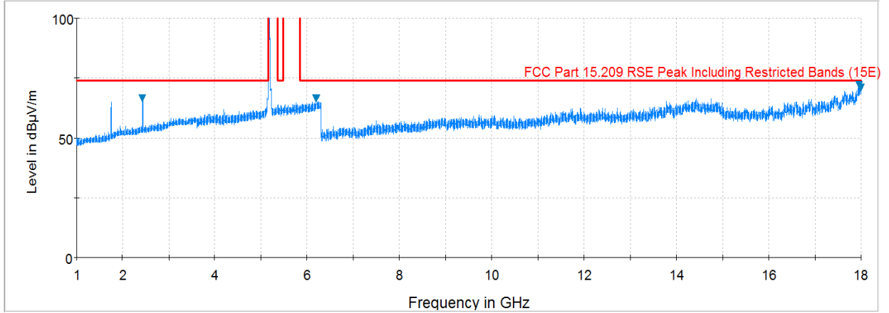
Plot 7-145. Radiated Spurious Plot above 1GHz (802.11a – U1 Ch. 40, Ant. Pol. H)
