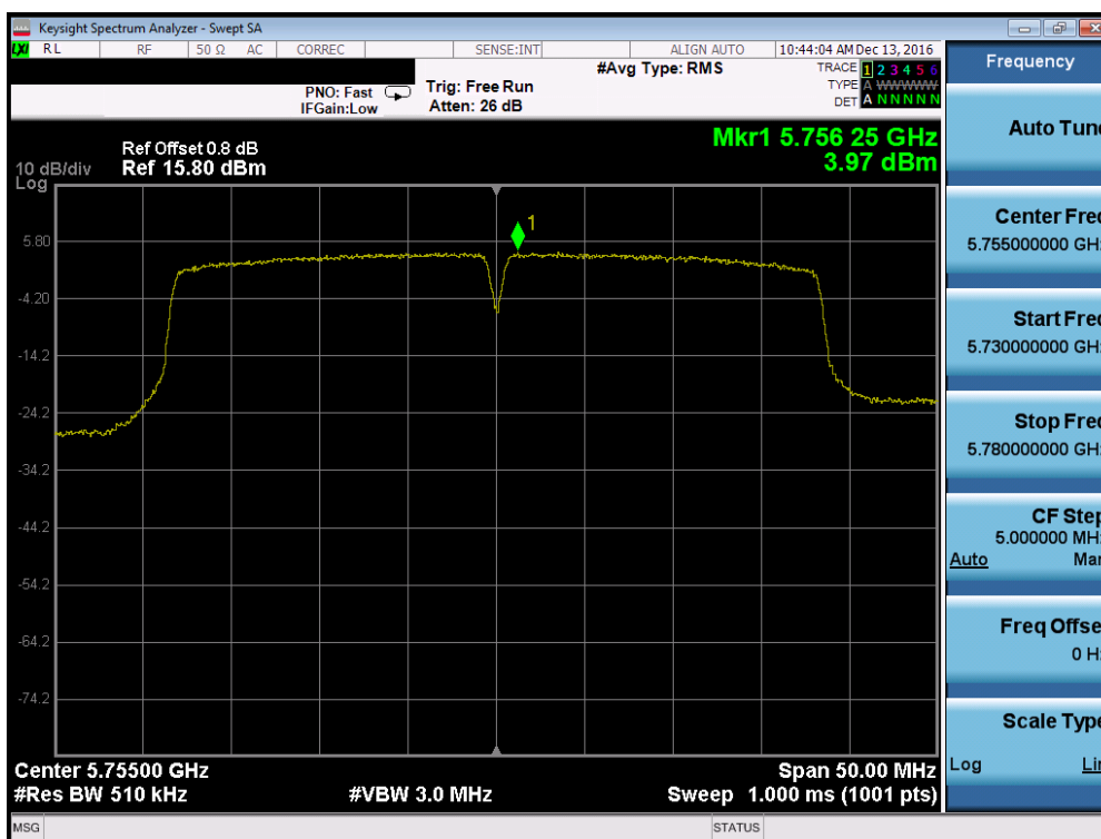
Plot 7-142. Power Spectral Density Plot (40MHz BW 802.11n (UNII Band 3) – Ch. 151)
