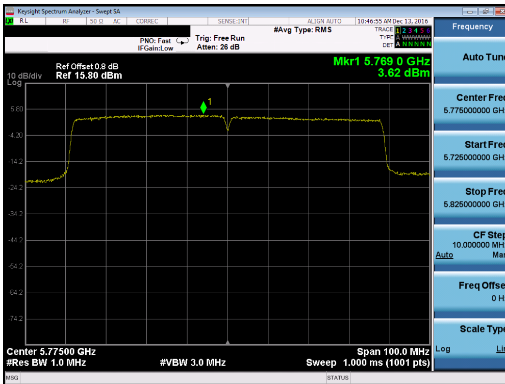
Plot 7-144. Power Spectral Density Plot (80MHz BW 802.11ac (UNII Band 3) – Ch. 155)
