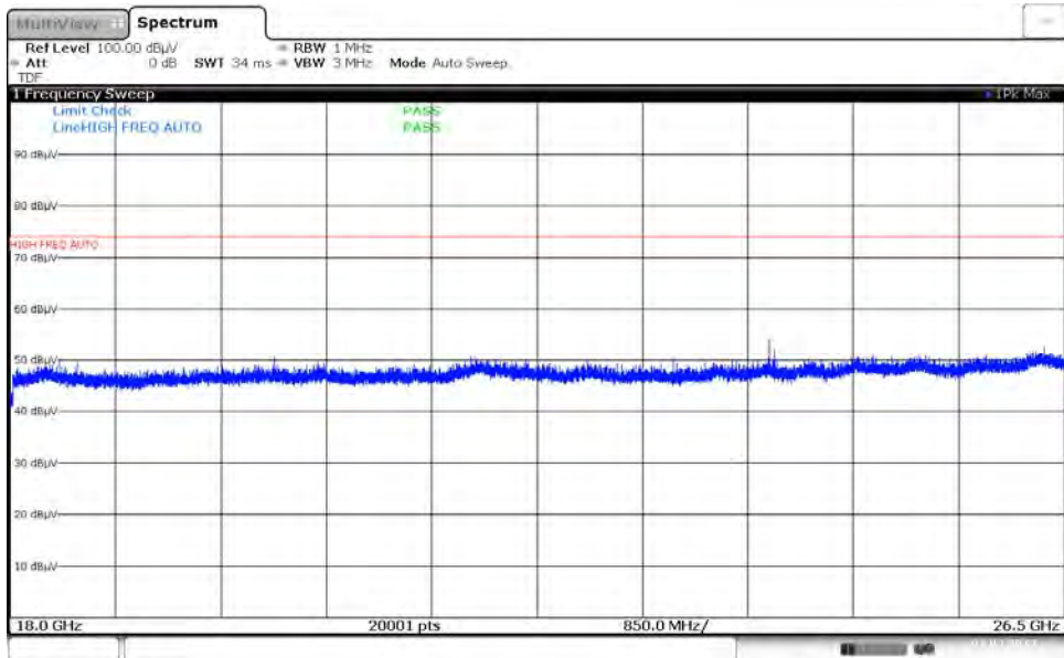
Plot 7-150. Radiated Spurious Plot above 18GHz - 26.5GHz (802.11a – Ant. Pol. V)
