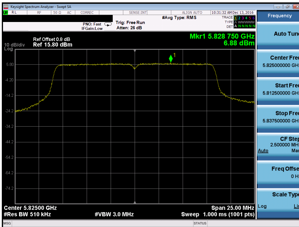
Plot 7-138. Power Spectral Density Plot (802.11a (UNII Band 3) – Ch. 165)
