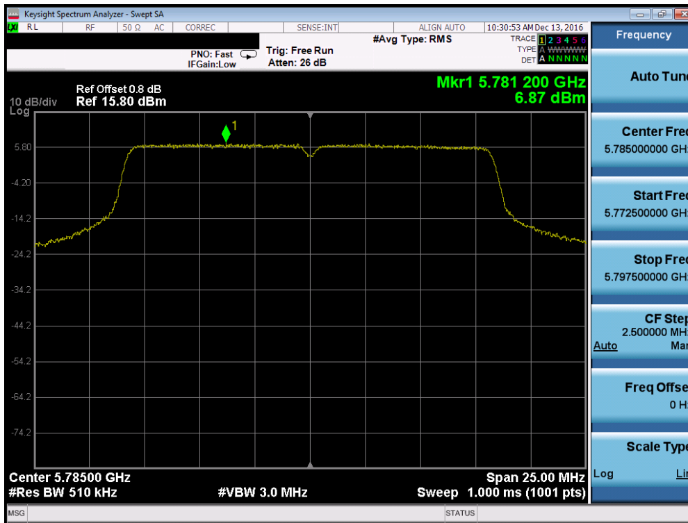
Plot 7-137. Power Spectral Density Plot (802.11a (UNII Band 3) – Ch. 157)
