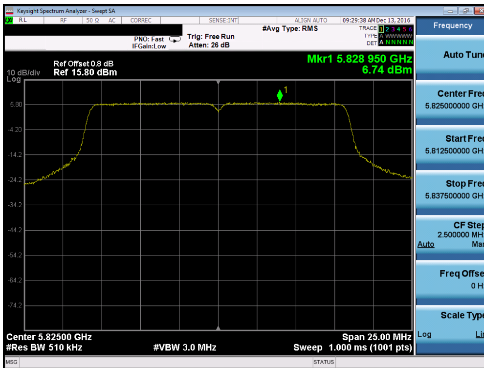
Plot 7-129. Power Spectral Density Plot (802.11a (UNII Band 3) – Ch. 165)
