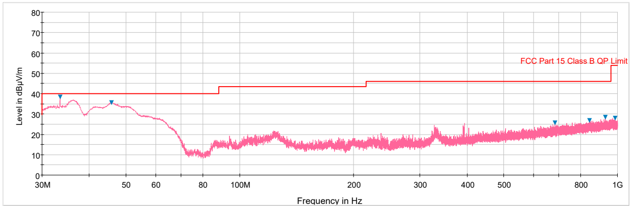
Plot 7-239. Radiated Spurious Plot below 1GHz (802.11a – U3 Ch. 157, Ant. Pol. H)
