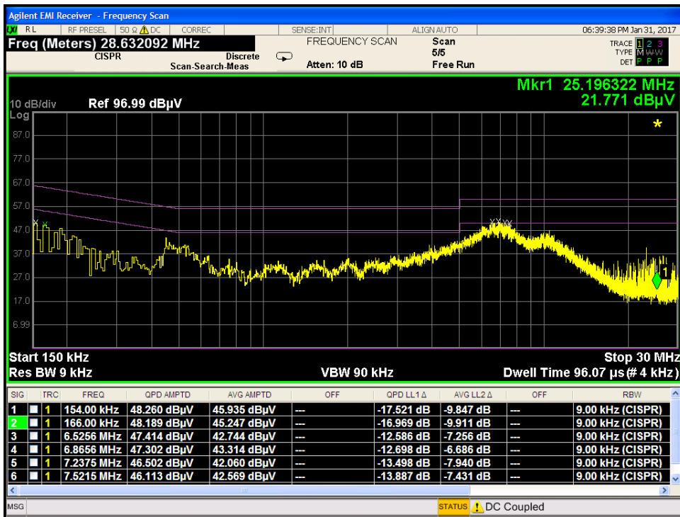
Plot 7-253. Line Conducted Plot with 802.11a UNII Band 3 (L1)
