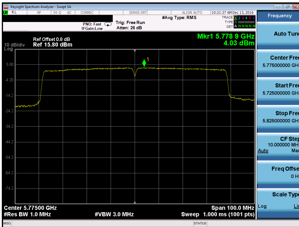
Plot 7-135. Power Spectral Density Plot (80MHz BW 802.11ac (UNII Band 3) – Ch. 155)
