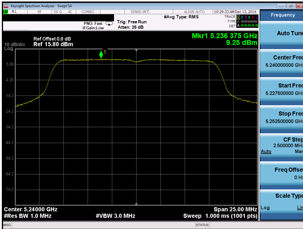
Plot 7-102. Power Spectral Density Plot (802.11a (UNII Band 1) – Ch. 48)
