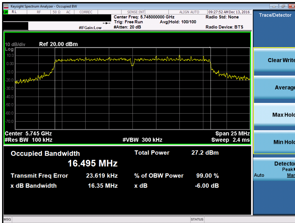
Plot 7-55. 6dB Bandwidth Plot (802.11a (UNII Band 3) – Ch. 149)
