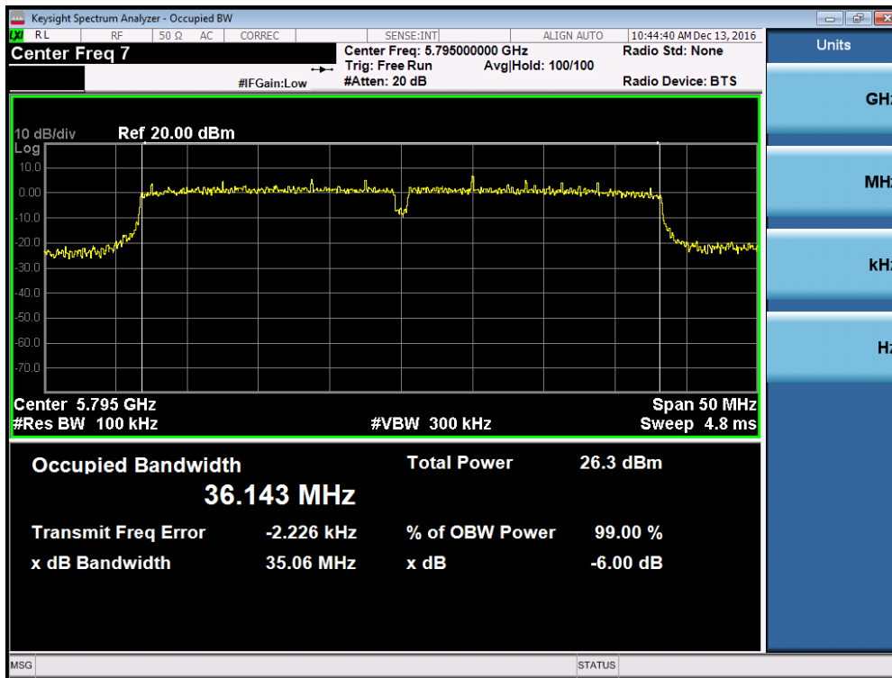
Plot 7-71. 6dB Bandwidth Plot (40MHz BW 802.11n (UNII Band 3) – Ch. 159)
