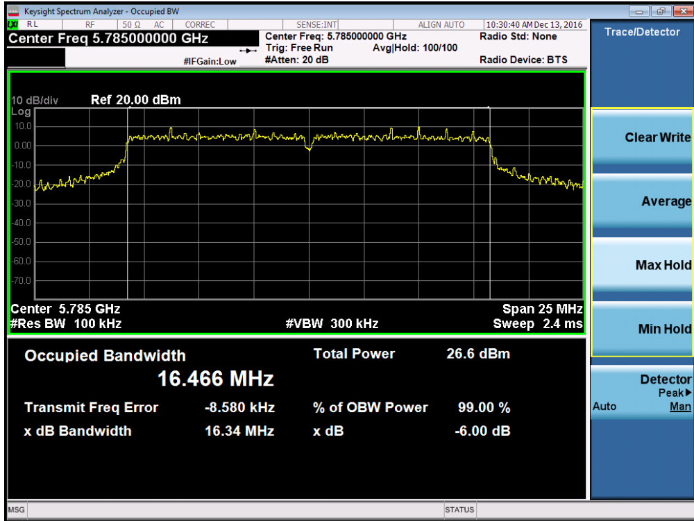
Plot 7-65. 6dB Bandwidth Plot (802.11a (UNII Band 3) – Ch. 157)
