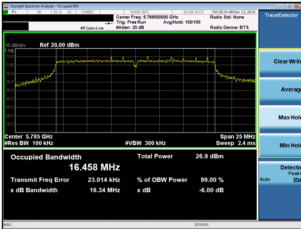
Plot 7-56. 6dB Bandwidth Plot (802.11a (UNII Band 3) – Ch. 157)
