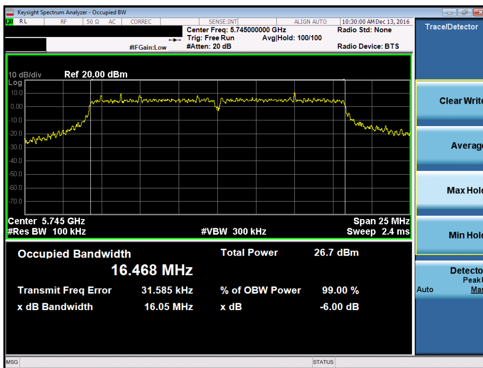
Plot 7-64. 6dB Bandwidth Plot (802.11a (UNII Band 3) – Ch. 149)
