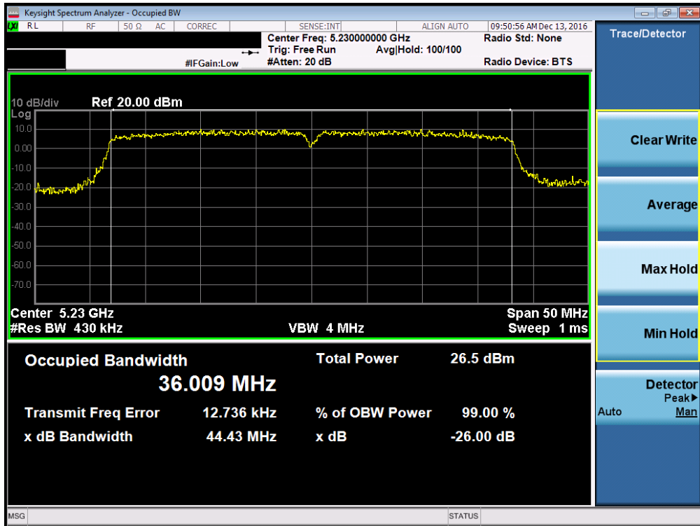
Plot 7-26. 26dB Bandwidth Plot (40MHz BW 802.11n (UNII Band 1) – Ch. 46)
