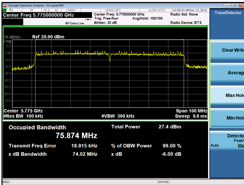
Plot 7-72. 6dB Bandwidth Plot (80MHz BW 802.11ac (UNII Band 3) – Ch. 155)
