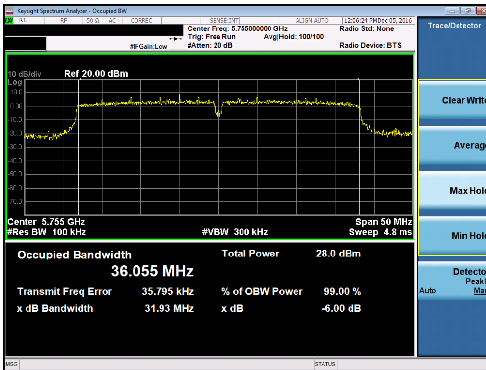
Plot 7-43. 6dB Bandwidth Plot (40MHz BW 802.11n (UNII Band 3) – Ch. 151)
