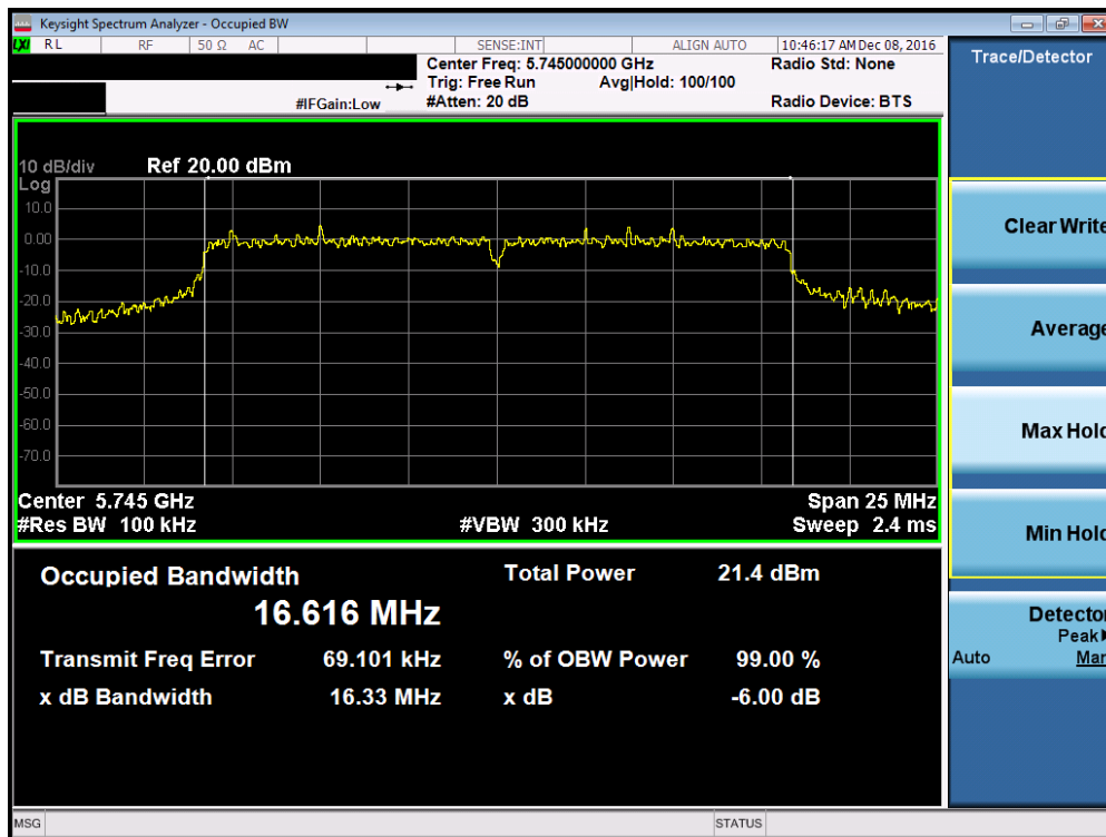
Plot 7-46. 6dB Bandwidth Plot (802.11a (UNII Band 3) – Ch. 149)
