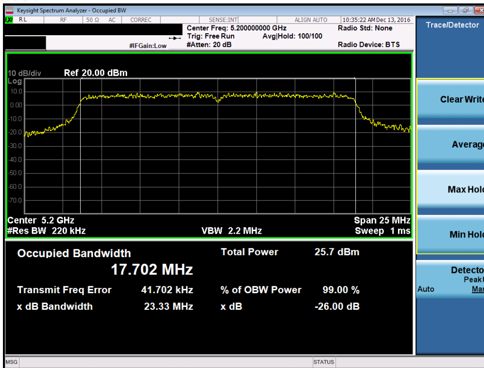
Plot 7-32. 26dB Bandwidth Plot (20MHz BW 802.11n (UNII Band 1) – Ch. 40)
