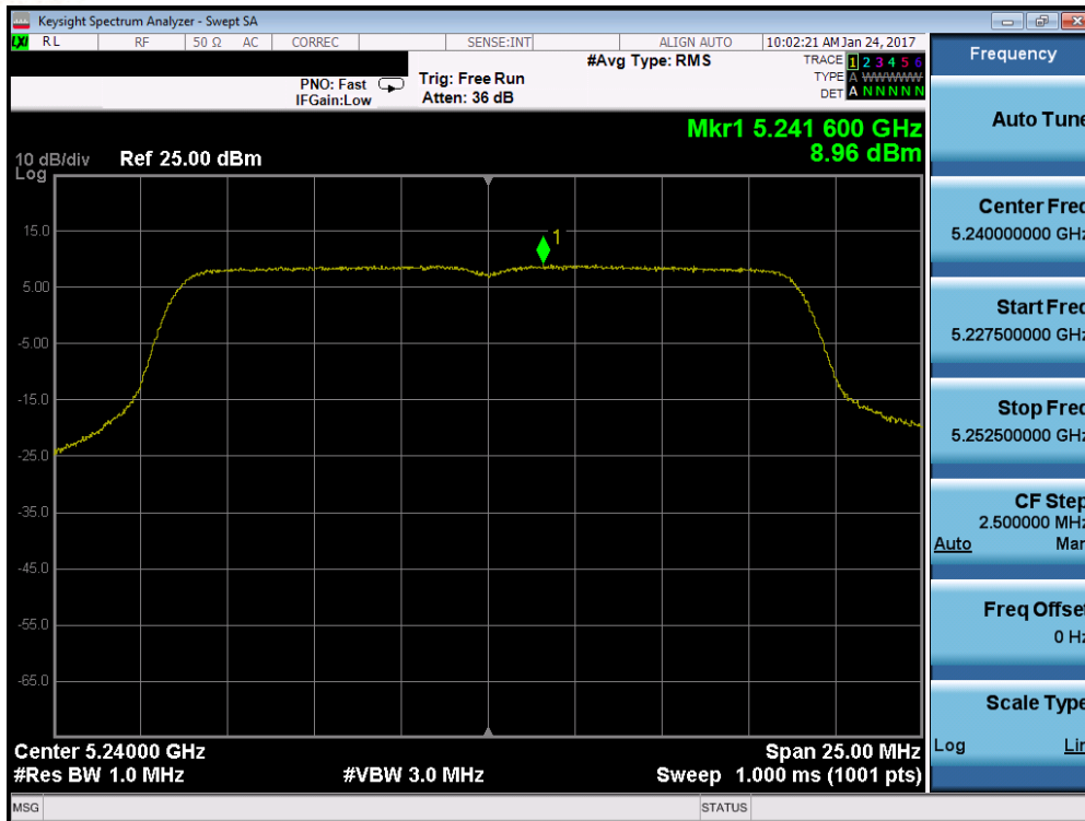
Plot 7-87. Power Spectral Density Plot (20MHz BW 802.11n (UNII Band 1) – Ch. 48)
