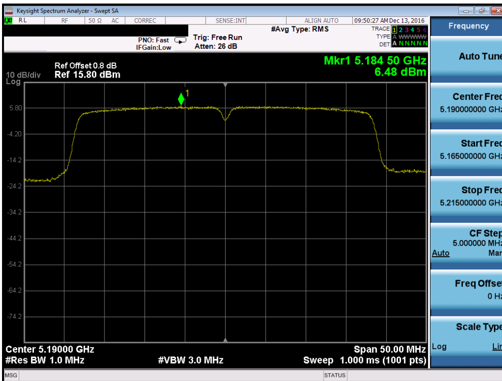
Plot 7-106. Power Spectral Density Plot (40MHz BW 802.11n (UNII Band 1) – Ch. 38)
