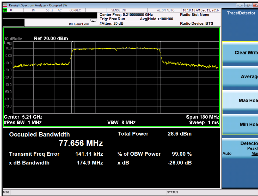
Plot 7-27. 26dB Bandwidth Plot (80MHz BW 802.11ac (UNII Band 1) – Ch. 42)
