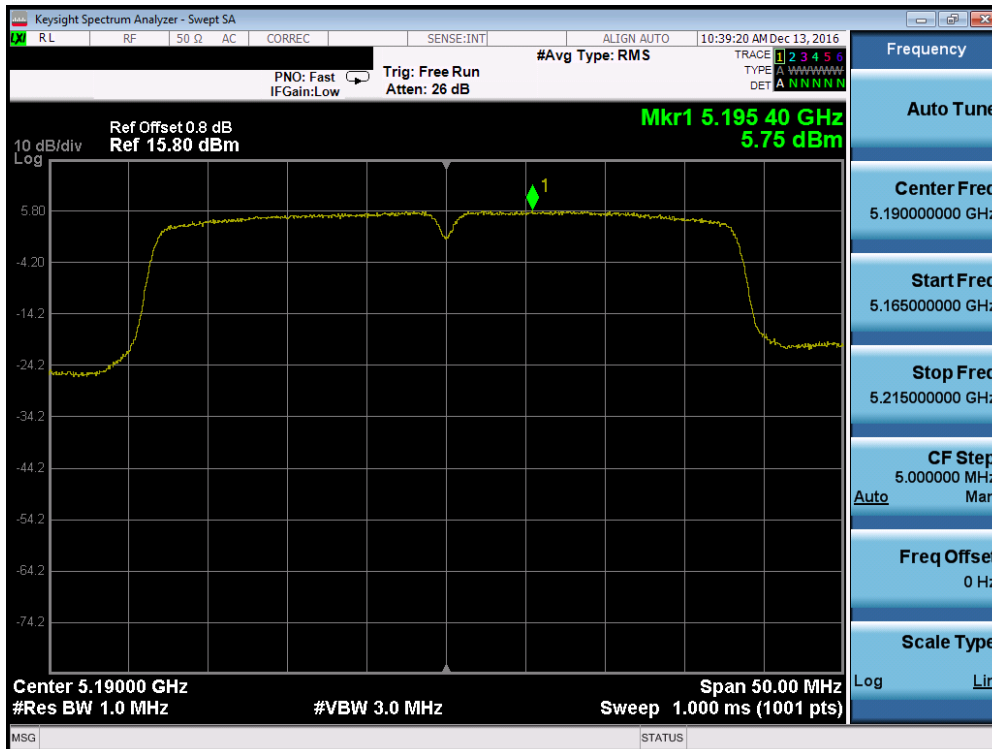
Plot 7-97. Power Spectral Density Plot (40MHz BW 802.11n (UNII Band 1) – Ch. 38)
