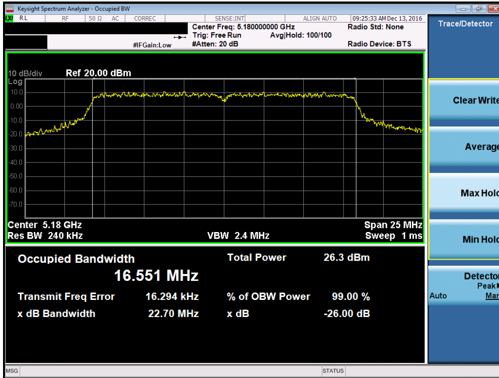
Plot 7-19. 26dB Bandwidth Plot (802.11a (UNII Band 1) – Ch. 36)
