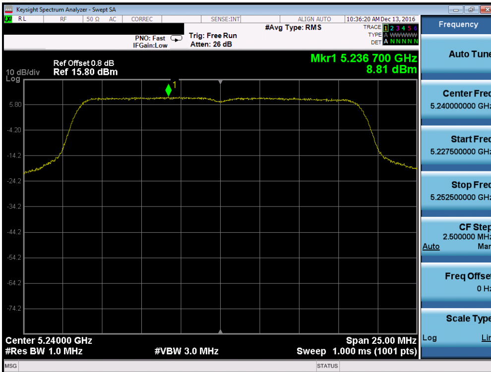
Plot 7-105. Power Spectral Density Plot (20MHz BW 802.11n (UNII Band 1) – Ch. 48)
