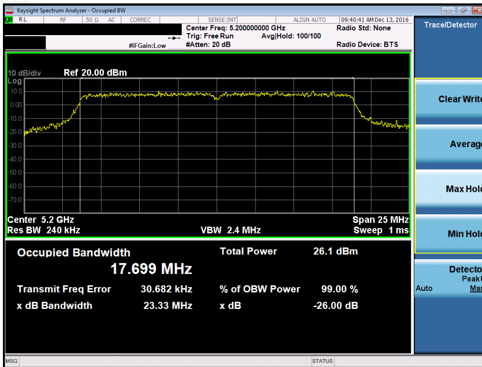
Plot 7-23. 26dB Bandwidth Plot (20MHz BW 802.11n (UNII Band 1) – Ch. 40)
