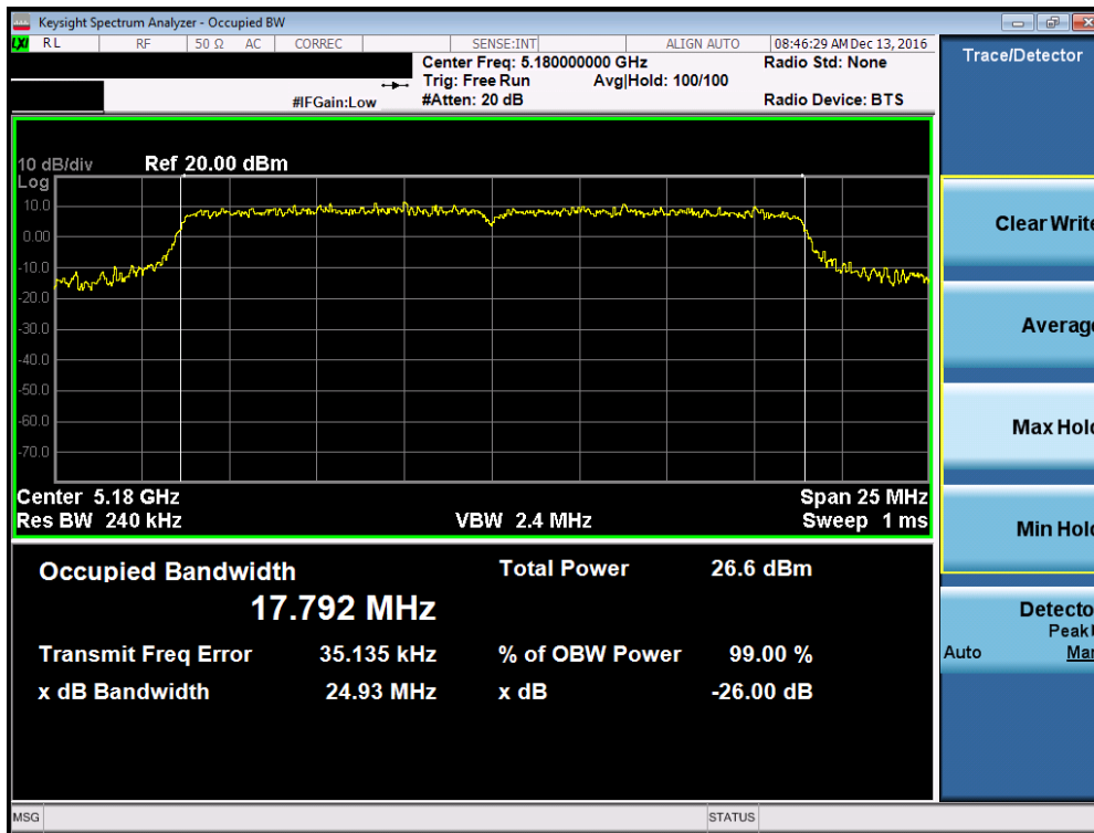
Plot 7-13. 26dB Bandwidth Plot (20MHz BW 802.11n (UNII Band 1) – Ch. 36)
