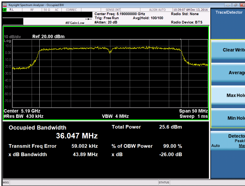
Plot 7-34. 26dB Bandwidth Plot (40MHz BW 802.11n (UNII Band 1) – Ch. 38)
