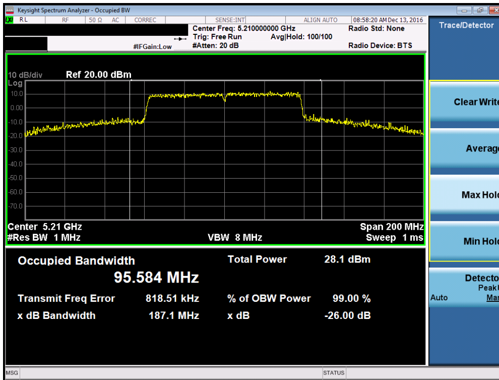
Plot 7-18. 26dB Bandwidth Plot (80MHz BW 802.11ac (UNII Band 1) – Ch. 42)
