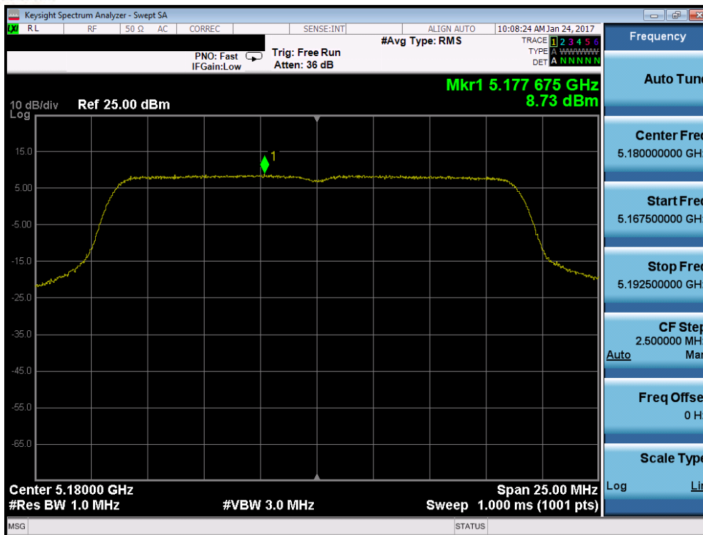
Plot 7-94. Power Spectral Density Plot (20MHz BW 802.11n (UNII Band 1) – Ch. 36)
