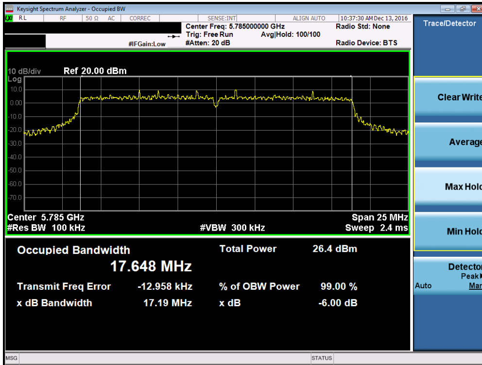
Plot 7-68. 6dB Bandwidth Plot (20MHz BW 802.11n (UNII Band 3) – Ch. 157)
