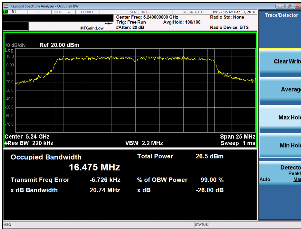
Plot 7-21. 26dB Bandwidth Plot (802.11a (UNII Band 1) – Ch. 48)
