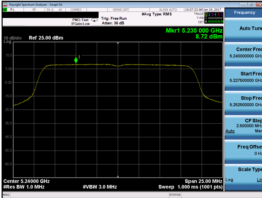
Plot 7-96. Power Spectral Density Plot (20MHz BW 802.11n (UNII Band 1) – Ch. 48)
