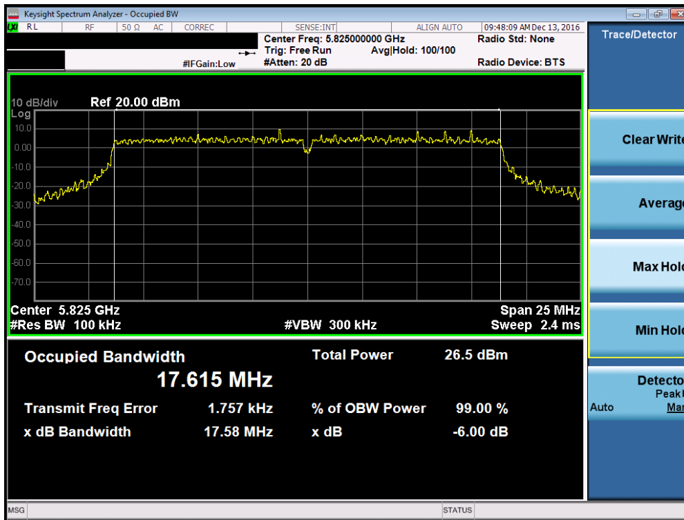
Plot 7-60. 6dB Bandwidth Plot (20MHz BW 802.11n (UNII Band 3) – Ch. 165)
