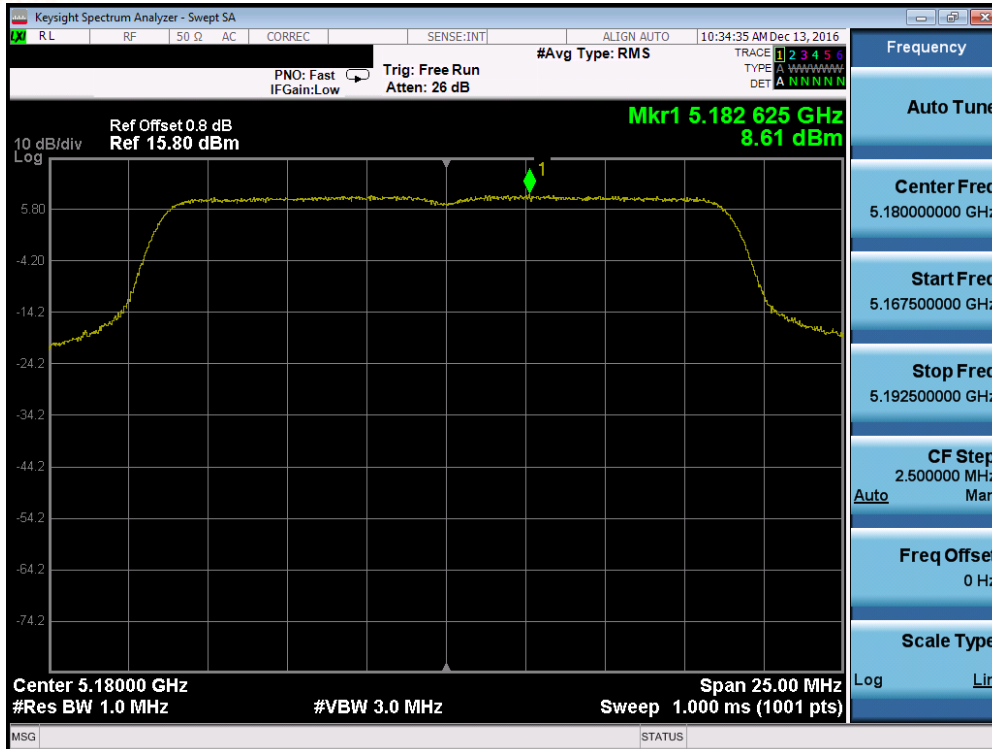
Plot 7-103. Power Spectral Density Plot (20MHz BW 802.11n (UNII Band 1) – Ch. 36)
