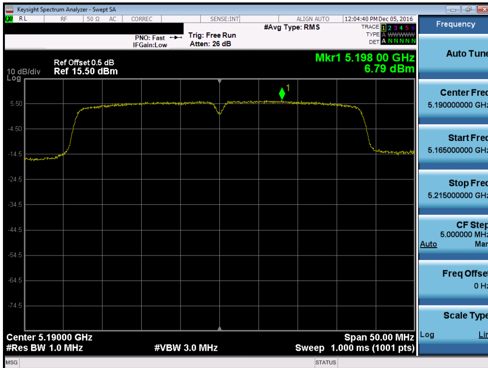
Plot 7-79. Power Spectral Density Plot (40MHz BW 802.11n (UNII Band 1) – Ch. 38)
