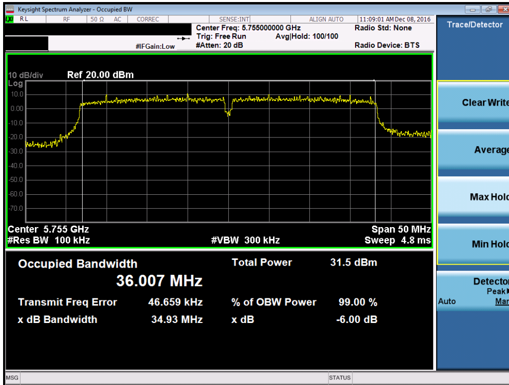
Plot 7-52. 6dB Bandwidth Plot (40MHz BW 802.11n (UNII Band 3) – Ch. 151)
