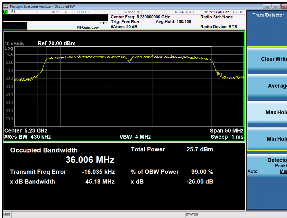
Plot 7-35. 26dB Bandwidth Plot (40MHz BW 802.11n (UNII Band 1) – Ch. 46)
