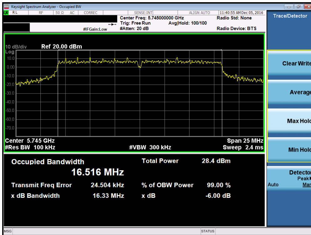
Plot 7-37. 6dB Bandwidth Plot (802.11a (UNII Band 3) – Ch. 149)
