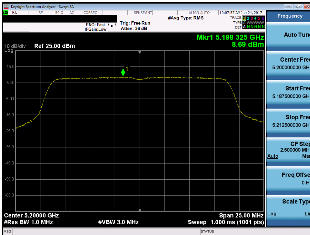
Plot 7-95. Power Spectral Density Plot (20MHz BW 802.11n (UNII Band 1) – Ch. 40)
