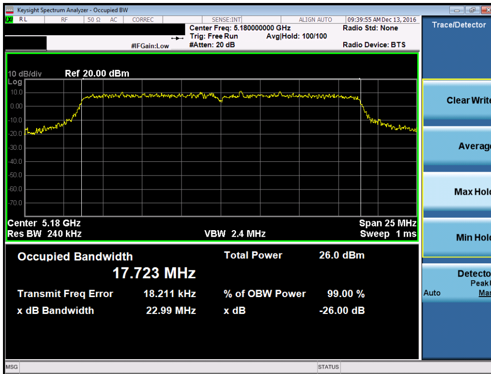
Plot 7-22. 26dB Bandwidth Plot (20MHz BW 802.11n (UNII Band 1) – Ch. 36)
