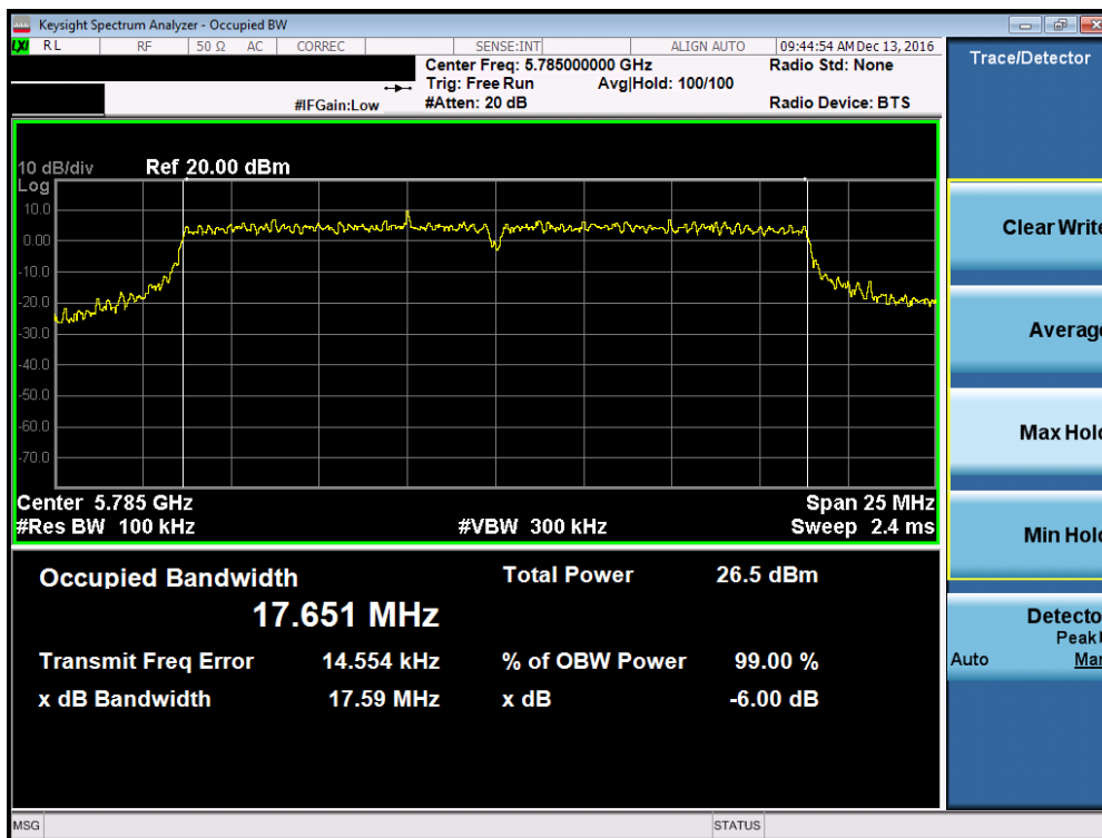
Plot 7-59. 6dB Bandwidth Plot (20MHz BW 802.11n (UNII Band 3) – Ch. 157)
