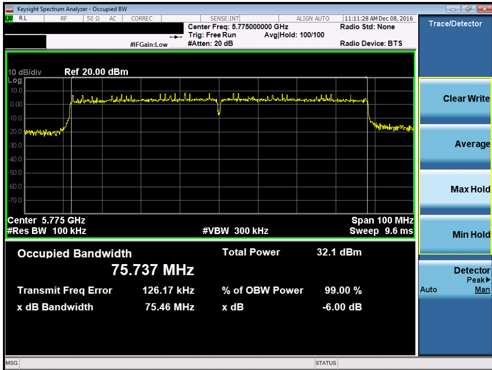
Plot 7-54. 6dB Bandwidth Plot (80MHz BW 802.11ac (UNII Band 3) – Ch. 155)
