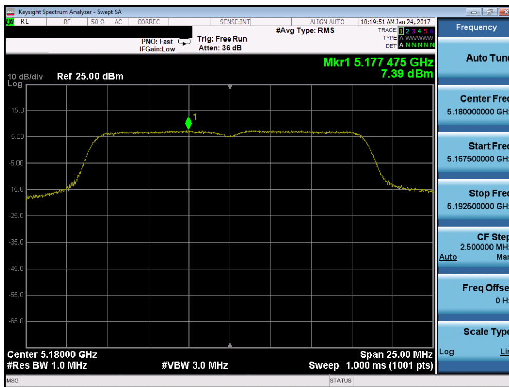
Plot 7-100. Power Spectral Density Plot (802.11a (UNII Band 1) – Ch. 36)
