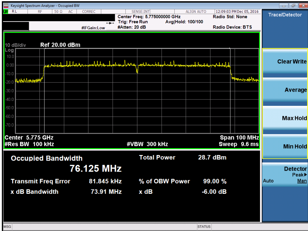
Plot 7-45. 6dB Bandwidth Plot (80MHz BW 802.11ac (UNII Band 3) – Ch. 155)
