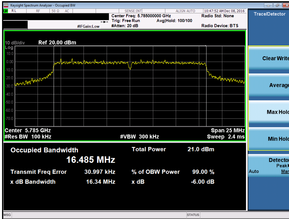
Plot 7-47. 6dB Bandwidth Plot (802.11a (UNII Band 3) – Ch. 157)
