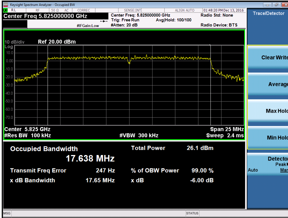
Plot 7-51. 6dB Bandwidth Plot (20MHz BW 802.11n (UNII Band 3) – Ch. 165)
