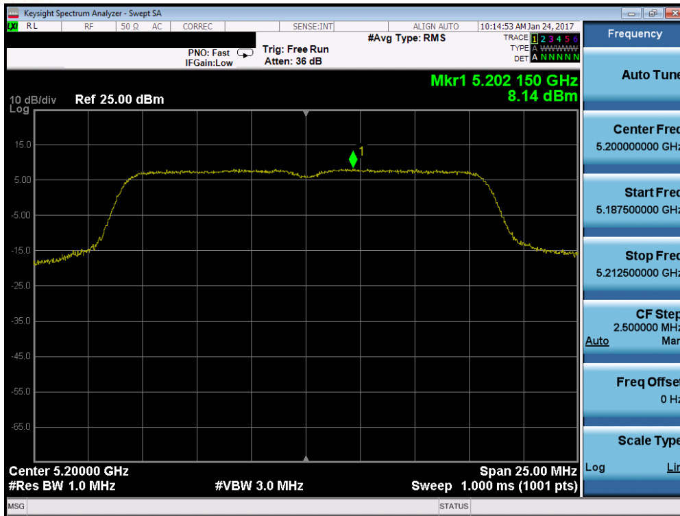
Plot 7-92. Power Spectral Density Plot (802.11a (UNII Band 1) – Ch. 40)
