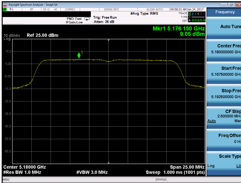
Plot 7-82. Power Spectral Density Plot (802.11a (UNII Band 1) – Ch. 36)
