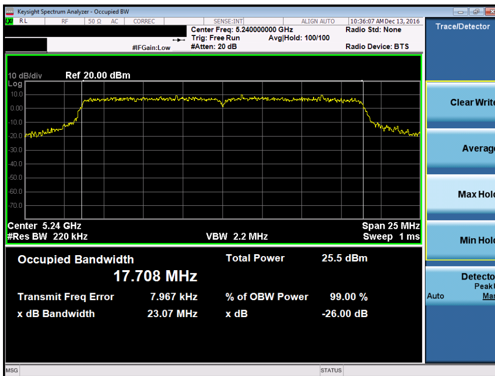
Plot 7-33. 26dB Bandwidth Plot (20MHz BW 802.11n (UNII Band 1) – Ch. 48)
