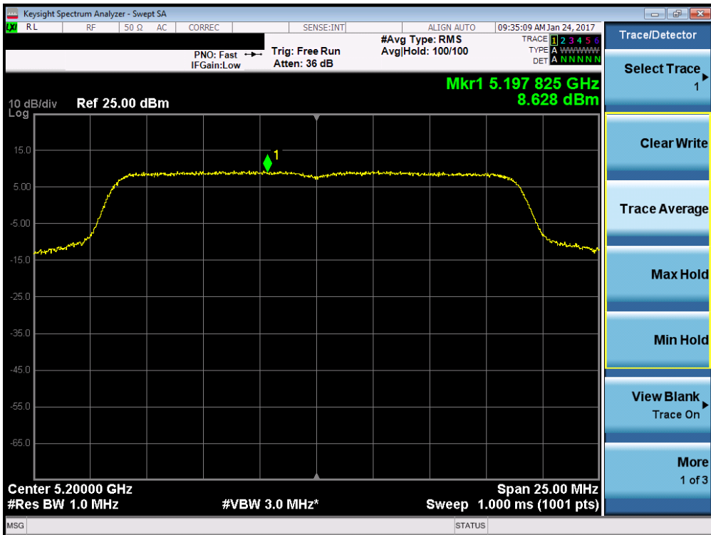
Plot 7-77. Power Spectral Density Plot (20MHz BW 802.11n (UNII Band 1) – Ch. 40)
