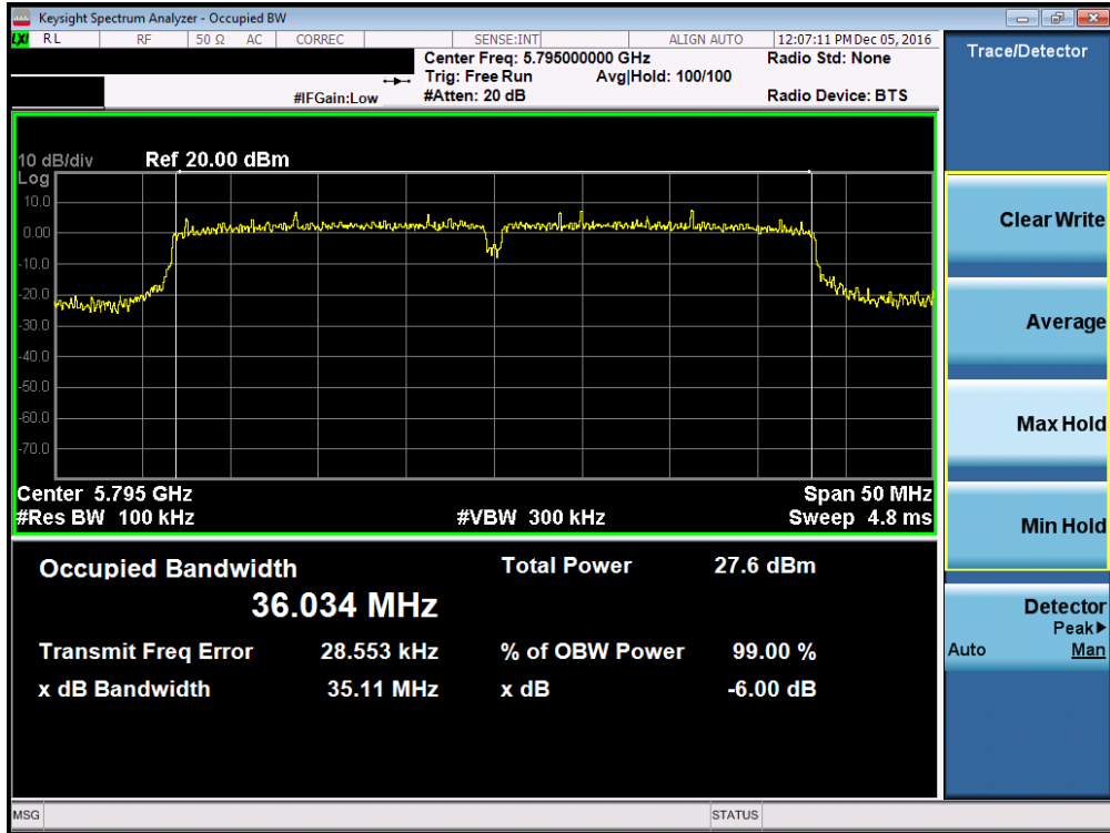
Plot 7-44. 6dB Bandwidth Plot (40MHz BW 802.11n (UNII Band 3) – Ch. 159)
