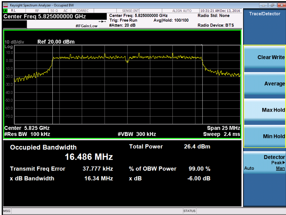
Plot 7-66. 6dB Bandwidth Plot (802.11a (UNII Band 3) – Ch. 165)
