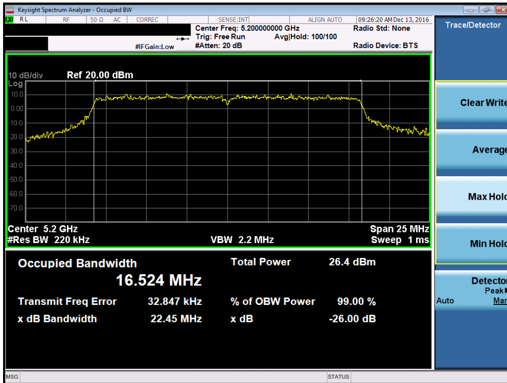
Plot 7-20. 26dB Bandwidth Plot (802.11a (UNII Band 1) – Ch. 40)
