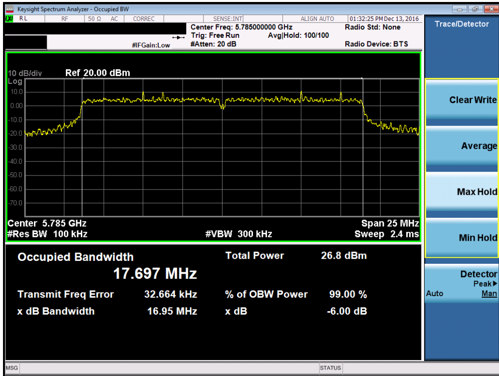
Plot 7-41. 6dB Bandwidth Plot (20MHz BW 802.11n (UNII Band 3) – Ch. 157)
