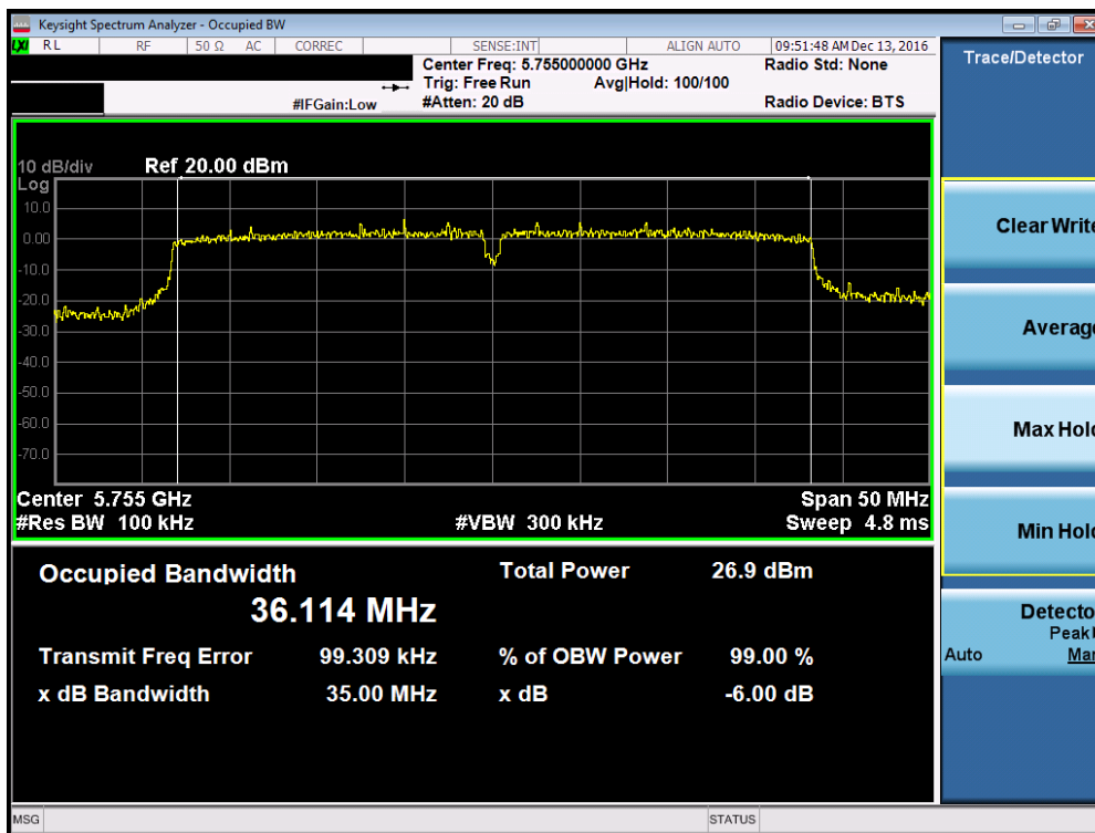
Plot 7-61. 6dB Bandwidth Plot (40MHz BW 802.11n (UNII Band 3) – Ch. 151)
