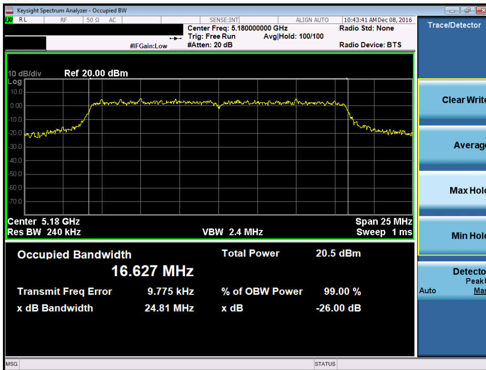
Plot 7-10. 26dB Bandwidth Plot (802.11a (UNII Band 1) – Ch. 36)
