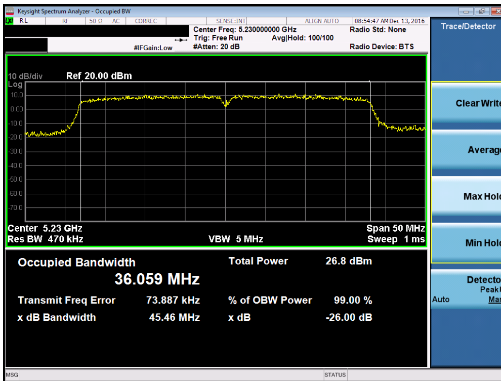
Plot 7-17. 26dB Bandwidth Plot (40MHz BW 802.11n (UNII Band 1) – Ch. 46)
