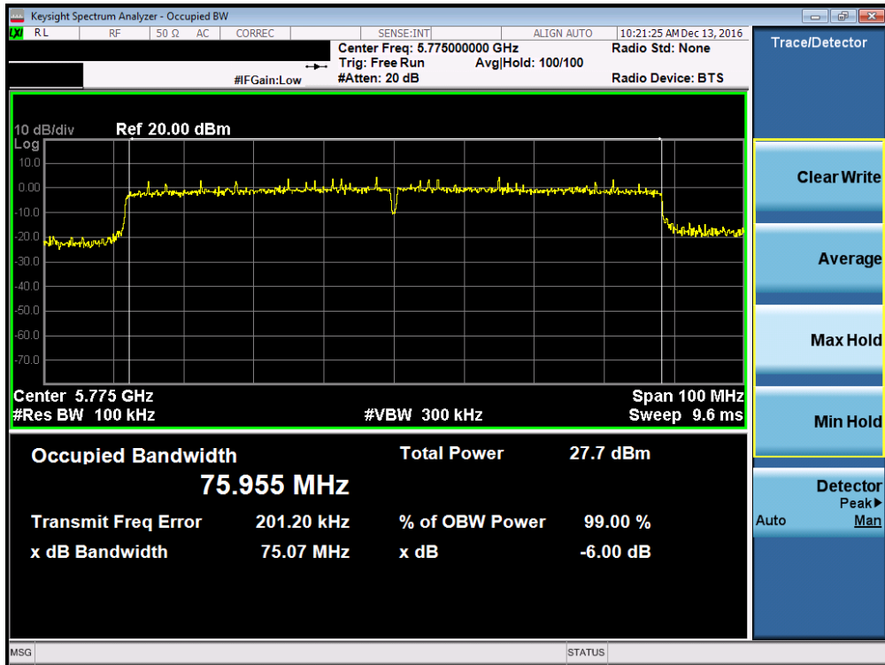
Plot 7-63. 6dB Bandwidth Plot (80MHz BW 802.11ac (UNII Band 3) – Ch. 155)
