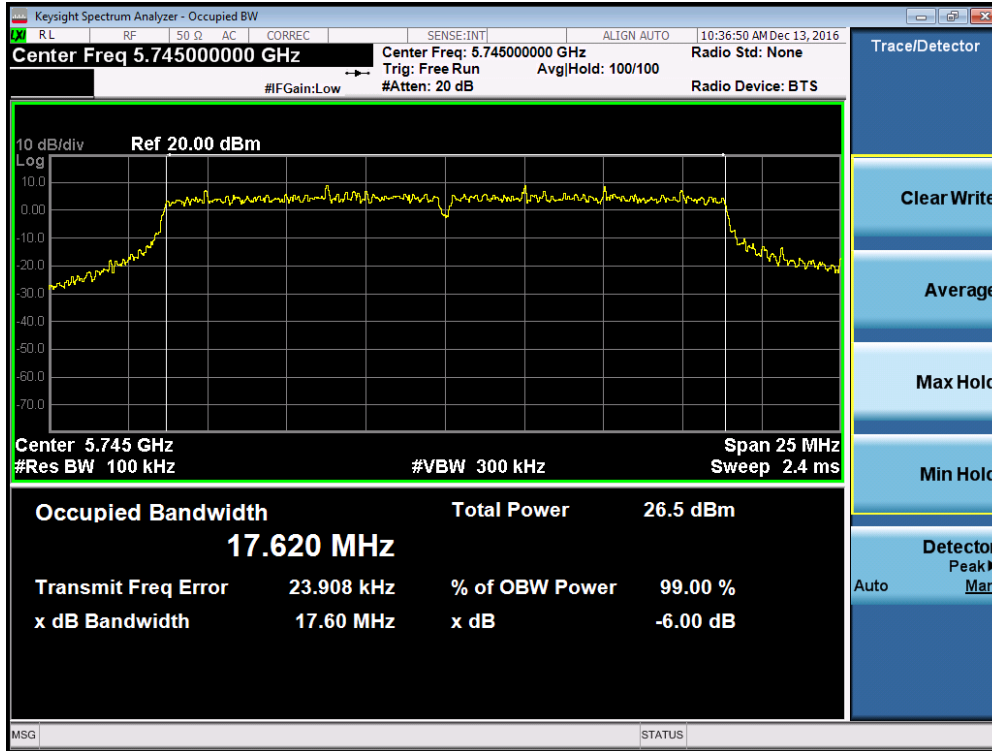
Plot 7-67. 6dB Bandwidth Plot (20MHz BW 802.11n (UNII Band 3) – Ch. 149)
