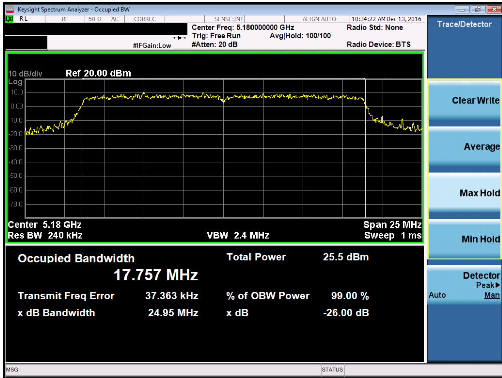
Plot 7-31. 26dB Bandwidth Plot (20MHz BW 802.11n (UNII Band 1) – Ch. 36)
