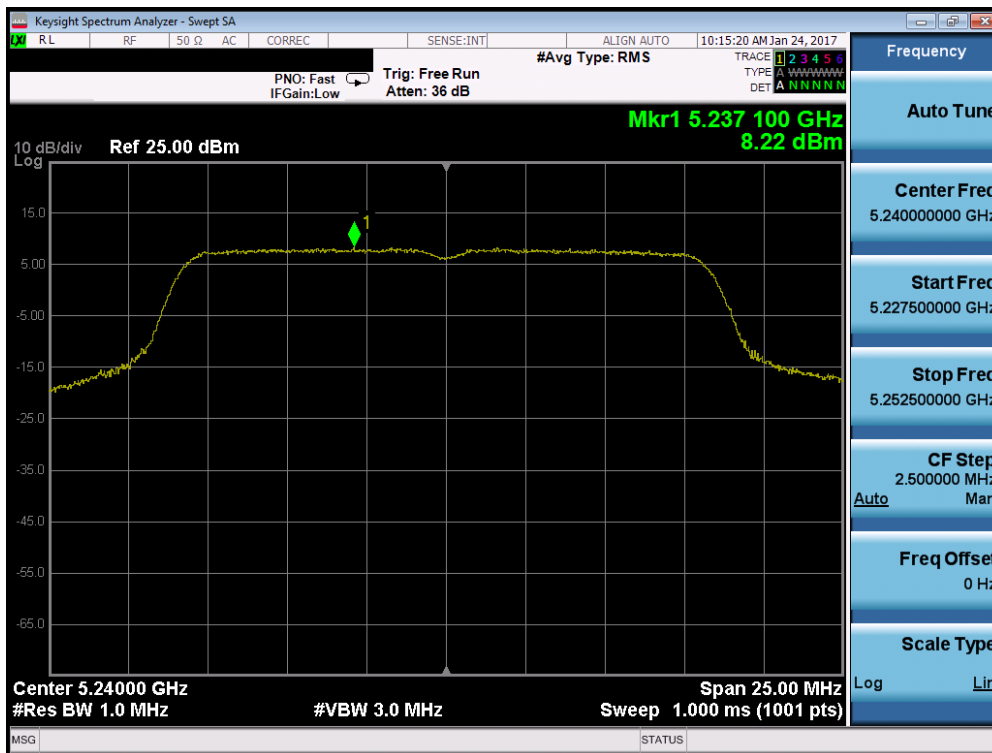
Plot 7-93. Power Spectral Density Plot (802.11a (UNII Band 1) – Ch. 48)
