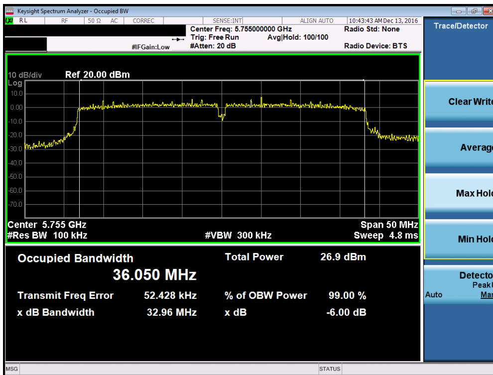
Plot 7-70. 6dB Bandwidth Plot (40MHz BW 802.11n (UNII Band 3) – Ch. 151)
