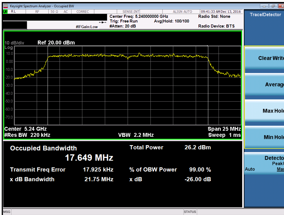
Plot 7-24. 26dB Bandwidth Plot (20MHz BW 802.11n (UNII Band 1) – Ch. 48)
