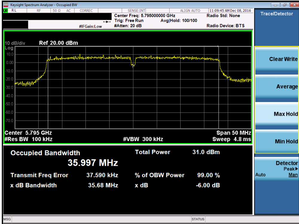
Plot 7-53. 6dB Bandwidth Plot (40MHz BW 802.11n (UNII Band 3) – Ch. 159)
