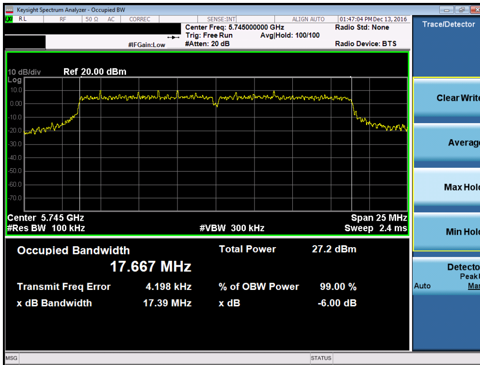
Plot 7-49. 6dB Bandwidth Plot (20MHz BW 802.11n (UNII Band 3) – Ch. 149)
