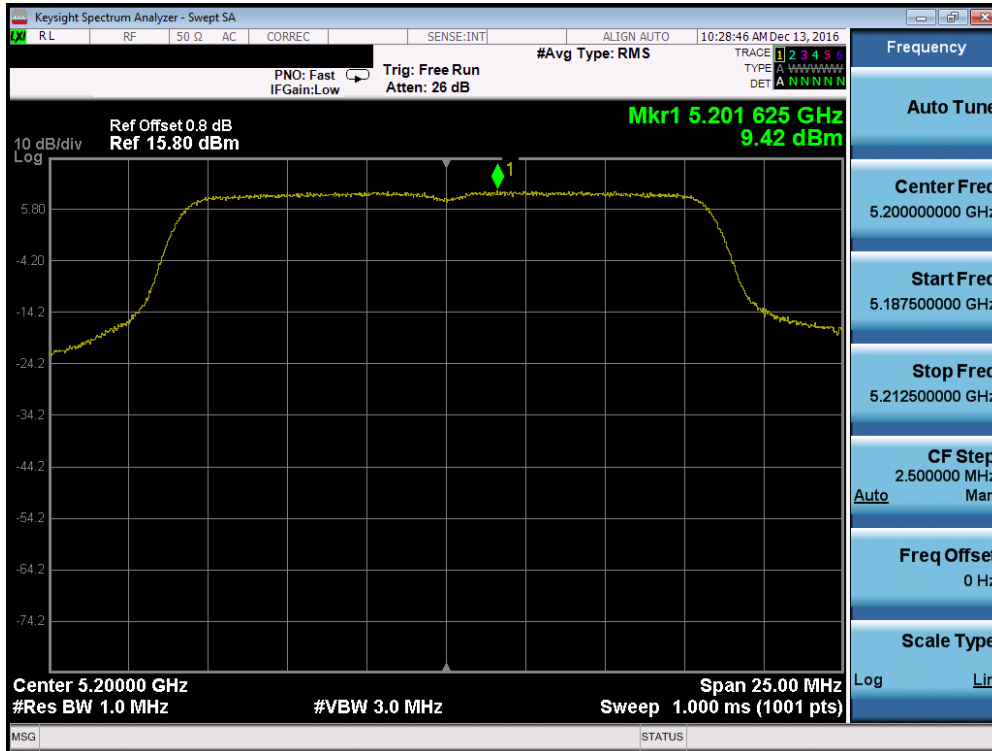
Plot 7-101. Power Spectral Density Plot (802.11a (UNII Band 1) – Ch. 40)
