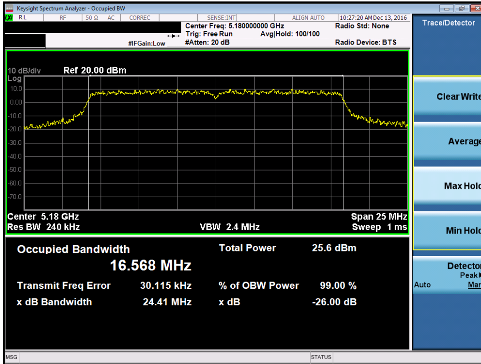
Plot 7-28. 26dB Bandwidth Plot (802.11a (UNII Band 1) – Ch. 36)
