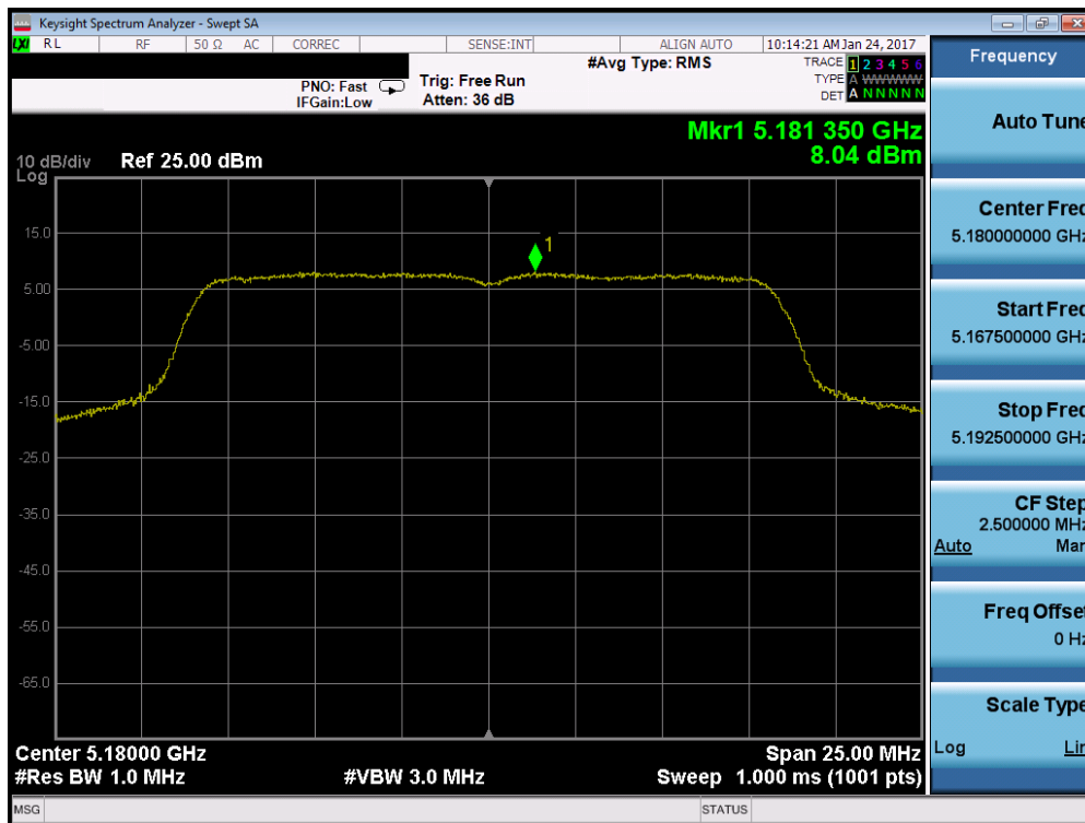
Plot 7-91. Power Spectral Density Plot (802.11a (UNII Band 1) – Ch. 36)
