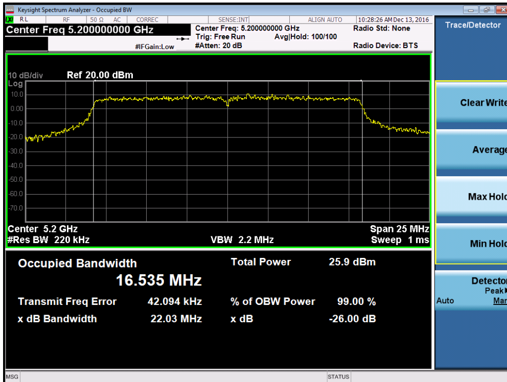
Plot 7-29. 26dB Bandwidth Plot (802.11a (UNII Band 1) – Ch. 40)
