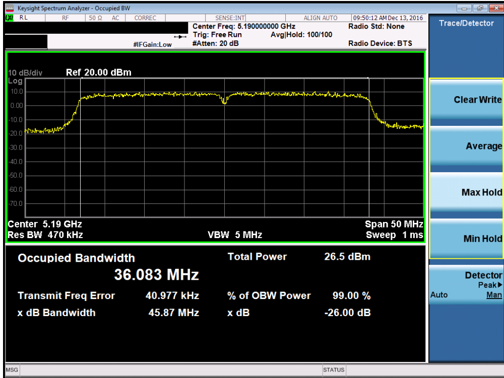
Plot 7-25. 26dB Bandwidth Plot (40MHz BW 802.11n (UNII Band 1) – Ch. 38)
