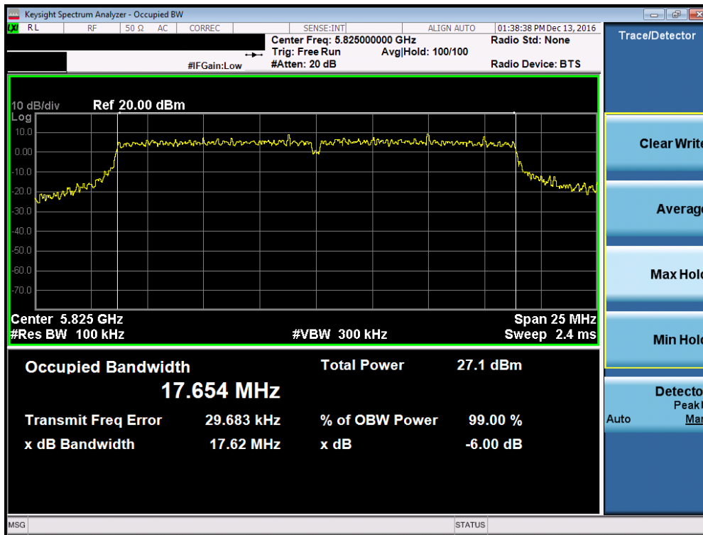
Plot 7-42. 6dB Bandwidth Plot (20MHz BW 802.11n (UNII Band 3) – Ch. 165)
