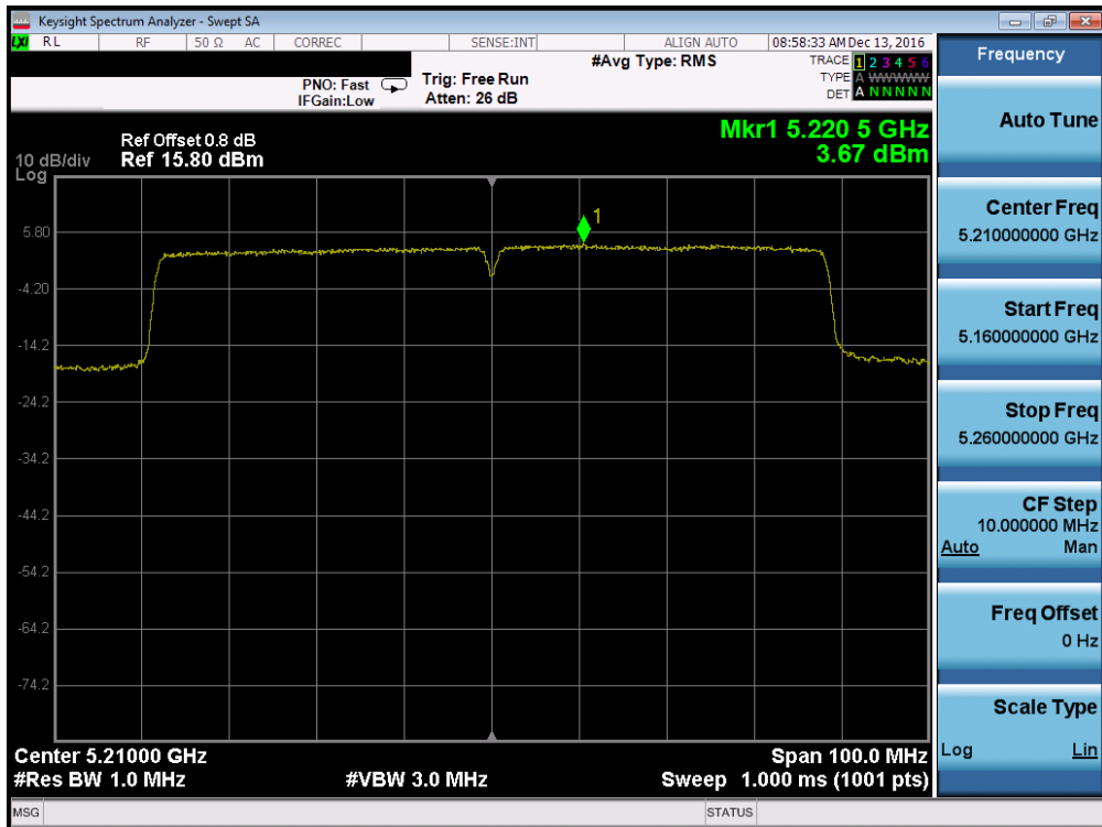
Plot 7-90. Power Spectral Density Plot (80MHz BW 802.11ac (UNII Band 1) – Ch. 42)
