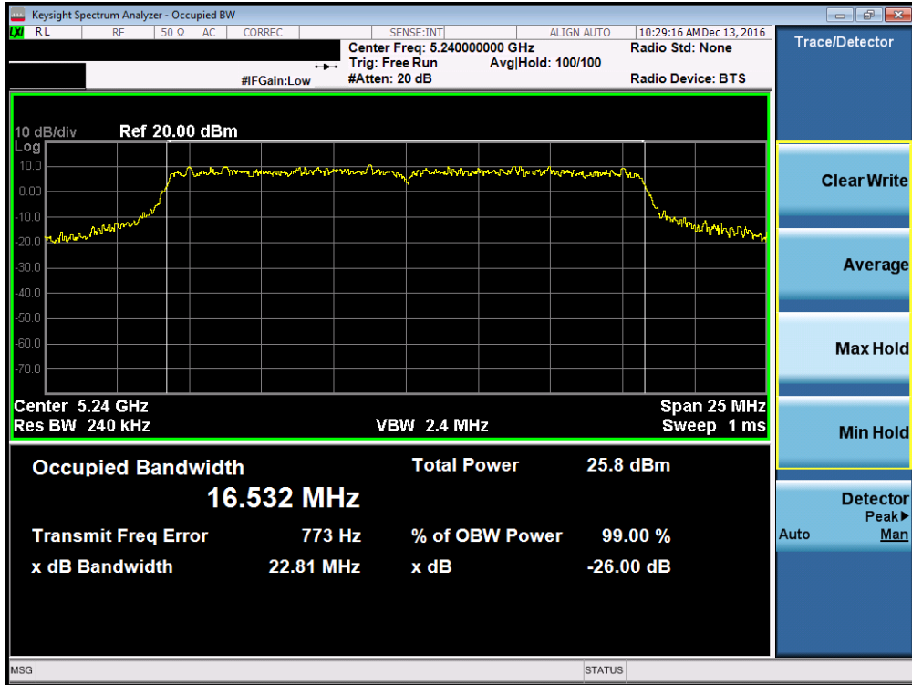
Plot 7-30. 26dB Bandwidth Plot (802.11a (UNII Band 1) – Ch. 48)
