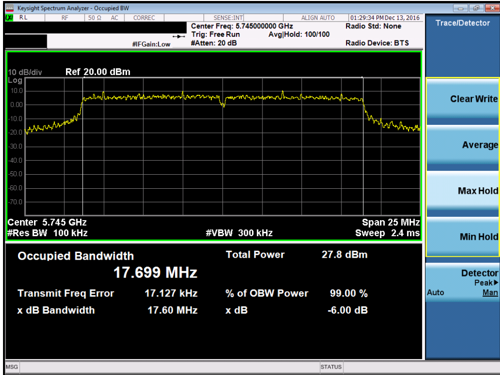
Plot 7-40. 6dB Bandwidth Plot (20MHz BW 802.11n (UNII Band 3) – Ch. 149)
