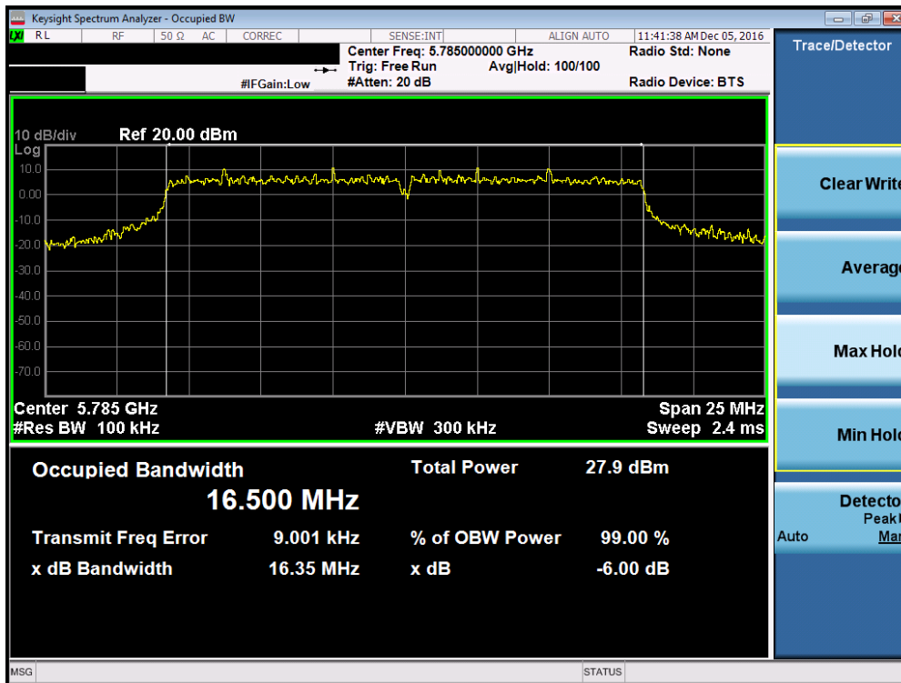
Plot 7-38. 6dB Bandwidth Plot (802.11a (UNII Band 3) – Ch. 157)
