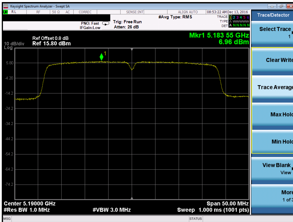
Plot 7-88. Power Spectral Density Plot (40MHz BW 802.11n (UNII Band 1) – Ch. 38)
