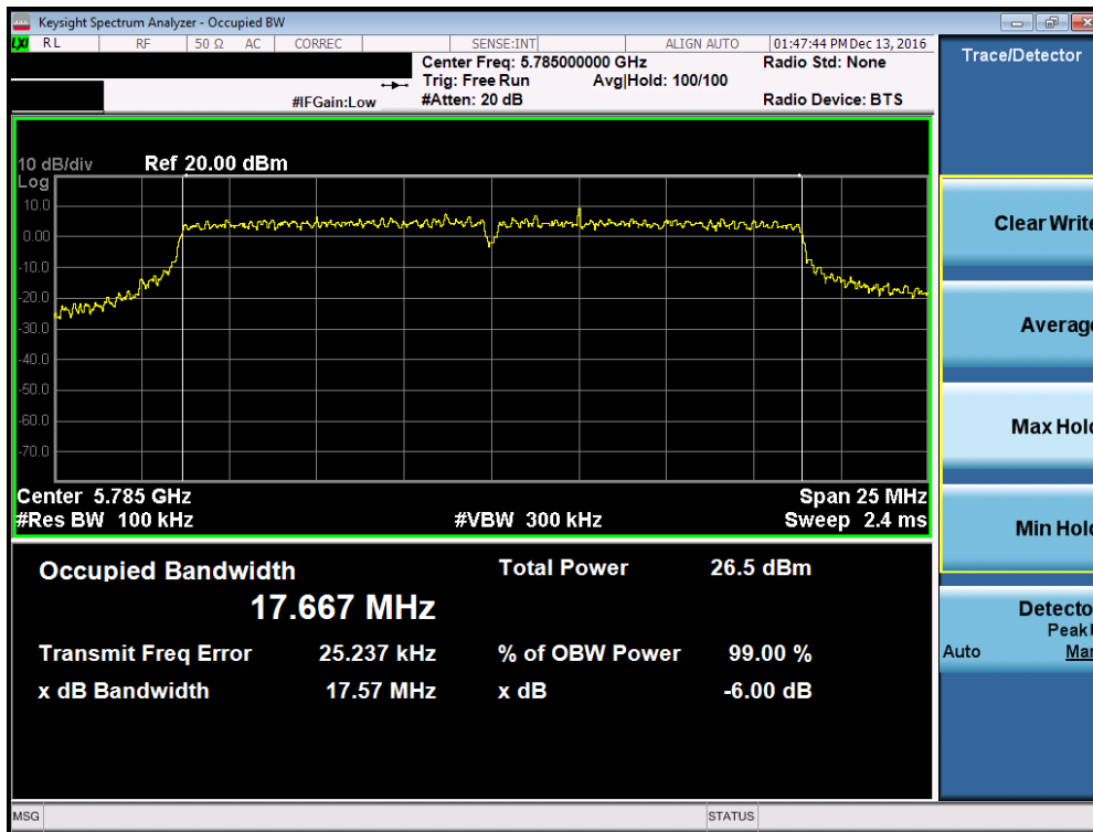
Plot 7-50. 6dB Bandwidth Plot (20MHz BW 802.11n (UNII Band 3) – Ch. 157)
