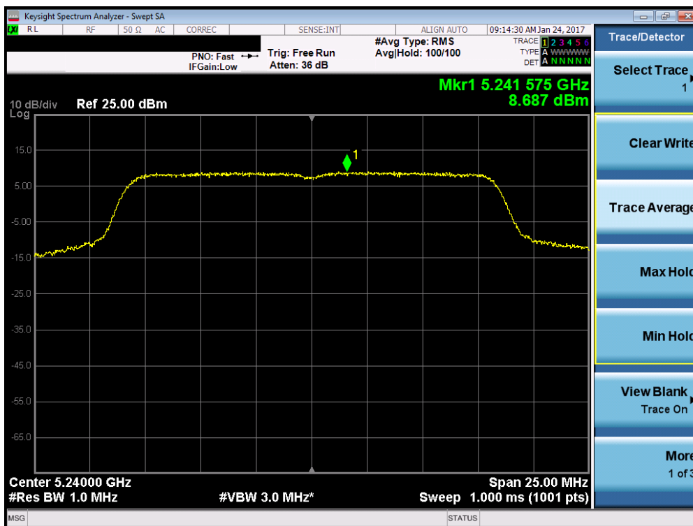
Plot 7-75. Power Spectral Density Plot (802.11a (UNII Band 1) – Ch. 48)
