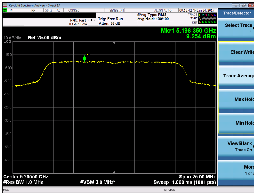
Plot 7-74. Power Spectral Density Plot (802.11a (UNII Band 1) – Ch. 40)
