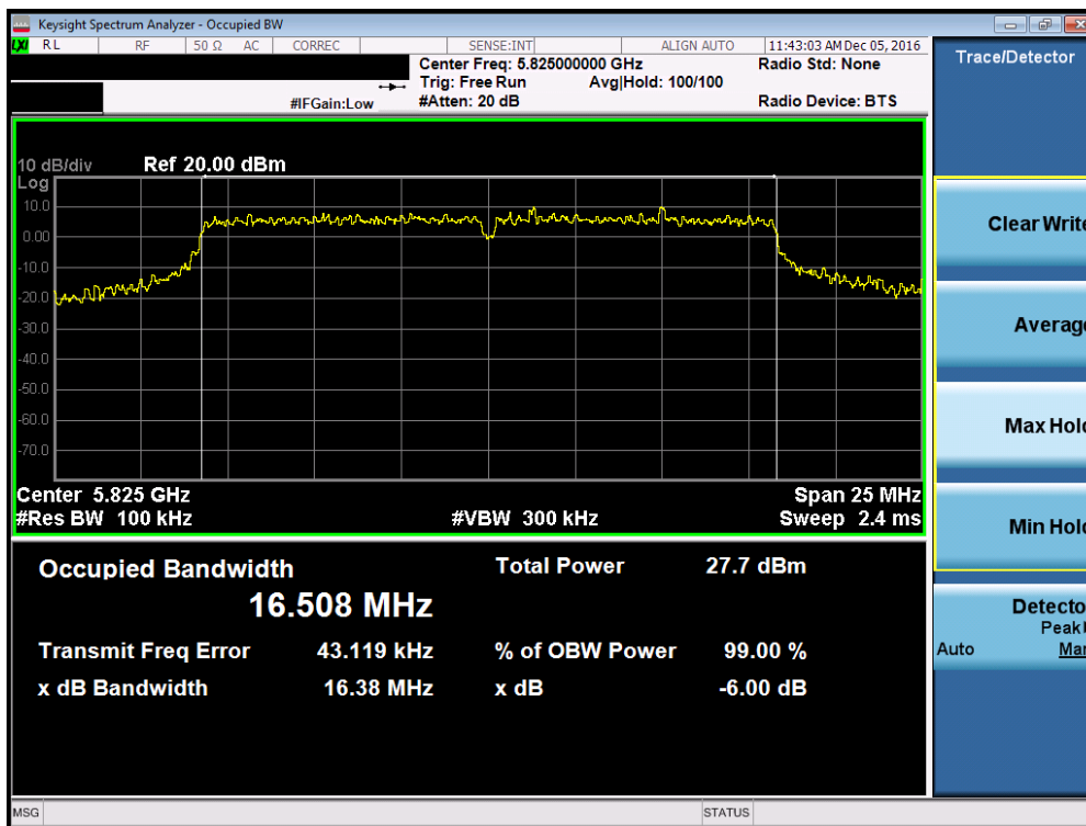
Plot 7-39. 6dB Bandwidth Plot (802.11a (UNII Band 3) – Ch. 165)
