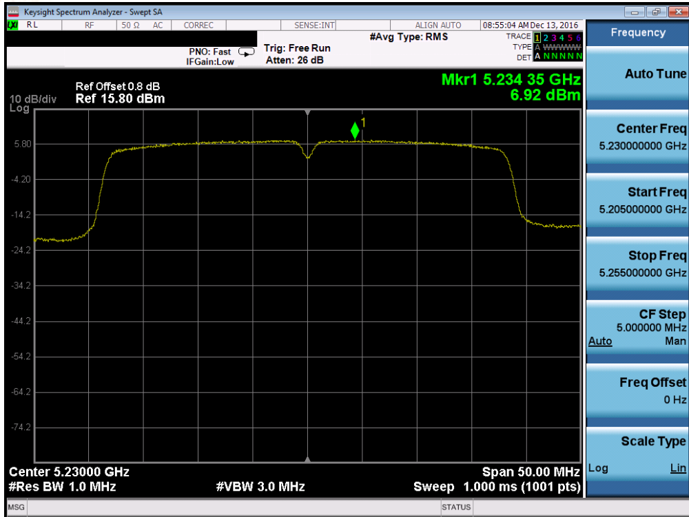
Plot 7-89. Power Spectral Density Plot (40MHz BW 802.11n (UNII Band 1) – Ch. 46)
