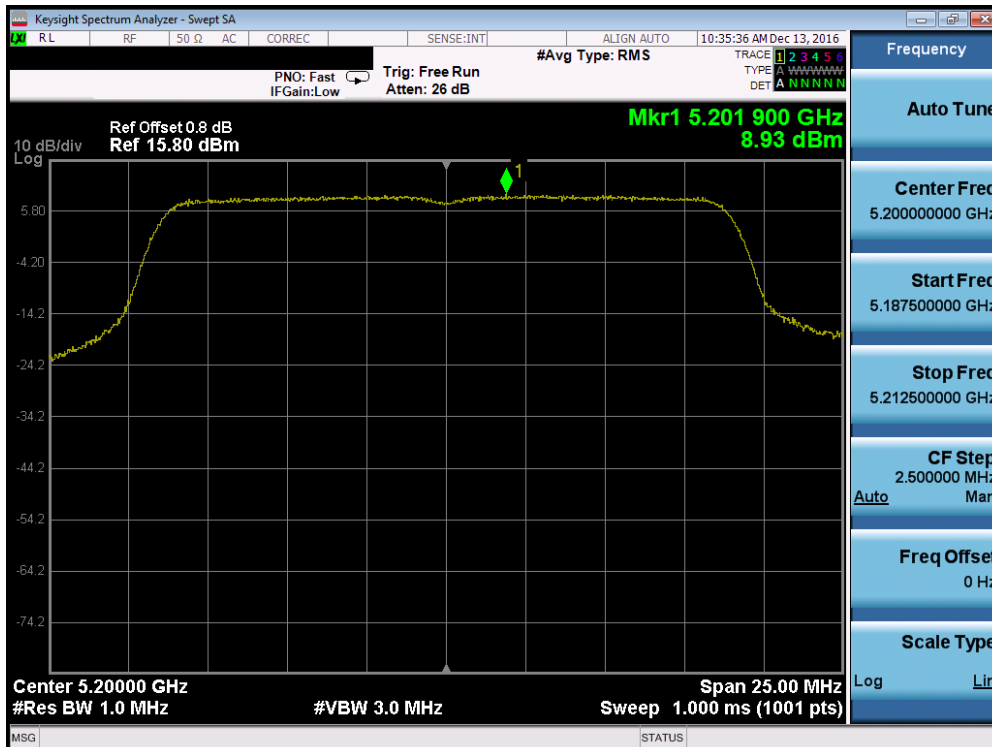
Plot 7-104. Power Spectral Density Plot (20MHz BW 802.11n (UNII Band 1) – Ch. 40)
