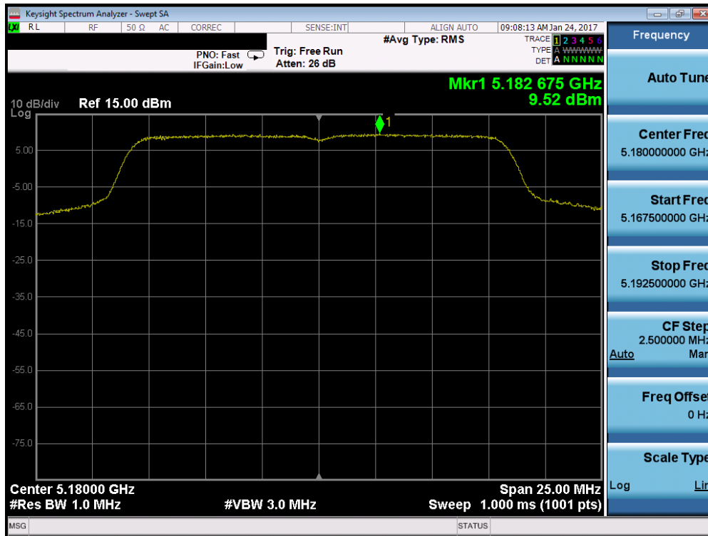
Plot 7-73. Power Spectral Density Plot (802.11a (UNII Band 1) – Ch. 36)
