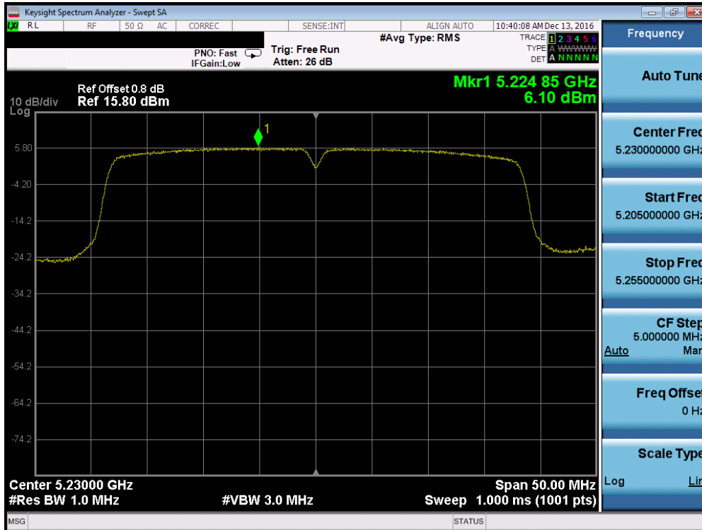
Plot 7-98. Power Spectral Density Plot (40MHz BW 802.11n (UNII Band 1) – Ch. 46)
