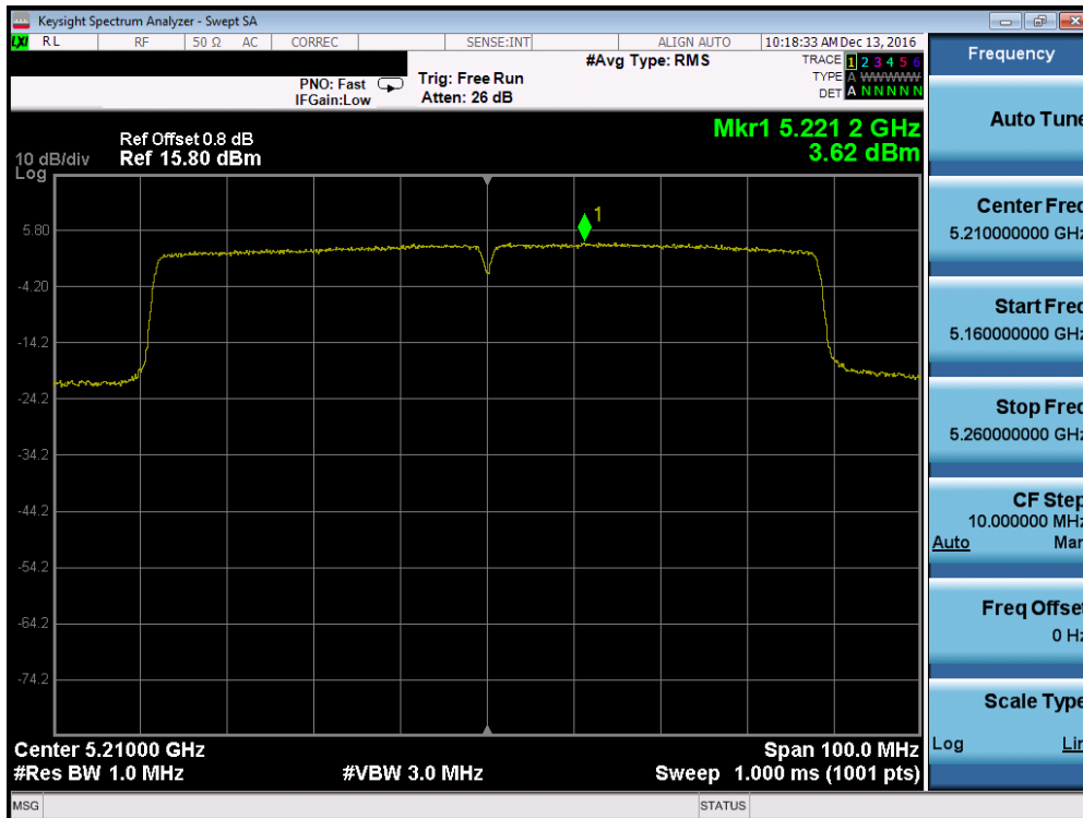
Plot 7-99. Power Spectral Density Plot (80MHz BW 802.11ac (UNII Band 1) – Ch. 42)
