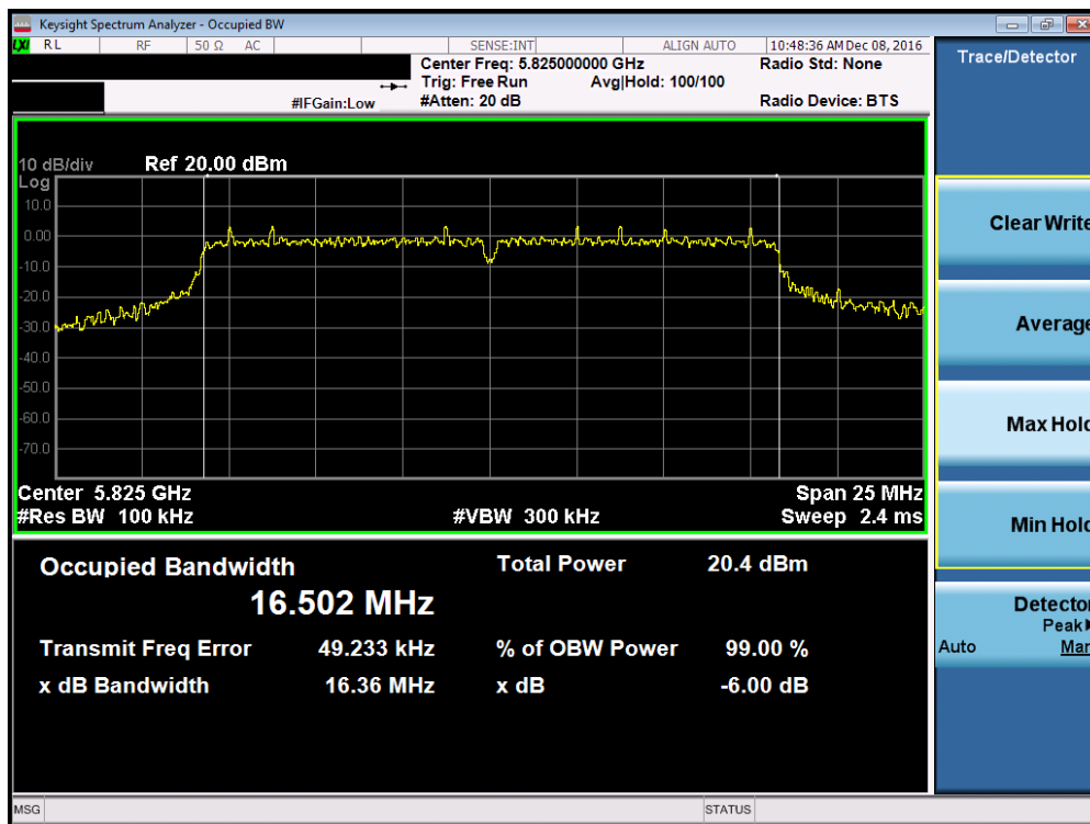
Plot 7-48. 6dB Bandwidth Plot (802.11a (UNII Band 3) – Ch. 165)
