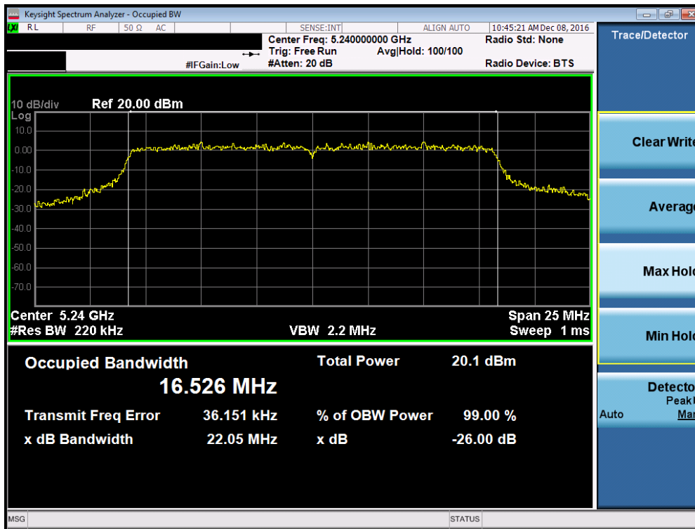
Plot 7-12. 26dB Bandwidth Plot (802.11a (UNII Band 1) – Ch. 48)
