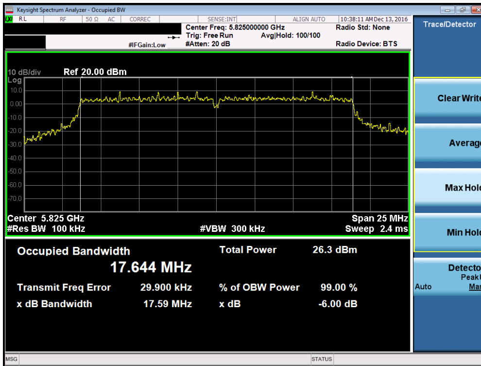
Plot 7-69. 6dB Bandwidth Plot (20MHz BW 802.11n (UNII Band 3) – Ch. 165)
