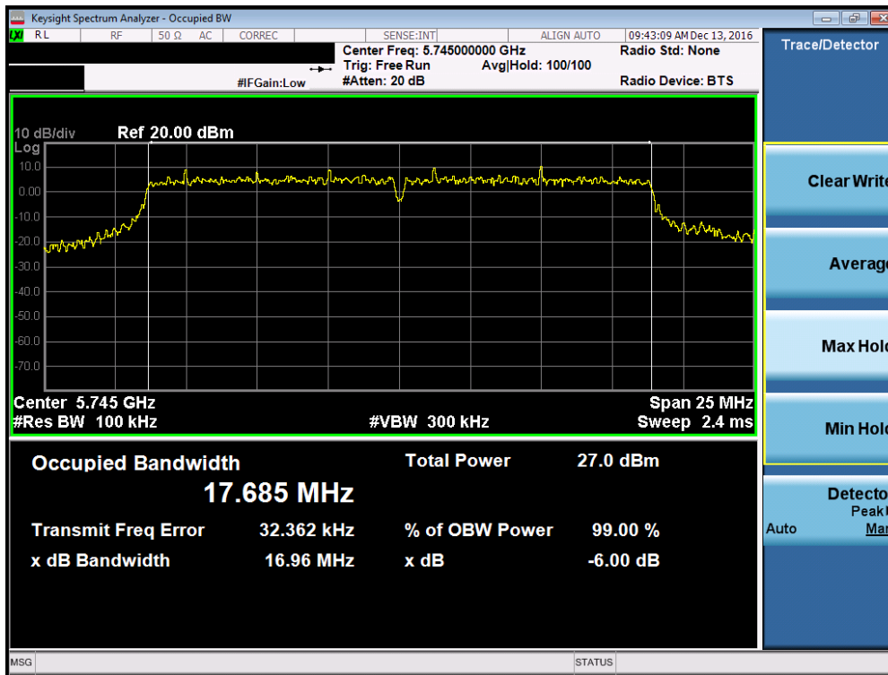
Plot 7-58. 6dB Bandwidth Plot (20MHz BW 802.11n (UNII Band 3) – Ch. 149)
