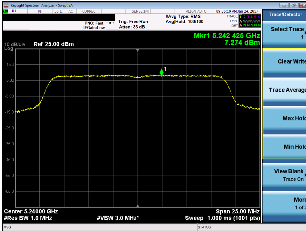
Plot 7-78. Power Spectral Density Plot (20MHz BW 802.11n (UNII Band 1) – Ch. 48)
