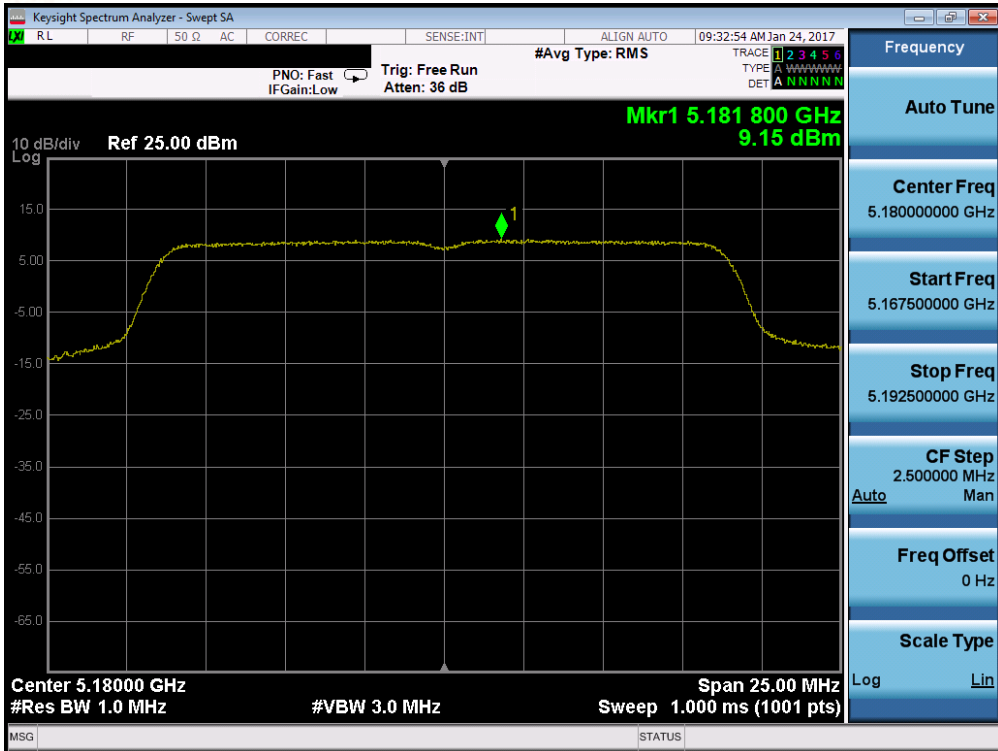
Plot 7-76. Power Spectral Density Plot (20MHz BW 802.11n (UNII Band 1) – Ch. 36)
