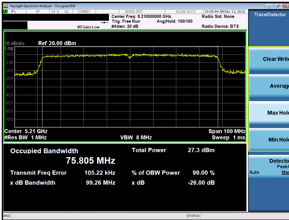
Plot 7-36. 26dB Bandwidth Plot (80MHz BW 802.11ac (UNII Band 1) – Ch. 42)
