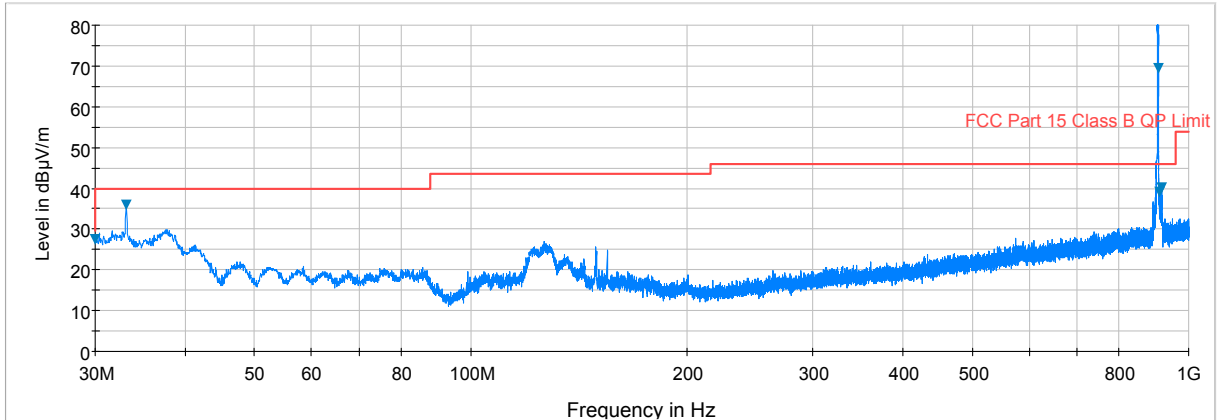
Plot 7-7. Radiated Spurious Plot below 1GHz (Zwave – 908.4MHz, Ant. Pol. H)
