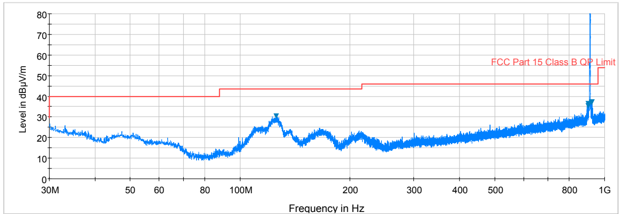
Plot 7-10. Radiated Spurious Plot below 1GHz (Zwave – 916MHz, Ant. Pol. H)
