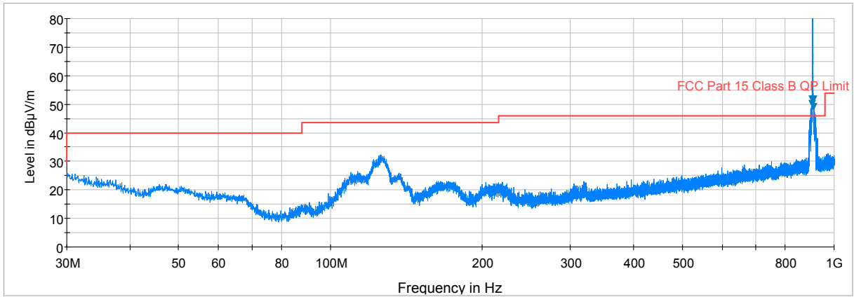
Plot 7-8. Radiated Spurious Plot below 1GHz (Zwave – 908.4MHz, Ant. Pol. H)
