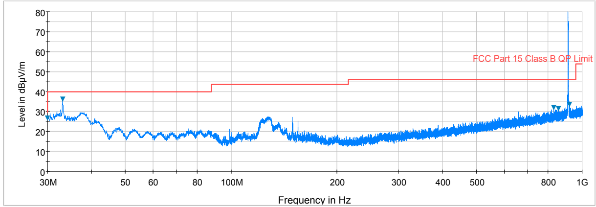
Plot 7-9. Radiated Spurious Plot below 1GHz (Zwave – 916MHz, Ant. Pol. H)
