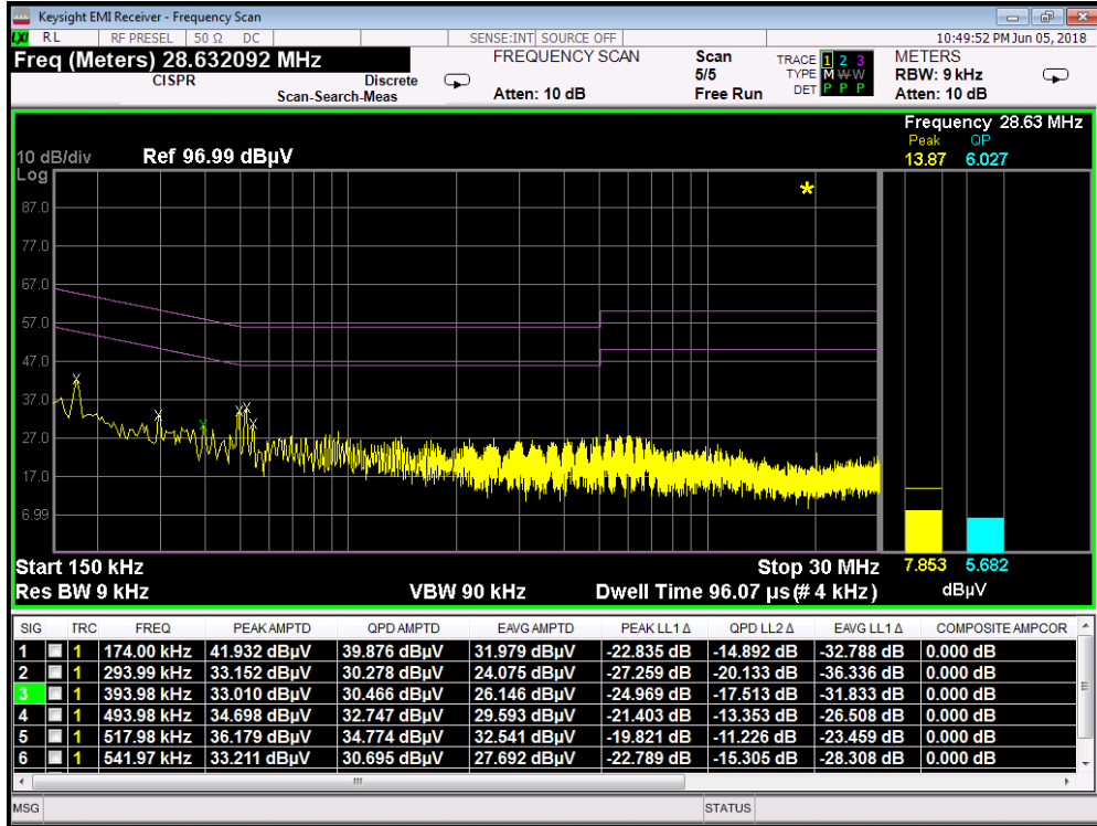
Plot 7-2. Line Conducted Plot (L1)
