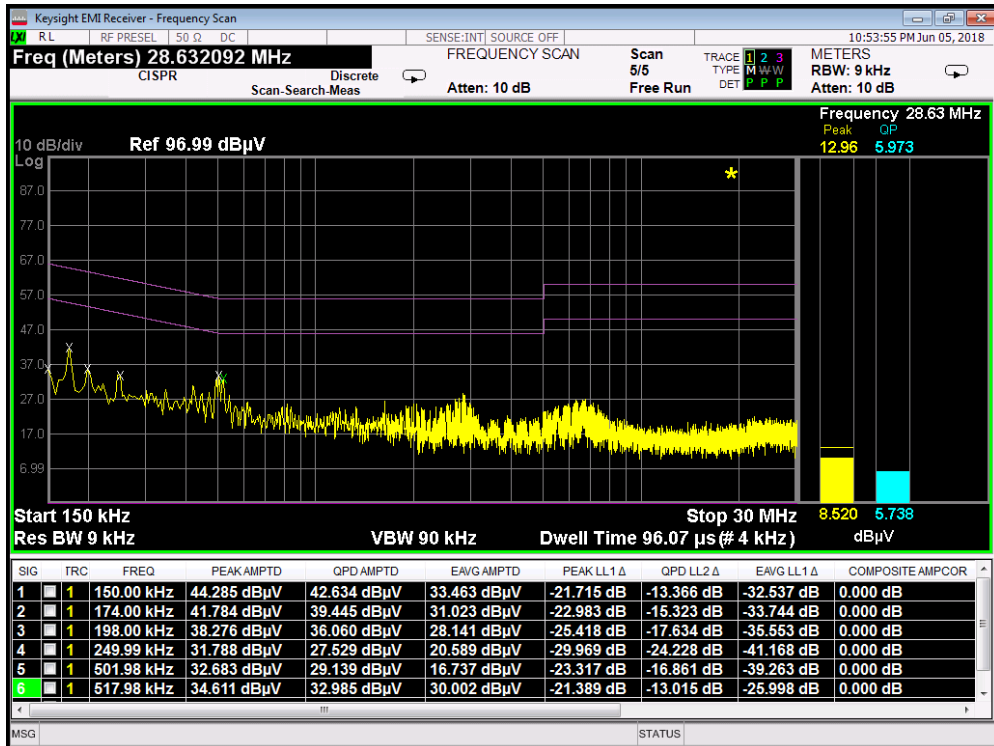
Plot 7-3. Line Conducted Plot (N)
