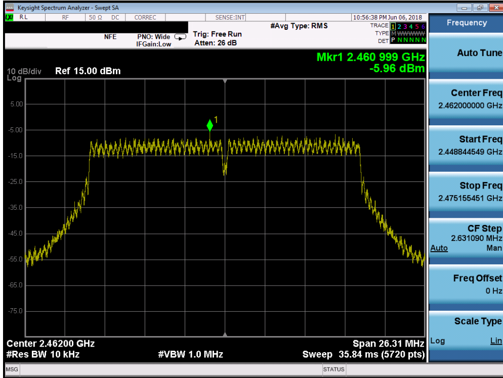
Plot 7-54. Power Spectral Density Plot SISO ANT2 (20MHz 802.11n (2.4GHz) – Ch. 11)
