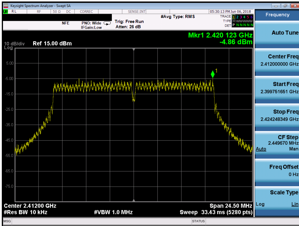
Plot 7-34. Power Spectral Density Plot SISO ANT1 (20MHz 802.11g – Ch. 1)
