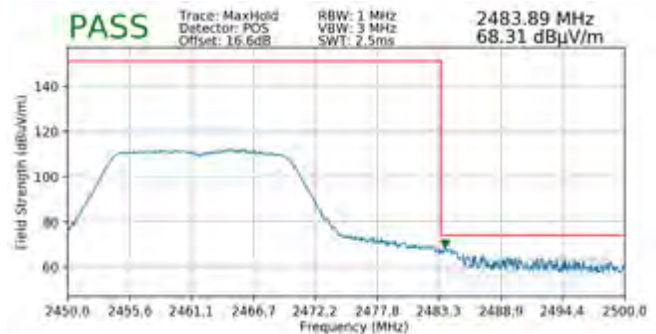
Plot 7-120. Radiated Restricted Upper Band Edge Measurement MIMO (Peak)
