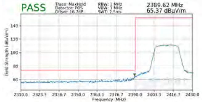
Plot 7-118. Radiated Restricted Lower Band Edge Measurement MIMO (Peak)
