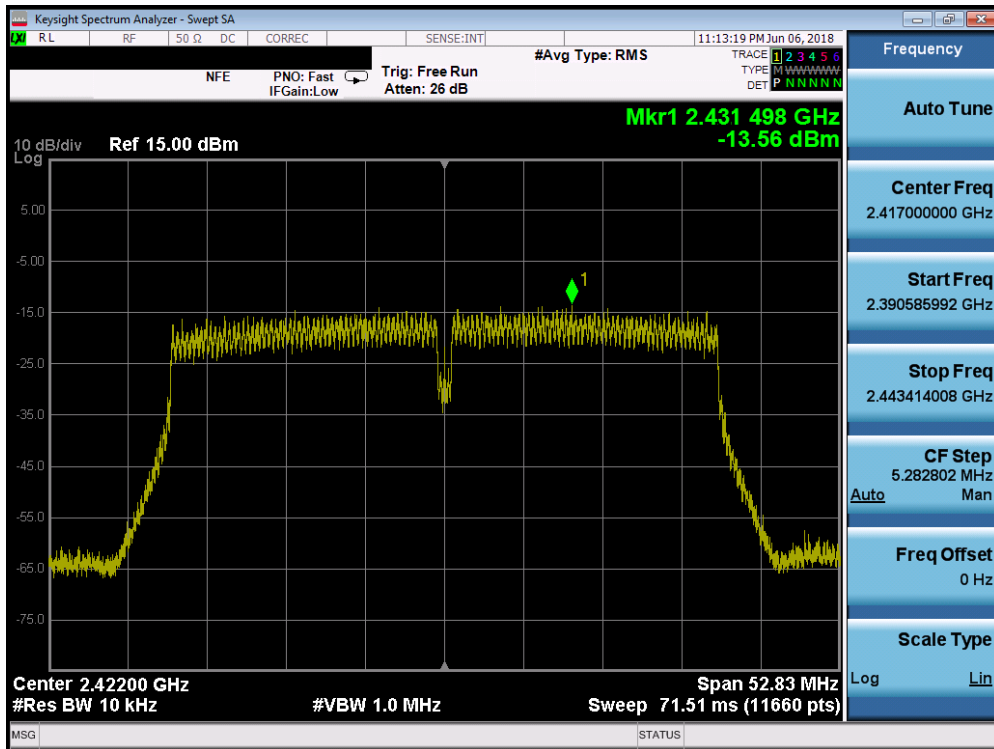
Plot 7-55. Power Spectral Density Plot SISO ANT2 (40MHz 802.11n (2.4GHz) – Ch. 3)
