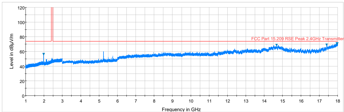
Plot 7-5. Radiated Pre-Scan Plot at 3-meters above 1 GHz (Ant. Pol. H)
