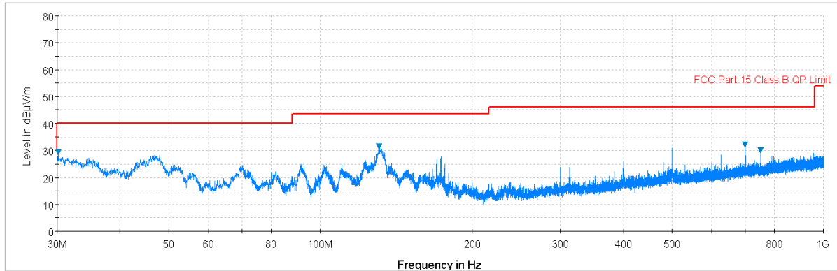
Plot 7-33. Radiated Spurious Plot below 1GHz (Pol. H)
