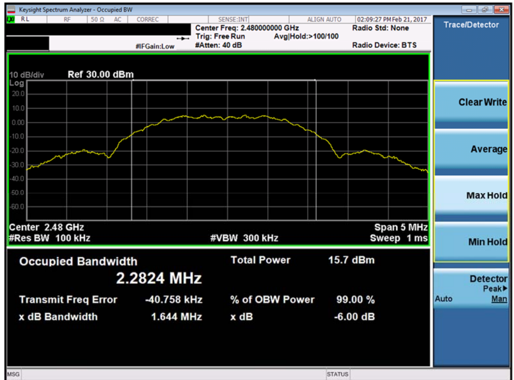
Plot 7-3. 6dB Bandwidth Plot (Zigbee – Ch. 26)
