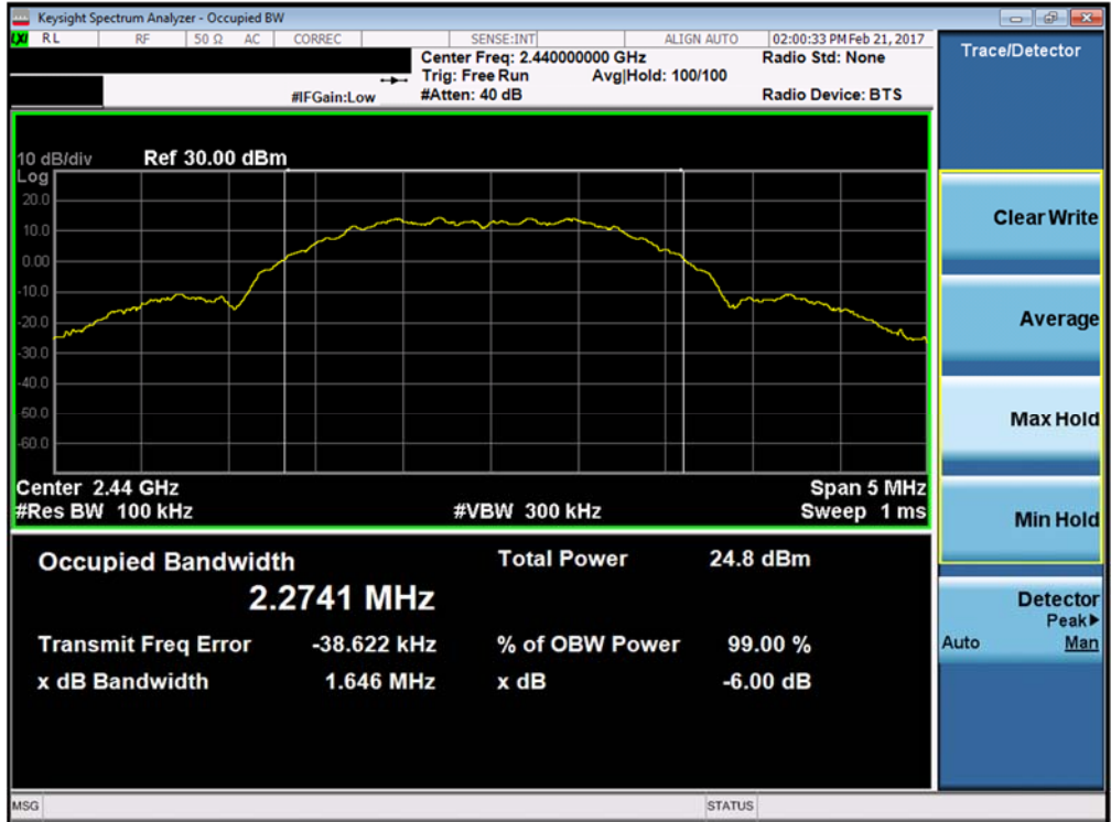
Plot 7-2. 6dB Bandwidth Plot (Zigbee – Ch. 18)
