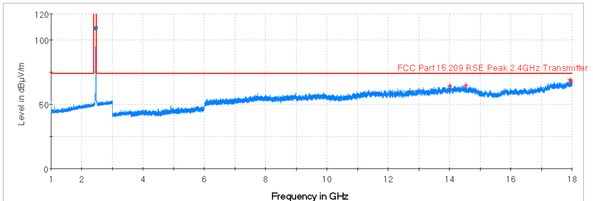
Plot 7-81. Radiated Spurious Plot above 1GHz (802.11b – Ch. 11, Ant. Pol. H)
