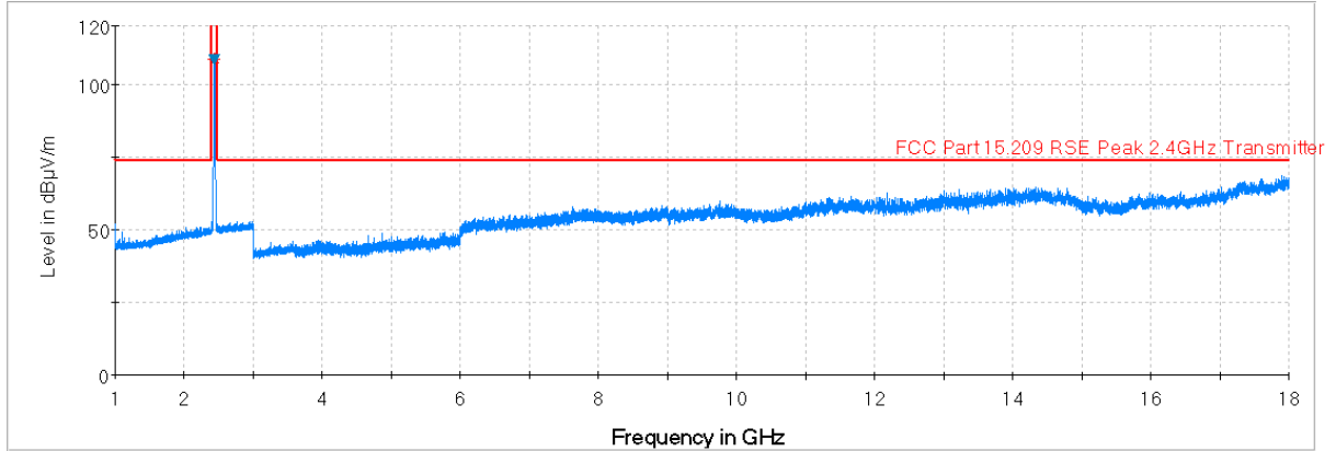
Plot 7-80. Radiated Spurious Plot above 1GHz (802.11b – Ch. 6, Ant. Pol. V)
