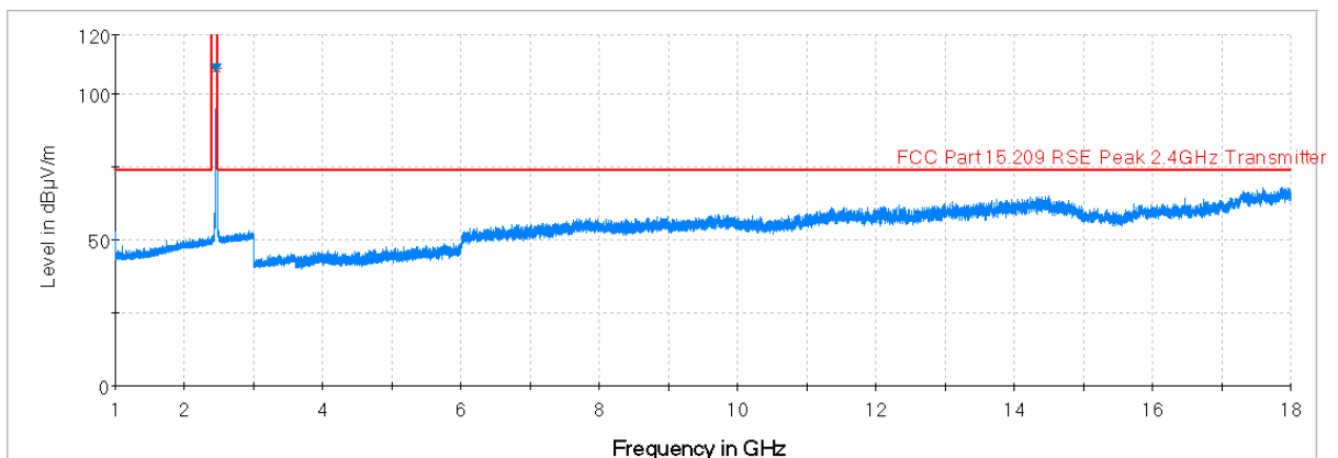
Plot 7-82. Radiated Spurious Plot above 1GHz (802.11b – Ch. 11, Ant. Pol. V)
