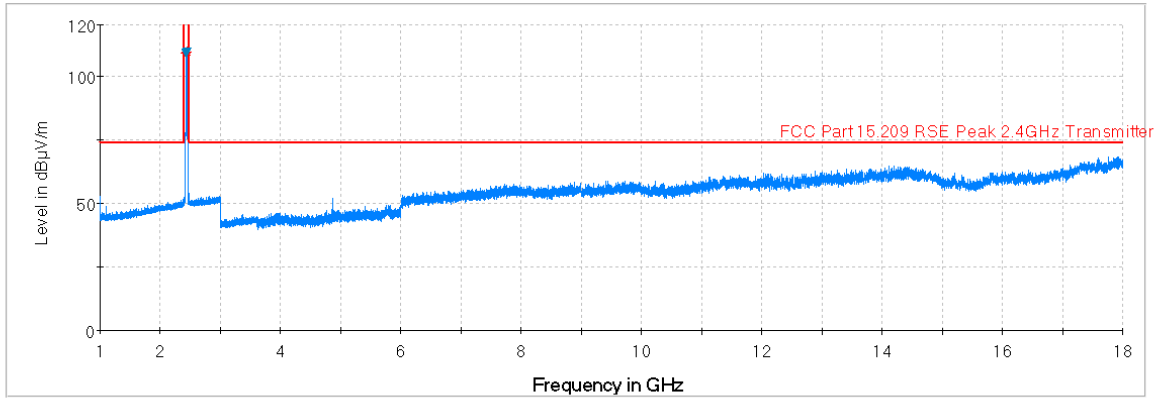
Plot 7-88. Radiated Spurious Plot above 1GHz (802.11b – Ch. 6, Ant. Pol. V)
