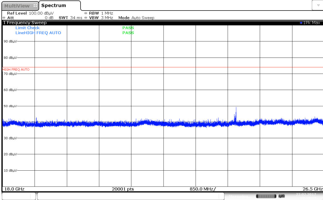
Plot 7-83. Radiated Spurious Plot above 18GHz (Pol. H)
