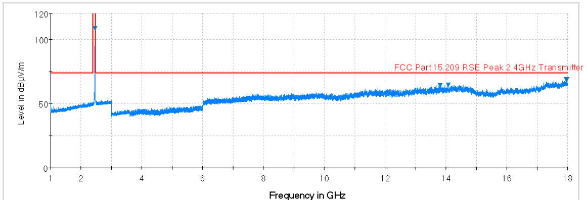
Plot 7-90. Radiated Spurious Plot above 1GHz (802.11b – Ch. 11, Ant. Pol. V)
