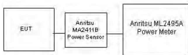
Figure 7-2. Test Instrument & Measurement Setup for Power Meter Measurements
