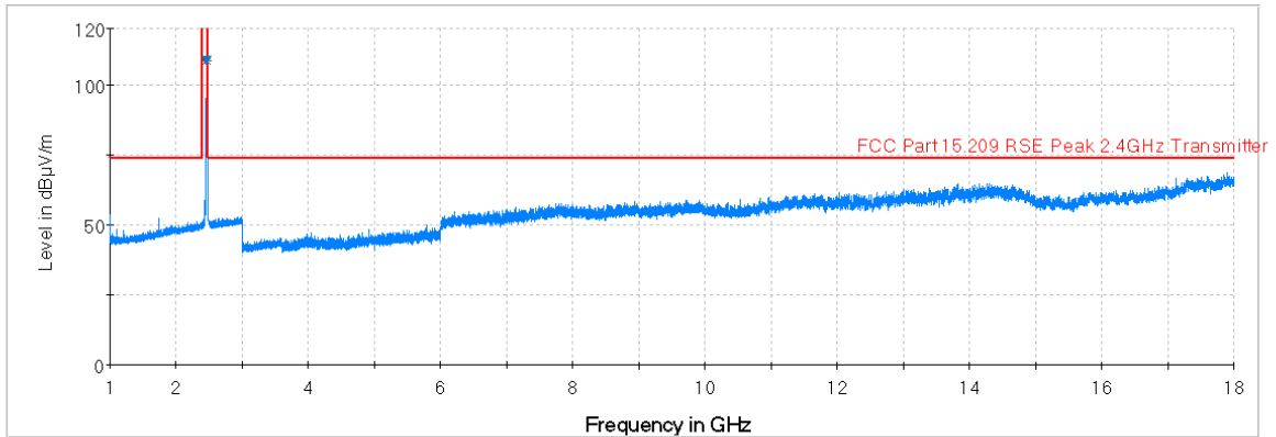
Plot 7-89. Radiated Spurious Plot above 1GHz (802.11b – Ch. 11, Ant. Pol. H)
