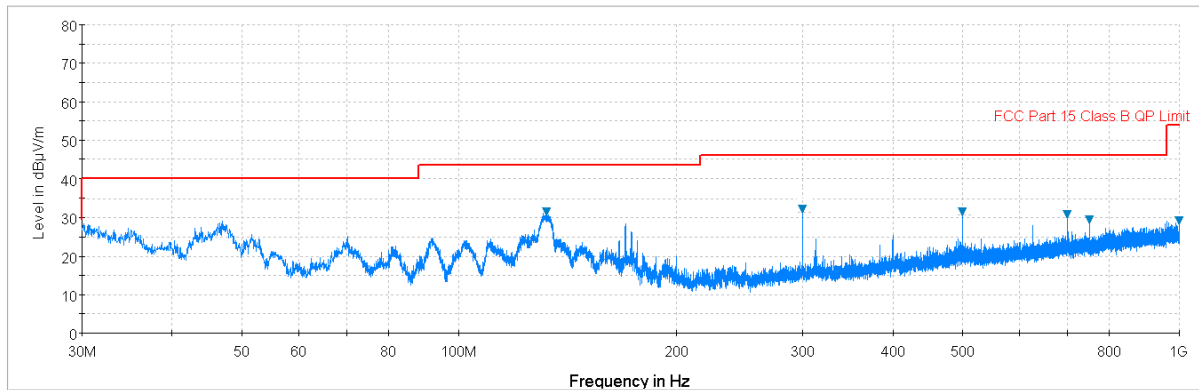
Plot 7-117. Radiated Spurious Plot below 1GHz (Pol. H)
