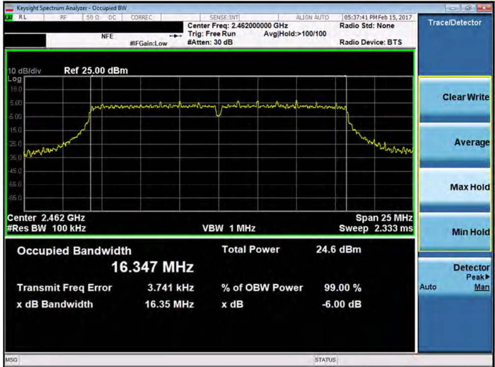
Plot 7-6. 6dB Bandwidth Plot (802.11g – Ch. 11)
