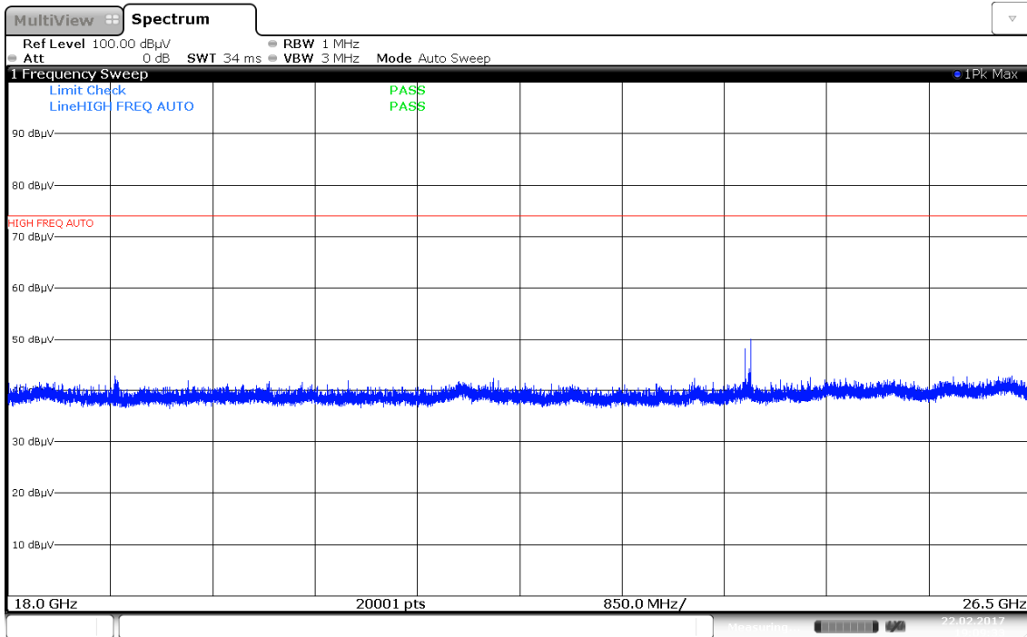
Plot 7-84. Radiated Spurious Plot above 18GHz (Pol. V)
