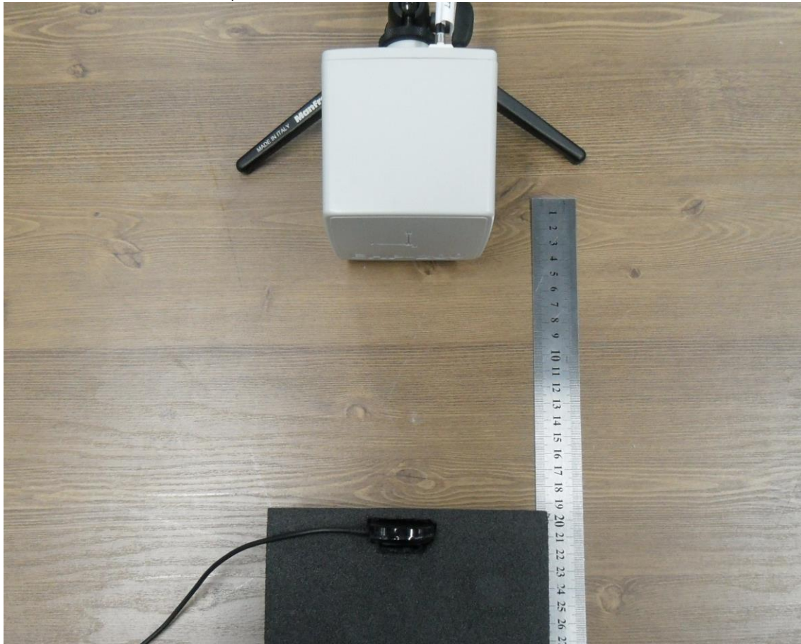
TOP, RF EXPOSURE SETUP PHOTO @20cm
