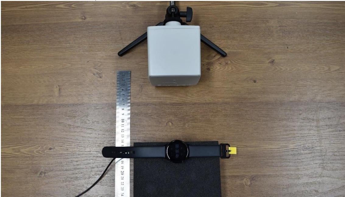
TOP, RF EXPOSURE SETUP PHOTO @20cm
