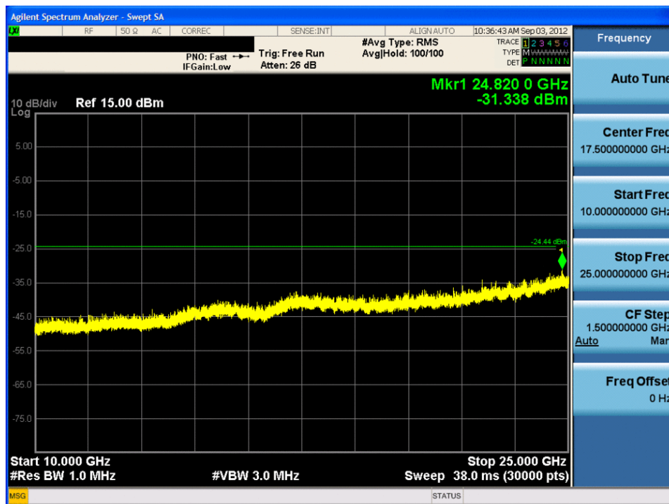
Plot 6-14. Conducted Spurious Plot (Bluetooth (LE) – Ch. 39)
