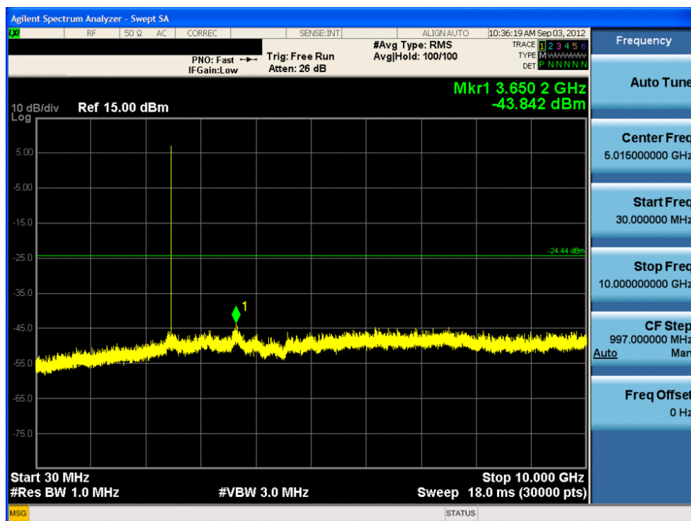
Plot 6-13. Conducted Spurious Plot (Bluetooth (LE) – Ch. 39)
