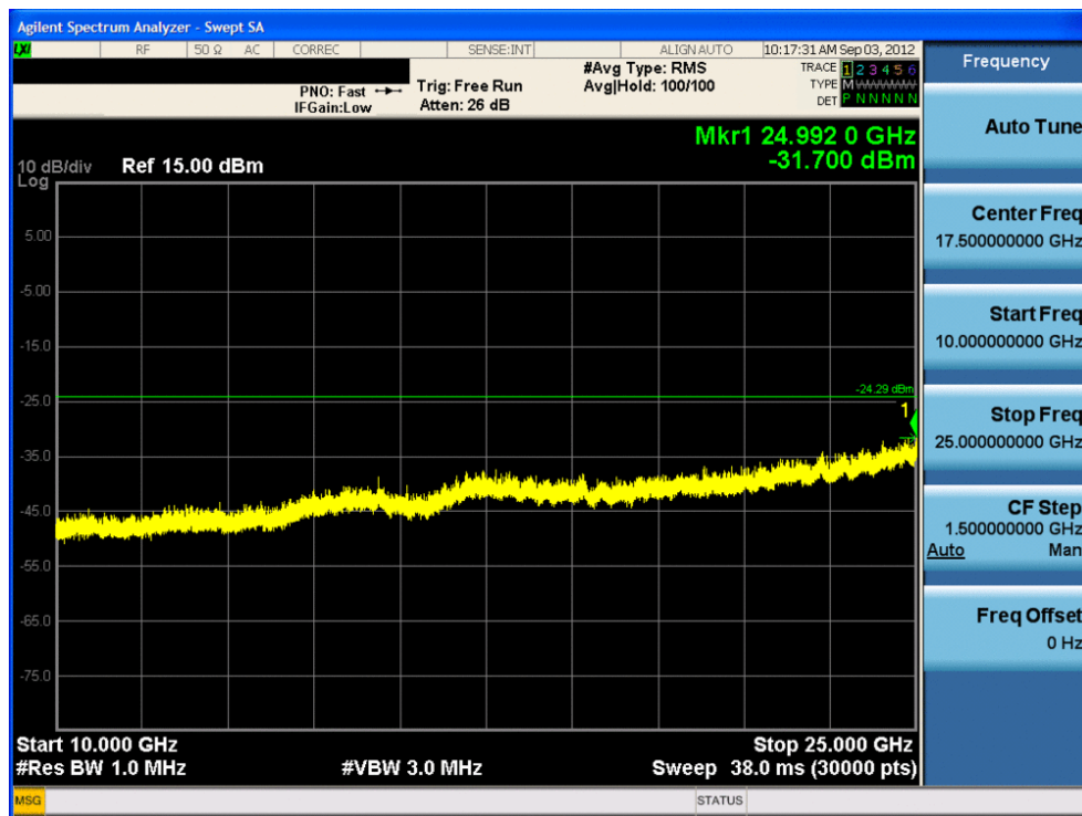
Plot 6-10. Conducted Spurious Plot (Bluetooth (LE) – Ch. 0)
