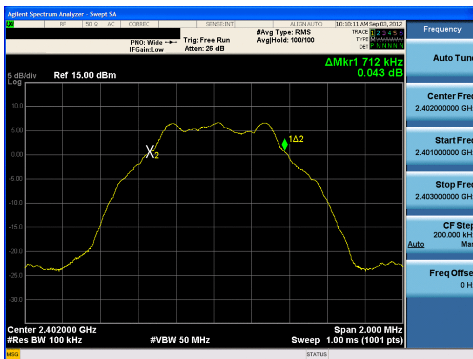
Plot 6-1. 6dB Bandwidth Plot (Bluetooth (LE) – Ch. 0)
