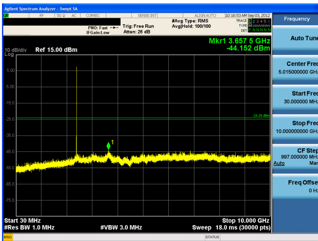
Plot 6-9. Conducted Spurious Plot (Bluetooth (LE) – Ch. 0)
