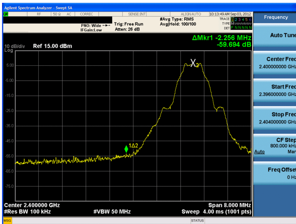
Plot 6-7. Band Edge Plot (Bluetooth (LE) – Ch. 0)
