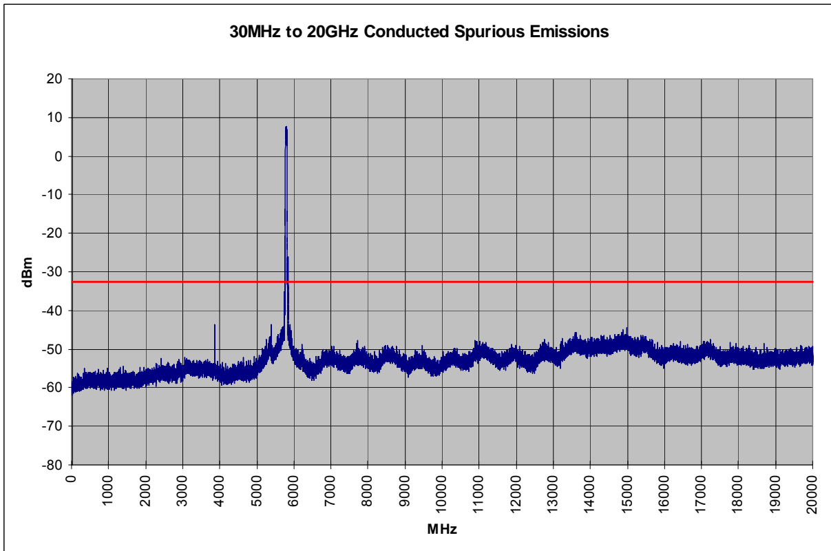
Plot 6-55. Conducted Spurious Plot (802.11a – Ch. 157)
