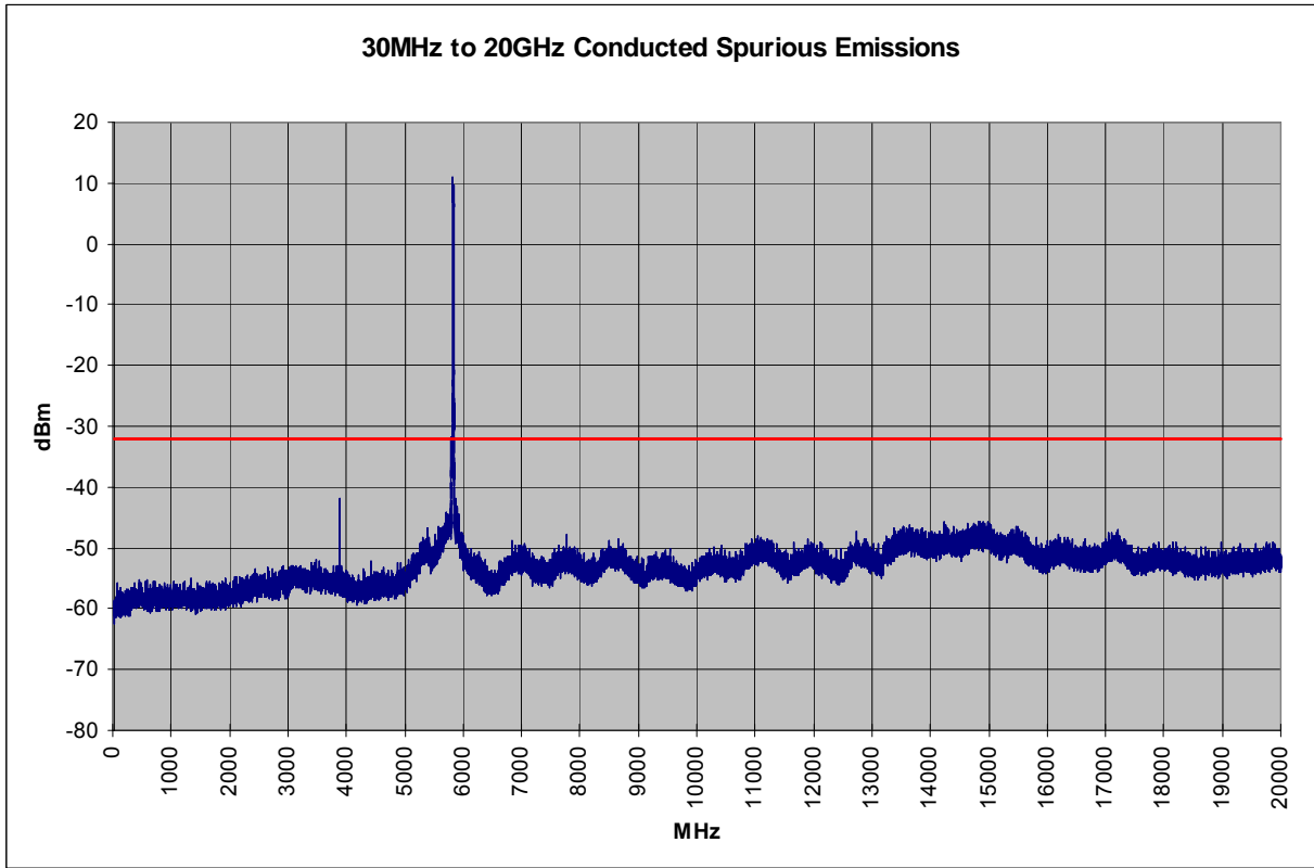
Plot 6-57. Conducted Spurious Plot (802.11a – Ch. 165)
