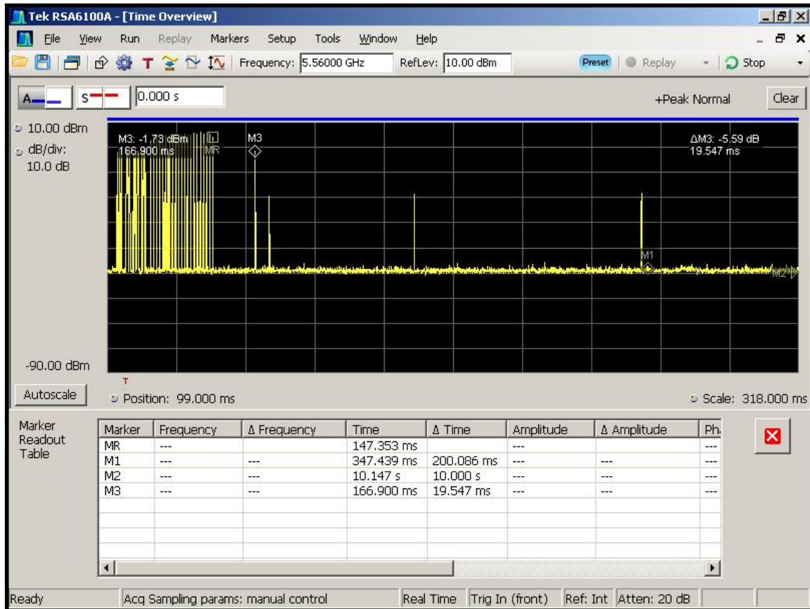
Figure 6-6. Client pulse detected before 200ms. This pulse is not included in aggregate time calculation.
