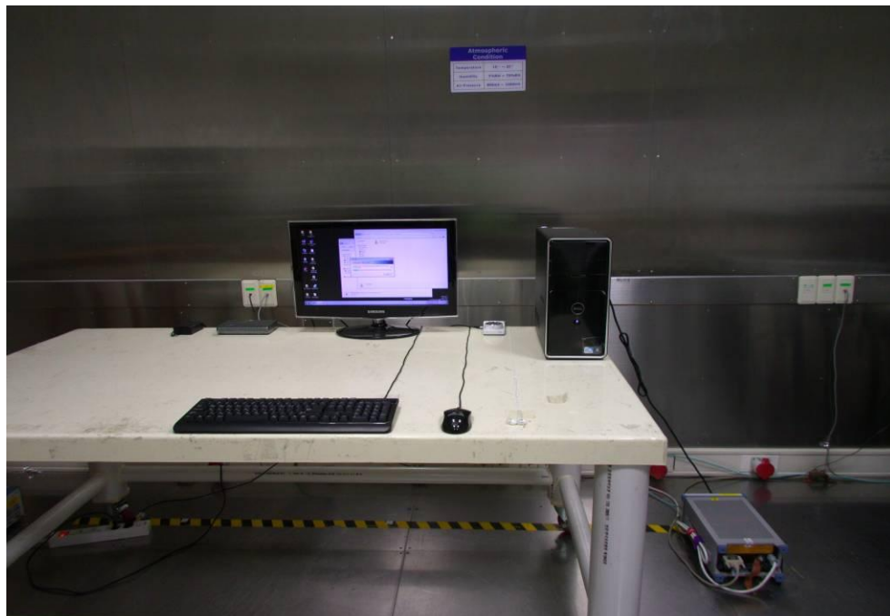
[ Conducted Disturbance – Front ]
