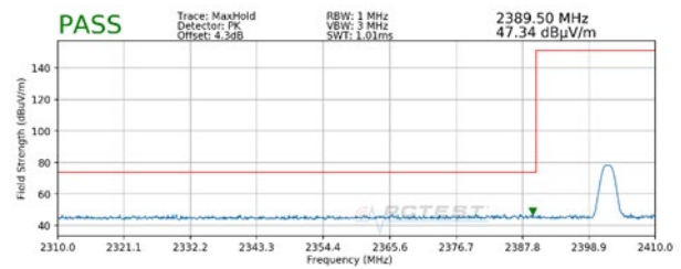
Plot 7-22. Radiated Restricted Lower Band Edge Measurement (Peak)
