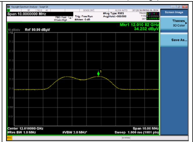
Low channel 5 th Harmonic (Average)
