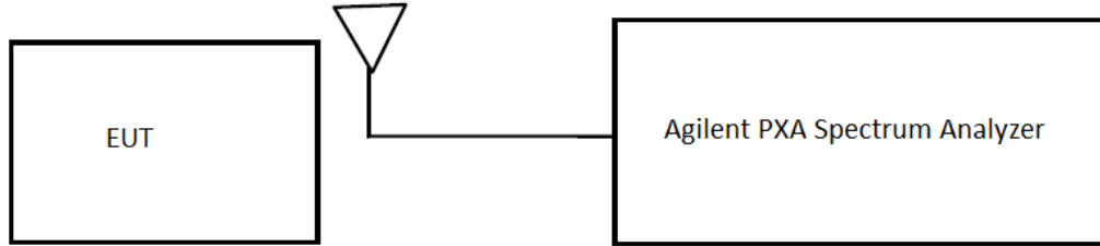
Figure 8-1. Test Instrument & Measurement Setup
