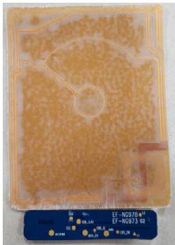
ANT Module(Front)
