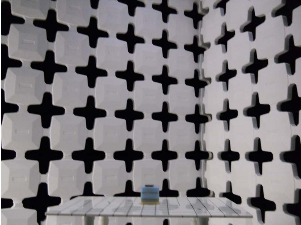
Figure 3 Radiated Test Setup
