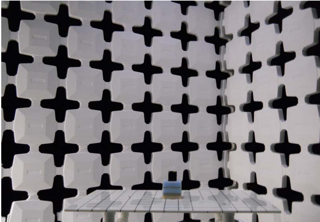
Figure 1 Radiated Test Setup
