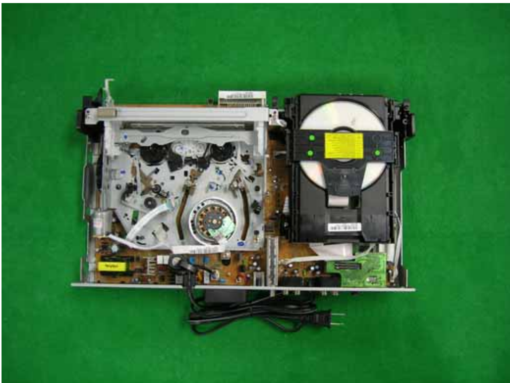
TOP VIEW (FRONT/TOP COVER OPENED)
