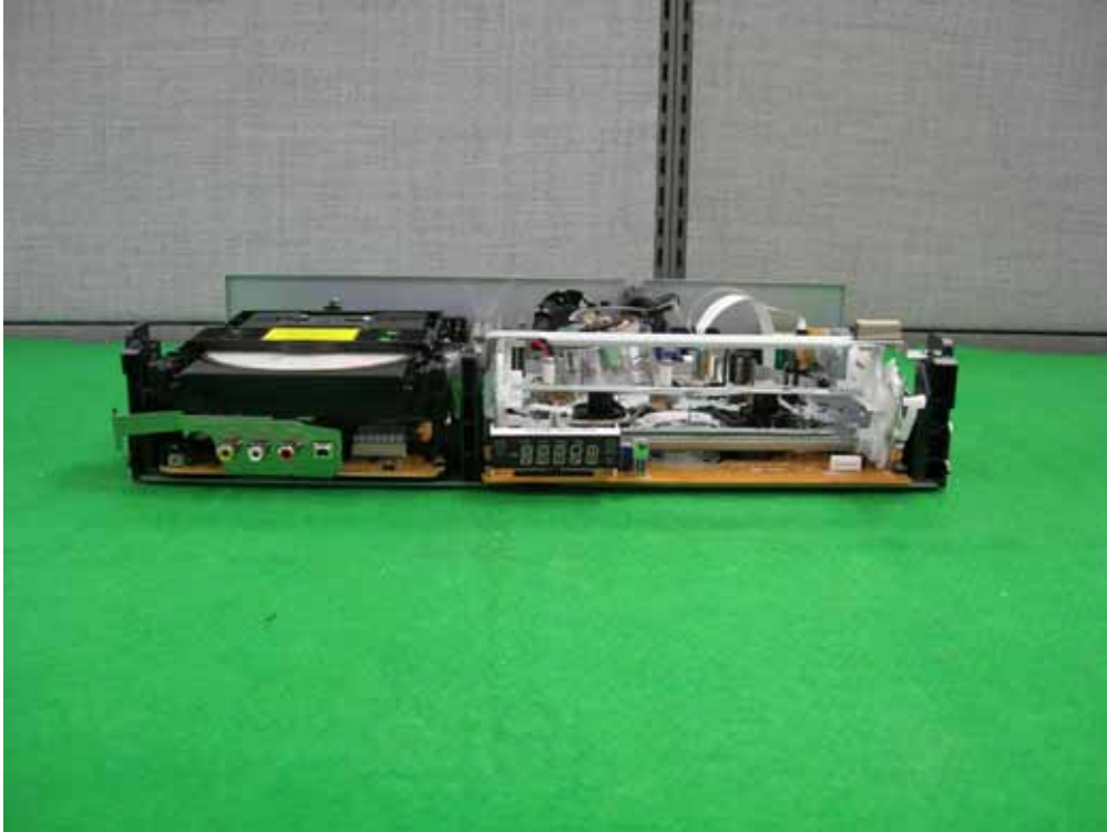
FRONT VIEW (FRONT/TOP COVER OPENED)
