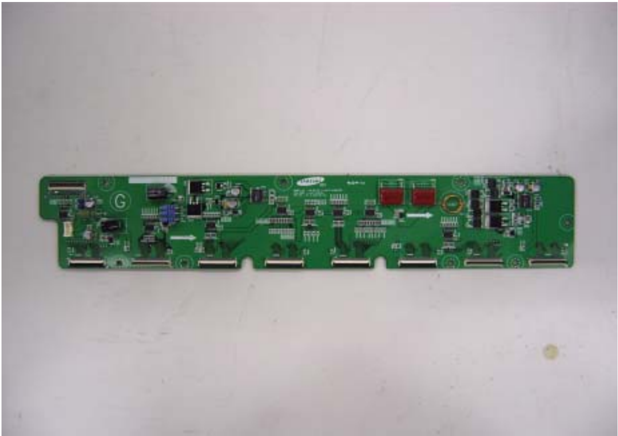
G buffer board top view
