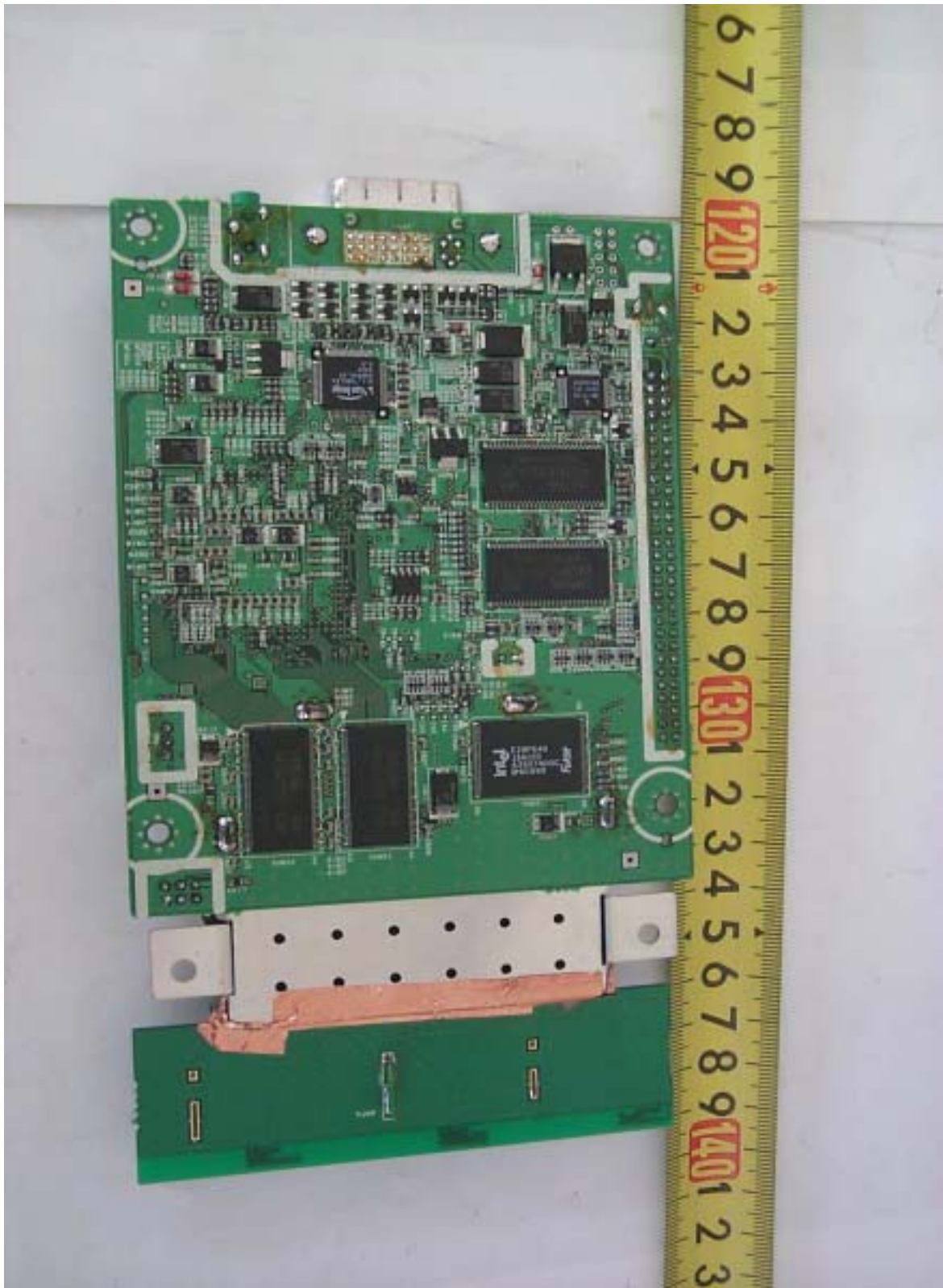
Main Board Bottom View (Wireless Module)
